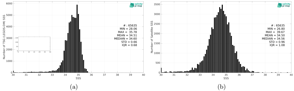
Figure 2: Histograms of SSS from TSG (LEGOS-DM) (a) and SMOS SSS L2Q v331 - 0.25 Deg (CATDS-CPDC) (b) considering all match-up pairs per bins of 0.1 over the North Pacific Ocean Pi-MEP region and for the full satellite product period.
