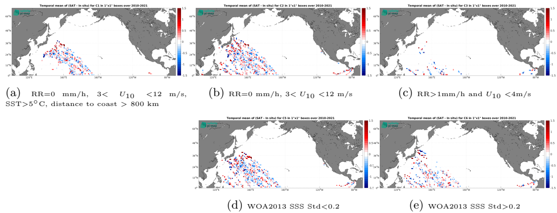
Figure 12: Temporal mean gridded over spatial boxes of size 1^\circ \times 1^\circ of \Delta\text{SSS} (SMOS SSS L2Q v331 - 0.25 Deg (CATDS-CPDC) - TSG (LEGOS-DM)) for 5 different subdatasets corresponding to:RR=0 mm/h, 3 < U_{10} < 12 m/s, SST >5^\circ\text{C} , distance to coast > 800 km (a), RR=0 mm/h, 3 < U_{10} < 12 m/s (b), RR >1 mm/h and U_{10} < 4 m/s (c), WOA2013 SSS Std <0.2 (d), WOA2013 SSS Std >0.2 (e).
