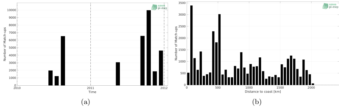
Figure 1: Number of match-ups between TSG (GOSUD-Sailing-ship) and SMOS SSS L2Q v331 - 0.25 Deg (CATDS-CPDC) SSS as a function of time (a) and as function of the distance to coast (b) over the North Pacific Ocean Pi-MEP region and for the full satellite product period.
