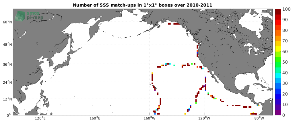
Figure 4: Number of SSS match-ups between TSG (GOSUD-Sailing-ship) SSS and the SMOS SSS L2Q v331 - 0.25 Deg (CATDS-CPDC) SSS product for the North Pacific Ocean Pi-MEP region over 1^\circ \times 1^\circ boxes and for the full satellite product period.
