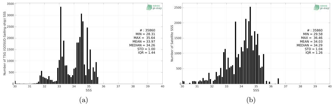
Figure 2: Histograms of SSS from TSG (GOSUD-Sailing-ship) (a) and SMOS SSS L2Q v331 - 0.25 Deg (CATDS-CPDC) (b) considering all match-up pairs per bins of 0.1 over the North Pacific Ocean Pi-MEP region and for the full satellite product period.
