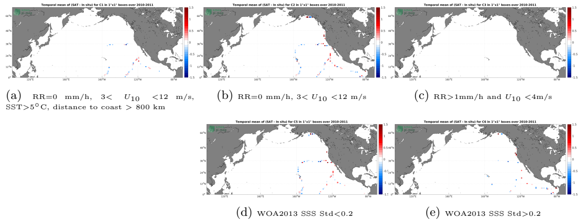
Figure 12: Temporal mean gridded over spatial boxes of size 1^\circ \times 1^\circ of \Delta SSS (SMOS SSS L2Q v331 - 0.25 Deg (CATDS-CPDC) - TSG (GOSUD-Sailing-ship)) for 5 different subdatasets corresponding to:RR=0 mm/h, 3 < U_{10} < 12 m/s, SST >5^\circ\text{C} , distance to coast > 800 km (a), RR=0 mm/h, 3 < U_{10} < 12 m/s (b), RR >1 mm/h and U_{10} < 4 m/s (c), WOA2013 SSS Std <0.2 (d), WOA2013 SSS Std >0.2 (e).
