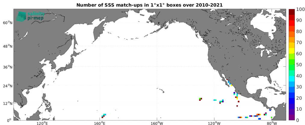
Figure 4: Number of SSS match-ups between TSG (GOSUD-Research-vessel) SSS and the SMOS SSS L2Q v331 - 0.25 Deg (CATDS-CPDC) SSS product for the North Pacific Ocean Pi-MEP region over 1^\circ \times 1^\circ boxes and for the full satellite product period.
