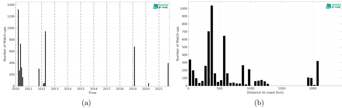
Figure 1: Number of match-ups between TSG (GOSUD-Research-vessel) and SMOS SSS L2Q v331 - 0.25 Deg (CATDS-CPDC) SSS as a function of time (a) and as function of the distance to coast (b) over the North Pacific Ocean Pi-MEP region and for the full satellite product period.
