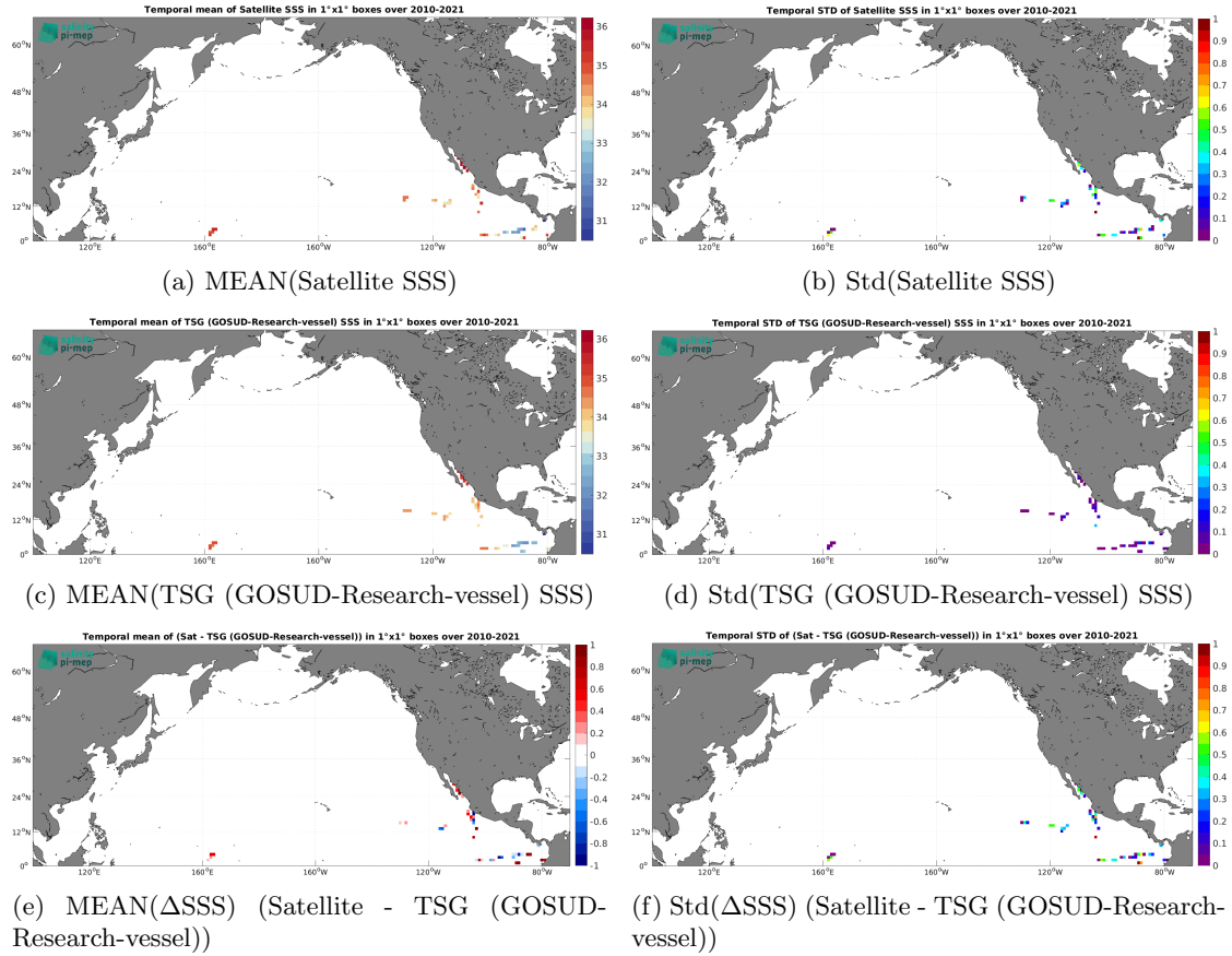
Figure 6: Temporal mean (left) and Std (right) of SSS from SMOS SSS L2Q v331 - 0.25 Deg (CATDS-CPDC) (top), TSG (GOSUD-Research-vessel) (middle), and of \Delta SSS (Satellite - TSG (GOSUD-Research-vessel)). Only match-up pairs are used to generate these maps.
