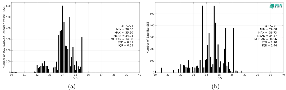
Figure 2: Histograms of SSS from TSG (GOSUD-Research-vessel) (a) and SMOS SSS L2Q v331 - 0.25 Deg (CATDS-CPDC) (b) considering all match-up pairs per bins of 0.1 over the North Pacific Ocean Pi-MEP region and for the full satellite product period.
