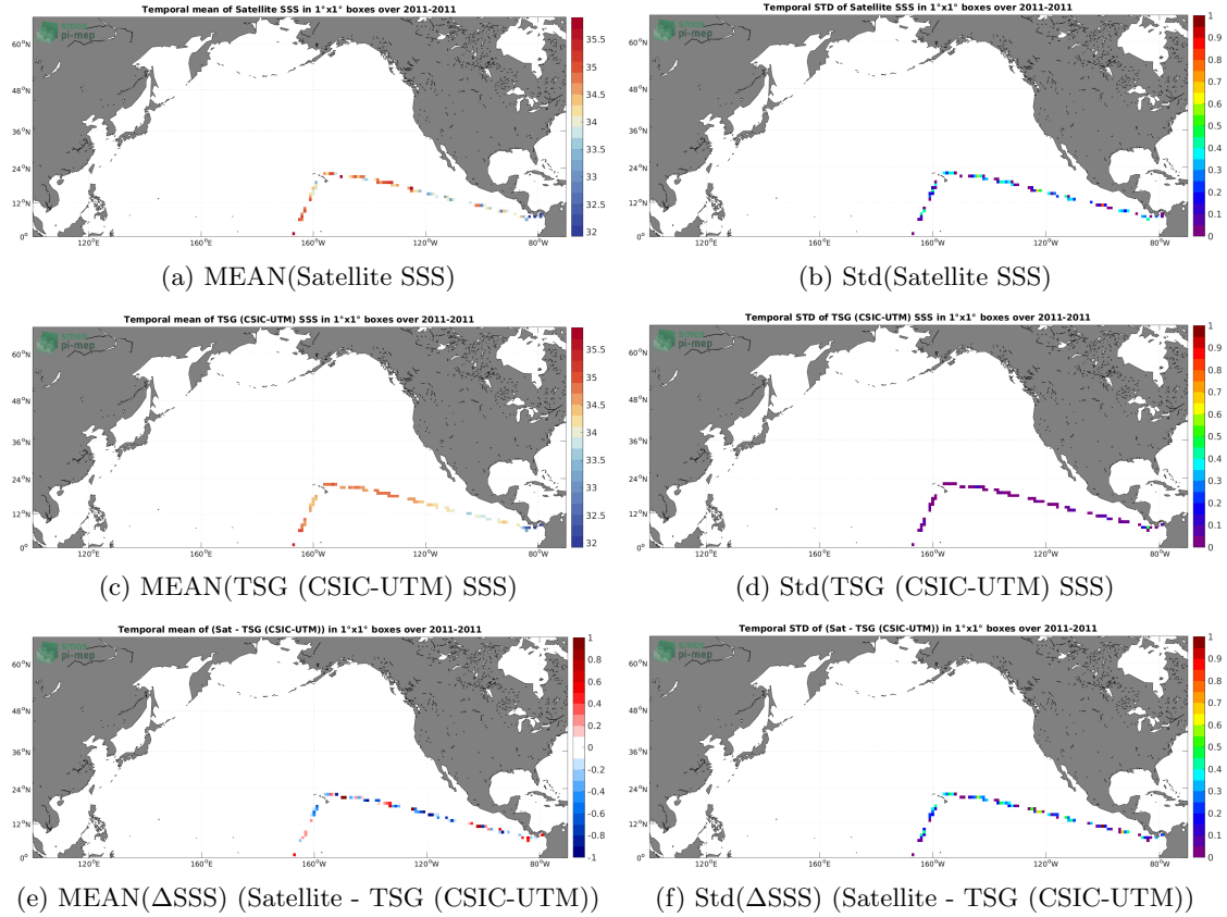
Figure 6: Temporal mean (left) and Std (right) of SSS from SMOS SSS L2Q v331 - 0.25 Deg (CATDS-CPDC) (top), TSG (CSIC-UTM) (middle), and of \Delta SSS (Satellite - TSG (CSIC-UTM)). Only match-up pairs are used to generate these maps.
