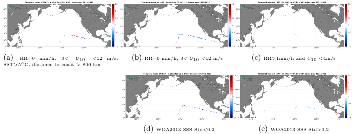
Figure 12: Temporal mean gridded over spatial boxes of size 1^{\circ}\times 1^{\circ} of \Delta\text{SSS} (SMOS SSS L2Q v331 - 0.25 Deg (CATDS-CPDC) - TSG (CSIC-UTM)) for 5 different subdatasets corresponding to:RR=0 mm/h, 3 < U_{10} < 12 m/s, SST >5^{\circ}\text{C} , distance to coast > 800 km (a), RR=0 mm/h, 3 < U_{10} < 12 m/s (b), RR >1 mm/h and U_{10} < 4 m/s (c), WOA2013 SSS Std <0.2 (d), WOA2013 SSS Std >0.2 (e).
