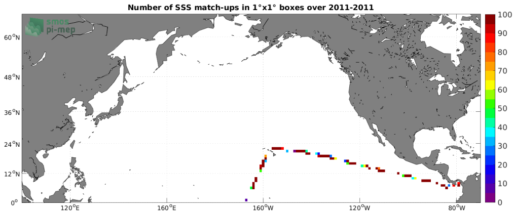
Figure 4: Number of SSS match-ups between TSG (CSIC-UTM) SSS and the SMOS SSS L2Q v331 - 0.25 Deg (CATDS-CPDC) SSS product for the North Pacific Ocean Pi-MEP region over 1^\circ \times 1^\circ boxes and for the full satellite product period.
