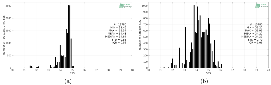
Figure 2: Histograms of SSS from TSG (CSIC-UTM) (a) and SMOS SSS L2Q v331 - 0.25 Deg (CATDS-CPDC) (b) considering all match-up pairs per bins of 0.1 over the North Pacific Ocean Pi-MEP region and for the full satellite product period.
