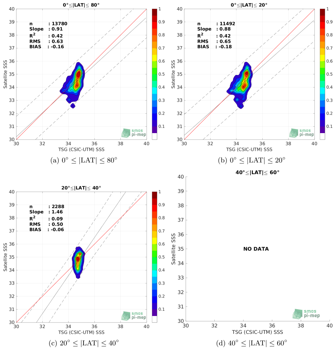
Figure 9: Contour maps of the concentration of SMOS SSS L2Q v331 - 0.25 Deg (CATDS-CPDC) SSS (y-axis) versus TSG (CSIC-UTM) SSS (x-axis) at match-up pairs for different latitude bands. For each plot, the red line shows x=y . The black thin and dashed lines indicate a linear fit through the data cloud and the \pm 95\% confidence levels, respectively. The number match-up pairs n , the slope and R^2 coefficient of the linear fit, the root mean square (RMS) and the mean bias between satellite and in situ data are indicated for each latitude band in each plots.
