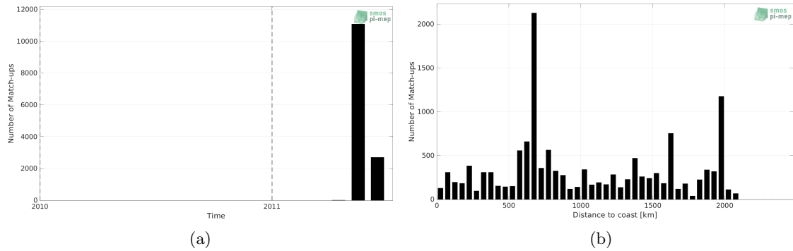
Figure 1: Number of match-ups between TSG (CSIC-UTM) and SMOS SSS L2Q v331 - 0.25 Deg (CATDS-CPDC) SSS as a function of time (a) and as function of the distance to coast (b) over the North Pacific Ocean Pi-MEP region and for the full satellite product period.
