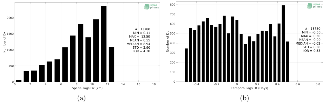
Figure 5: Histograms of the spatial (a) and temporal (b) lags between the location/time of the TSG (CSIC-UTM) measurement and the date of the corresponding SMOS SSS L2Q v331 - 0.25 Deg (CATDS-CPDC) SSS pixel.
