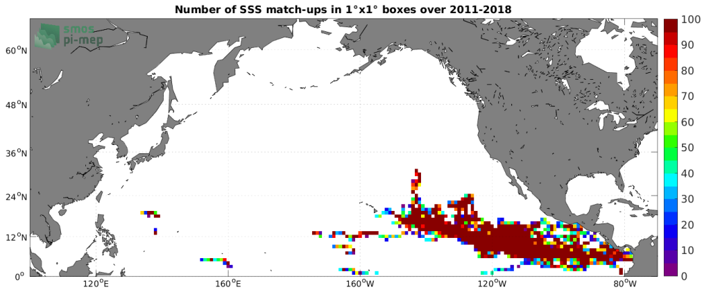
Figure 3: Number of SSS match-ups between Surface drifters SSS and the SMOS SSS L2Q v331 - 0.25 Deg (CATDS-CPDC) SSS product for the North Pacific Ocean Pi-MEP region over 1^\circ \times 1^\circ boxes and for the full satellite product period.
