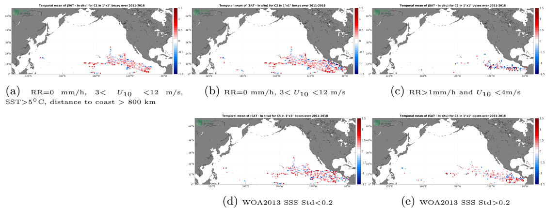
Figure 11: Temporal mean gridded over spatial boxes of size 1^\circ \times 1^\circ of \Delta SSS (SMOS SSS L2Q v331 - 0.25 Deg (CATDS-CPDC) - Surface drifters) for 5 different subdatasets corresponding to: RR=0 mm/h, 3 < U_{10} < 12 m/s, SST >5^\circ C, distance to coast > 800 km (a), RR=0 mm/h, 3 < U_{10} < 12 m/s (b), RR >1 mm/h and U_{10} < 4 m/s (c), WOA2013 SSS Std <0.2 (d), WOA2013 SSS Std >0.2 (e).
