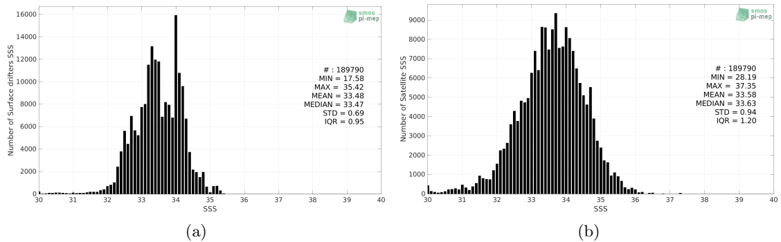
Figure 2: Histograms of SSS from Surface drifters (a) and SMOS SSS L2Q v331 - 0.25 Deg (CATDS-CPDC) (b) considering all match-up pairs per bins of 0.1 over the North Pacific Ocean Pi-MEP region and for the full satellite product period.
