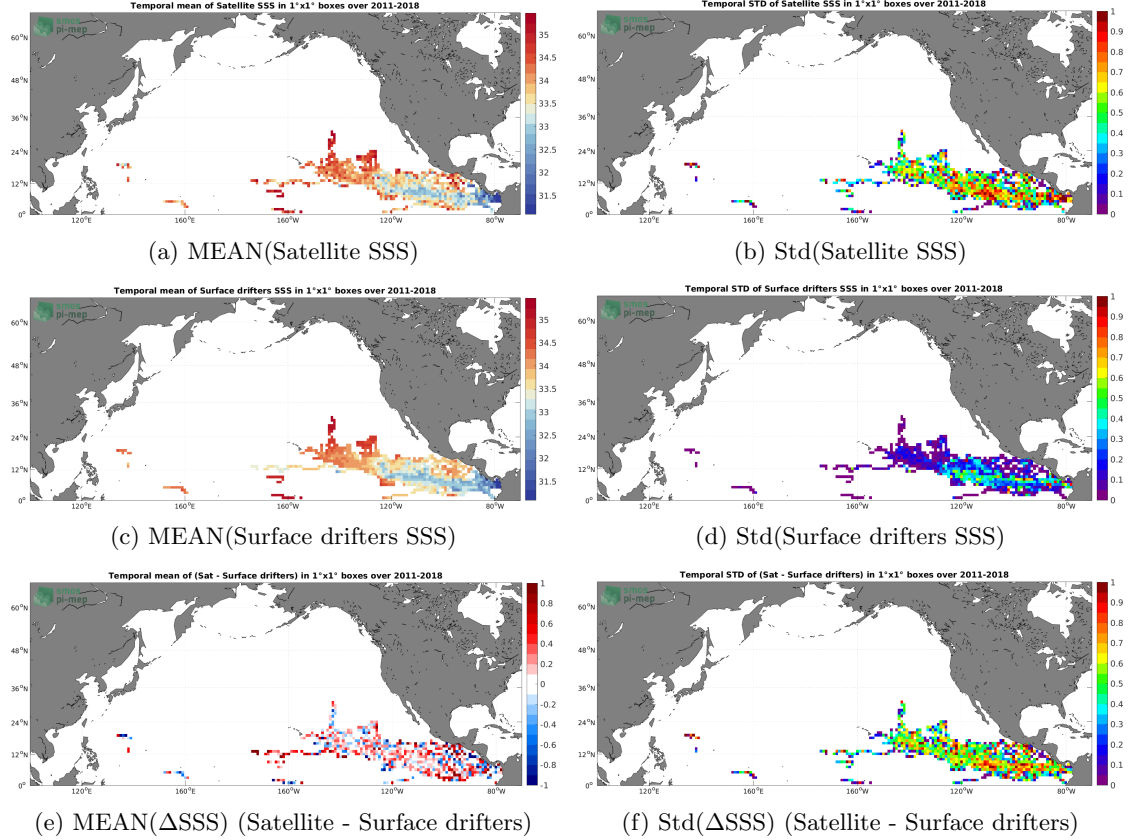
Figure 5: Temporal mean (left) and Std (right) of SSS from SMOS SSS L2Q v331 - 0.25 Deg (CATDS-CPDC) (top), Surface drifters (middle), and of \Delta SSS (Satellite - Surface drifters). Only match-up pairs are used to generate these maps.
