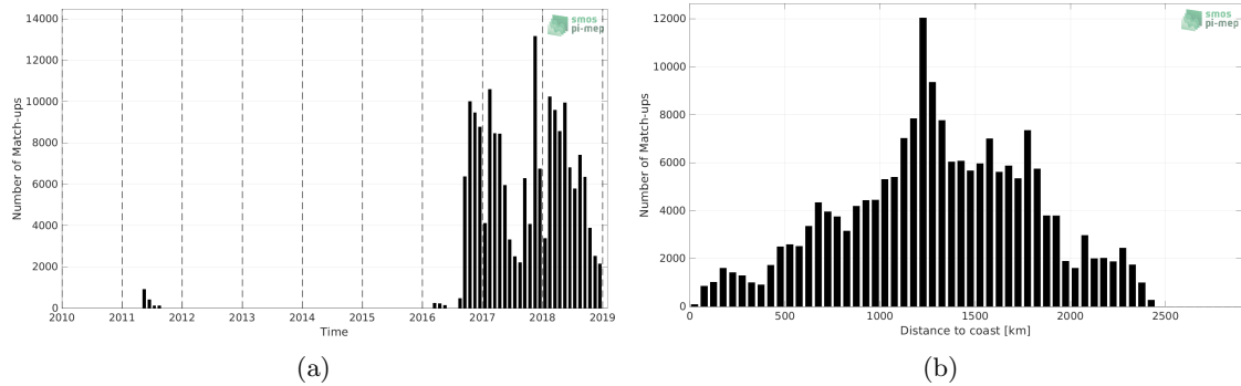
Figure 1: Number of match-ups between Surface drifters and SMOS SSS L2Q v331 - 0.25 Deg (CATDS-CPDC) SSS as a function of time (a) and as function of the distance to coast (b) over the North Pacific Ocean Pi-MEP region and for the full satellite product period.
