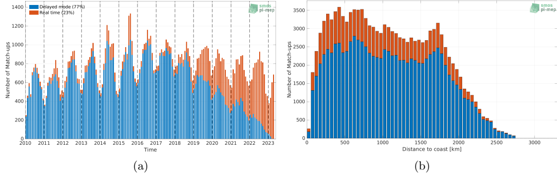
Figure 1: Number of match-ups between Argo and SMOS SSS L2Q v331 - 0.25 Deg (CATDS-CPDC) SSS as a function of time (a) and as function of the distance to coast (b) over the North Pacific Ocean Pi-MEP region and for the full satellite product period.
