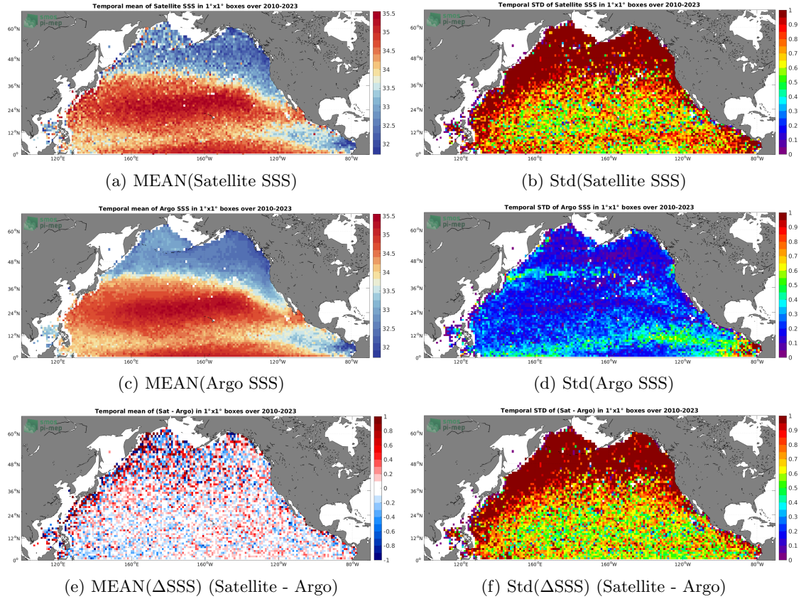
Figure 6: Temporal mean (left) and Std (right) of SSS from SMOS SSS L2Q v331 - 0.25 Deg (CATDS-CPDC) (top), Argo (middle), and of \Delta SSS (Satellite - Argo). Only match-up pairs are used to generate these maps.
