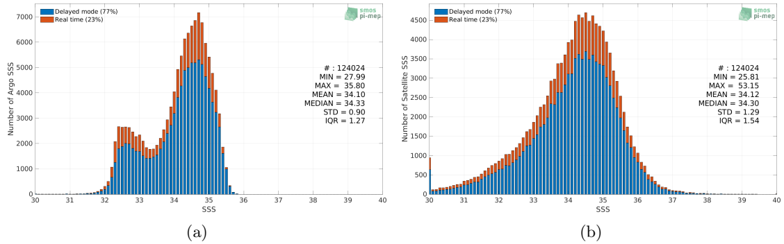
Figure 2: Histograms of SSS from Argo (a) and SMOS SSS L2Q v331 - 0.25 Deg (CATDS-CPDC) (b) considering all match-up pairs per bins of 0.1 over the North Pacific Ocean Pi-MEP region and for the full satellite product period.
