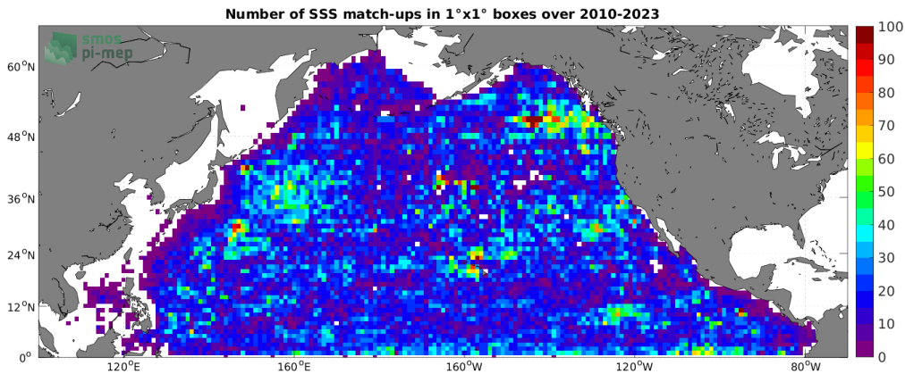
Figure 4: Number of SSS match-ups between Argo SSS and the SMOS SSS L2Q v331 - 0.25 Deg (CATDS-CPDC) SSS product for the North Pacific Ocean Pi-MEP region over 1^\circ \times 1^\circ boxes and for the full satellite product period.
