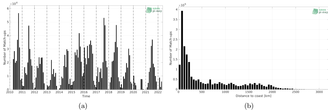
Figure 1: Number of match-ups between TSG (SAMOS) and SMOS SSS L2Q v330 - 0.25 Deg (CATDS-CPDC) SSS as a function of time (a) and as function of the distance to coast (b) over the North Pacific Ocean Pi-MEP region and for the full satellite product period.
