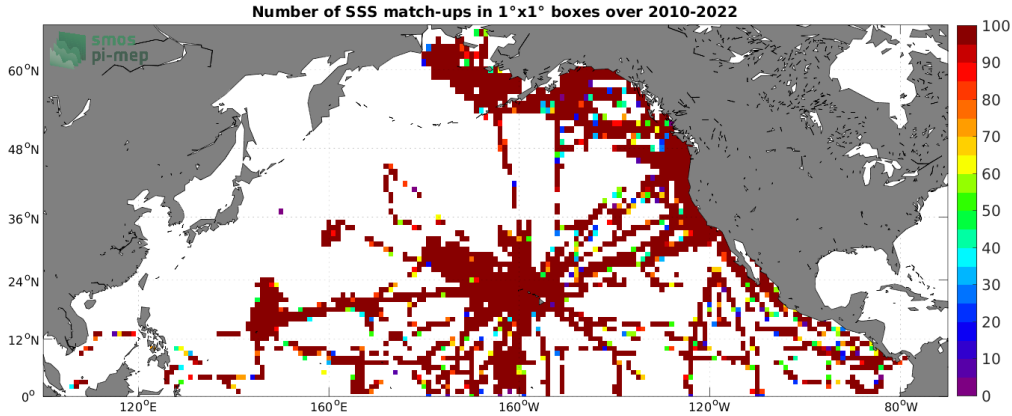
Figure 4: Number of SSS match-ups between TSG (SAMOS) SSS and the SMOS SSS L2Q v330 - 0.25 Deg (CATDS-CPDC) SSS product for the North Pacific Ocean Pi-MEP region over 1^\circ \times 1^\circ boxes and for the full satellite product period.
