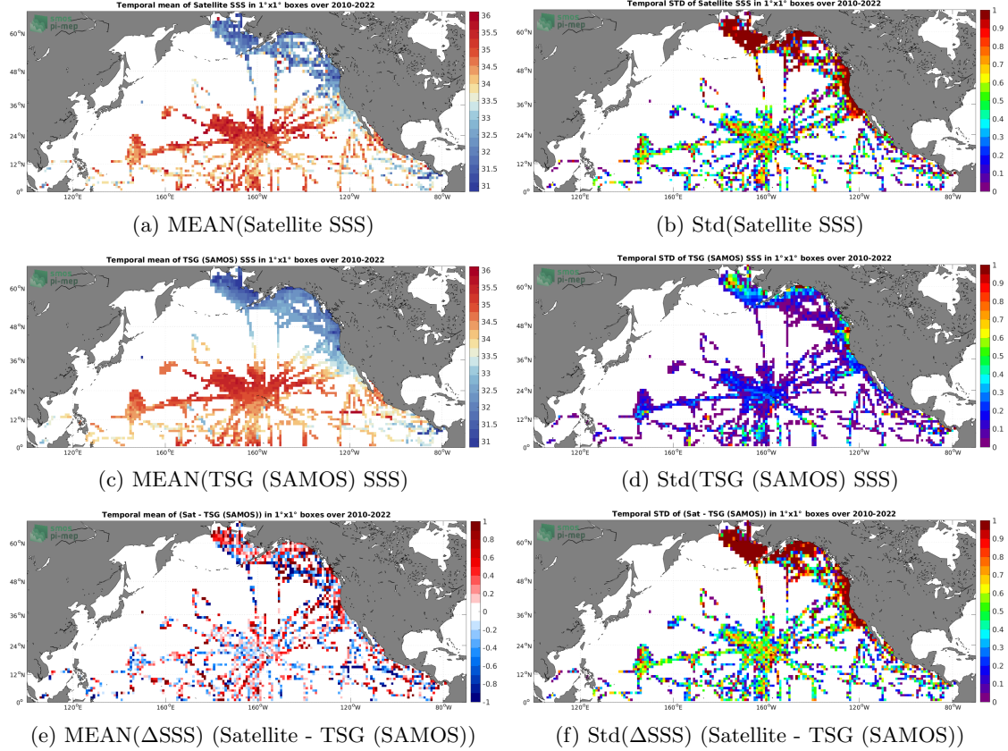
Figure 6: Temporal mean (left) and Std (right) of SSS from SMOS SSS L2Q v330 - 0.25 Deg (CATDS-CPDC) (top), TSG (SAMOS) (middle), and of \Delta SSS (Satellite - TSG (SAMOS)). Only match-up pairs are used to generate these maps.
