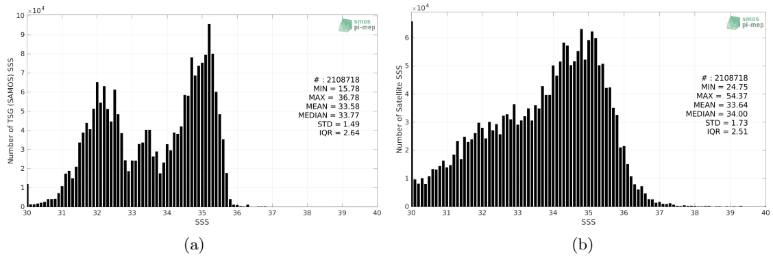
Figure 2: Histograms of SSS from TSG (SAMOS) (a) and SMOS SSS L2Q v330 - 0.25 Deg (CATDS-CPDC) (b) considering all match-up pairs per bins of 0.1 over the North Pacific Ocean Pi-MEP region and for the full satellite product period.
