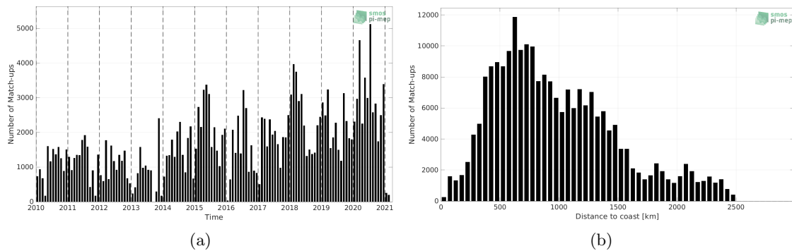
Figure 1: Number of match-ups between TSG (LEGOS-DM) and SMOS SSS L2Q v330 - 0.25 Deg (CATDS-CPDC) SSS as a function of time (a) and as function of the distance to coast (b) over the North Pacific Ocean Pi-MEP region and for the full satellite product period.
