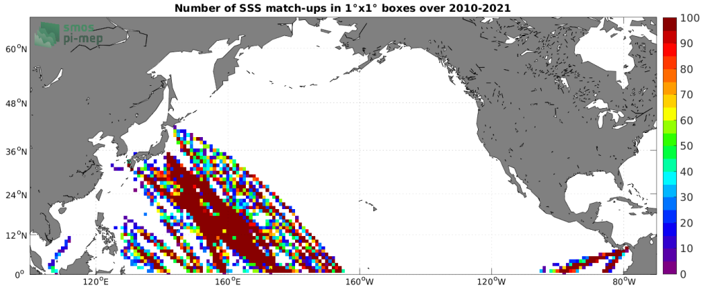
Figure 4: Number of SSS match-ups between TSG (LEGOS-DM) SSS and the SMOS SSS L2Q v330 - 0.25 Deg (CATDS-CPDC) SSS product for the North Pacific Ocean Pi-MEP region over 1^\circ \times 1^\circ boxes and for the full satellite product period.
