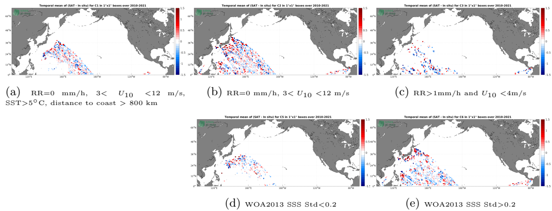
Figure 12: Temporal mean gridded over spatial boxes of size 1^\circ \times 1^\circ of \Delta SSS (SMOS SSS L2Q v330 - 0.25 Deg (CATDS-CPDC) - TSG (LEGOS-DM)) for 5 different subdatasets corresponding to: RR=0 mm/h, 3 < U_{10} < 12 m/s, SST >5^\circ C, distance to coast > 800 km (a), RR=0 mm/h, 3 < U_{10} < 12 m/s (b), RR >1 mm/h and U_{10} < 4 m/s (c), WOA2013 SSS Std <0.2 (d), WOA2013 SSS Std >0.2 (e).
