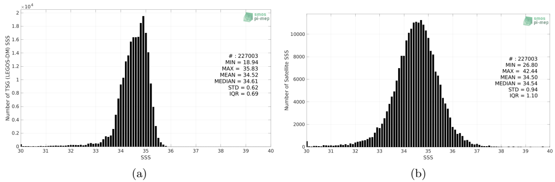
Figure 2: Histograms of SSS from TSG (LEGOS-DM) (a) and SMOS SSS L2Q v330 - 0.25 Deg (CATDS-CPDC) (b) considering all match-up pairs per bins of 0.1 over the North Pacific Ocean Pi-MEP region and for the full satellite product period.
