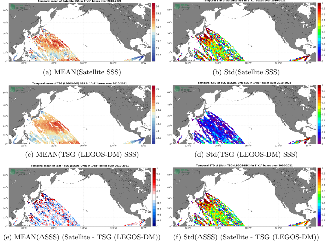
Figure 6: Temporal mean (left) and Std (right) of SSS from SMOS SSS L2Q v330 - 0.25 Deg (CATDS-CPDC) (top), TSG (LEGOS-DM) (middle), and of \Delta\text{SSS} (Satellite - TSG (LEGOS-DM)). Only match-up pairs are used to generate these maps.
