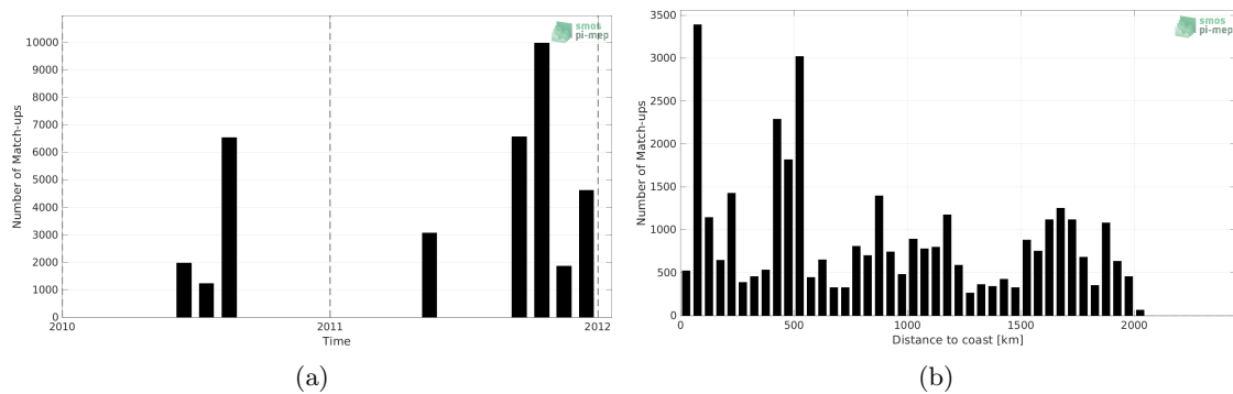
Figure 1: Number of match-ups between TSG (GOSUD-Sailing-ship) and SMOS SSS L2Q v330 - 0.25 Deg (CATDS-CPDC) SSS as a function of time (a) and as function of the distance to coast (b) over the North Pacific Ocean Pi-MEP region and for the full satellite product period.
