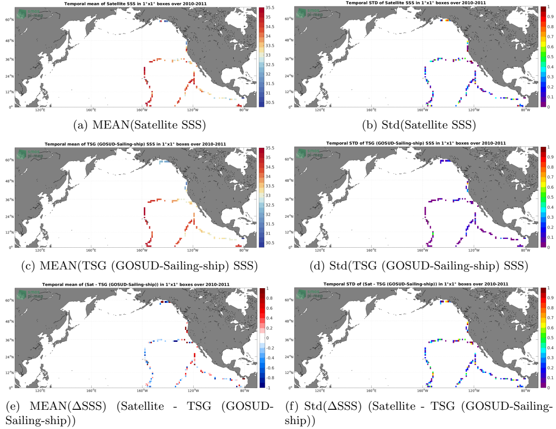
Figure 6: Temporal mean (left) and Std (right) of SSS from SMOS SSS L2Q v330 - 0.25 Deg (CATDS-CPDC) (top), TSG (GOSUD-Sailing-ship) (middle), and of \Delta SSS (Satellite - TSG (GOSUD-Sailing-ship)). Only match-up pairs are used to generate these maps.
