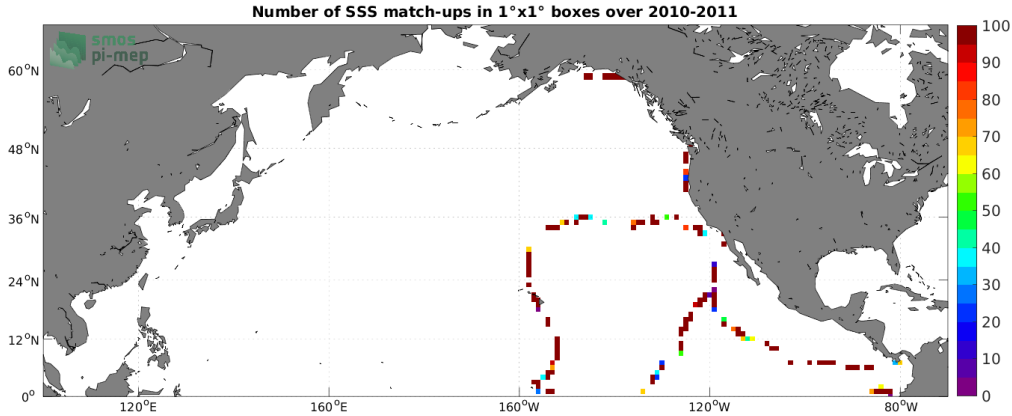
Figure 4: Number of SSS match-ups between TSG (GOSUD-Sailing-ship) SSS and the SMOS SSS L2Q v330 - 0.25 Deg (CATDS-CPDC) SSS product for the North Pacific Ocean Pi-MEP region over 1^\circ \times 1^\circ boxes and for the full satellite product period.
