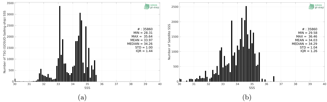
Figure 2: Histograms of SSS from TSG (GOSUD-Sailing-ship) (a) and SMOS SSS L2Q v330 - 0.25 Deg (CATDS-CPDC) (b) considering all match-up pairs per bins of 0.1 over the North Pacific Ocean Pi-MEP region and for the full satellite product period.
