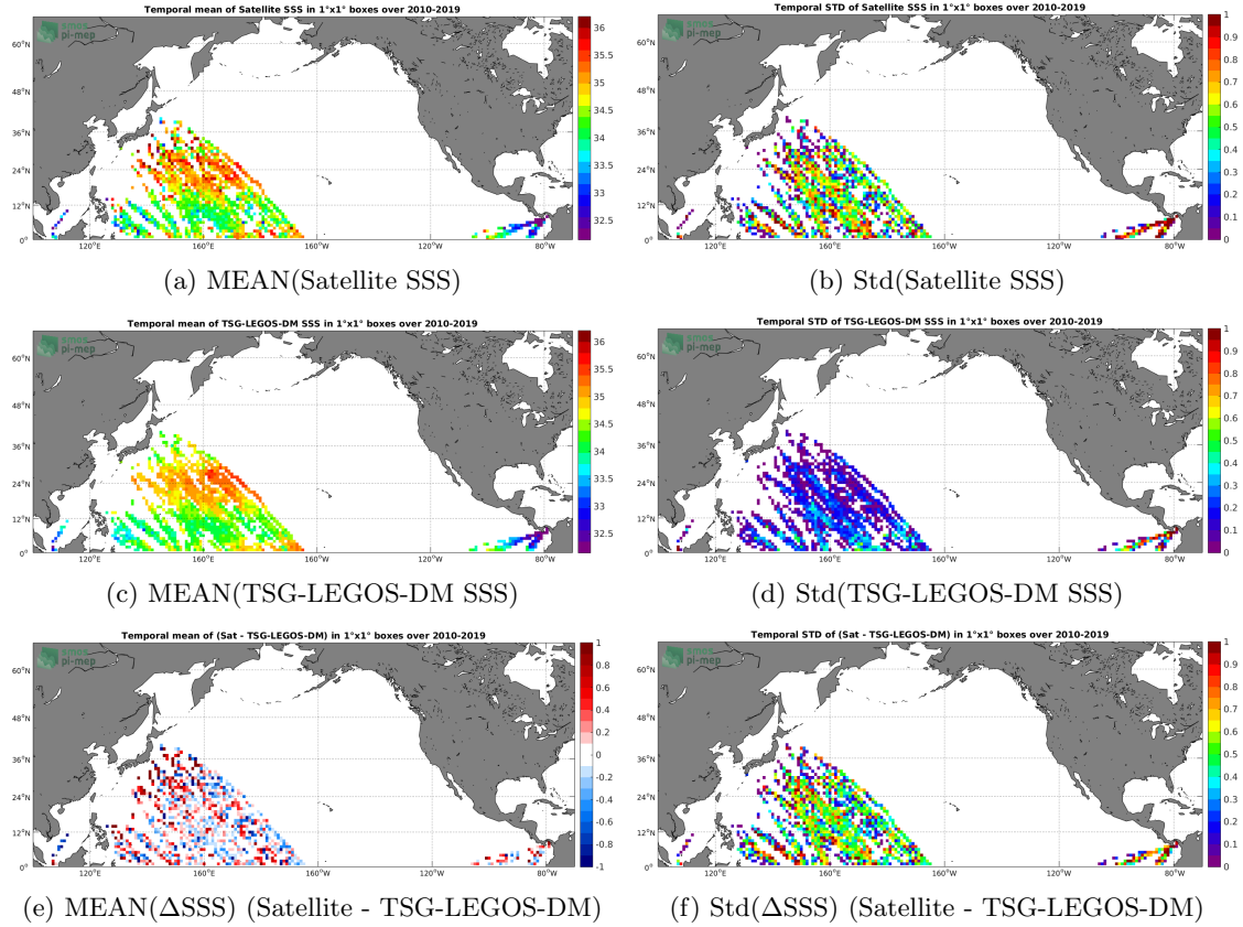
Figure 6: Temporal mean (left) and Std (right) of SSS from SMOS L2Q v321 - 0.25 Deg (CATDS-CPDC) (top), TSG-LEGOS-DM (middle), and of \Delta SSS (Satellite - TSG-LEGOS-DM). Only match-up pairs are used to generate these maps.
