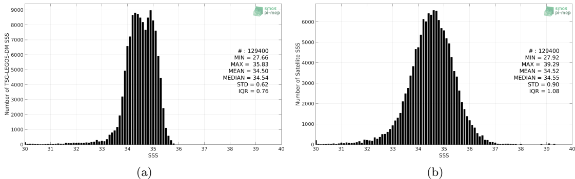
Figure 2: Histograms of SSS from TSG-LEGOS-DM (a) and SMOS L2Q v321 - 0.25 Deg (CATDS-CPDC) (b) considering all match-up pairs per bins of 0.1 over the North Pacific Ocean Pi-MEP region and for the full satellite product period.
