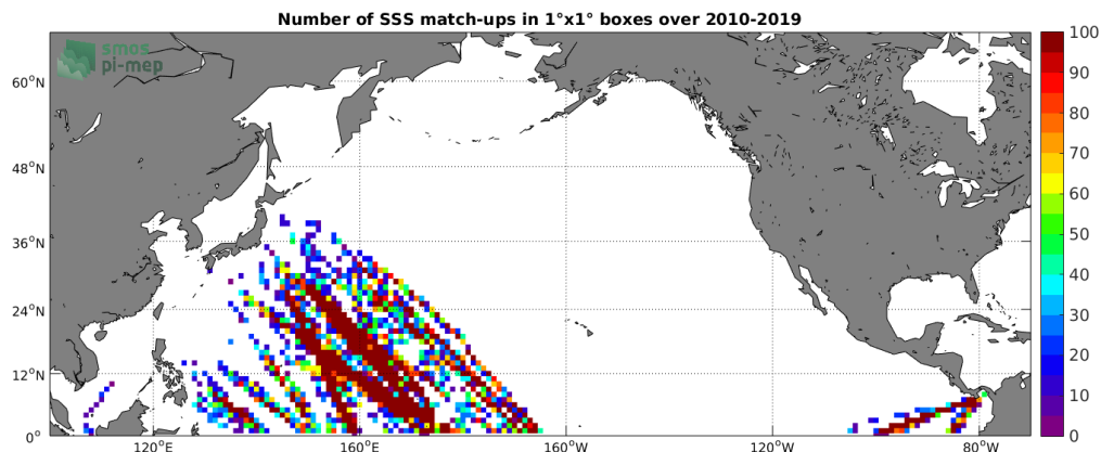
Figure 4: Number of SSS match-ups between TSG-LEGOS-DM SSS and the SMOS L2Q v321 - 0.25 Deg (CATDS-CPDC) SSS product for the North Pacific Ocean Pi-MEP region over 1^\circ \times 1^\circ boxes and for the full satellite product period.
