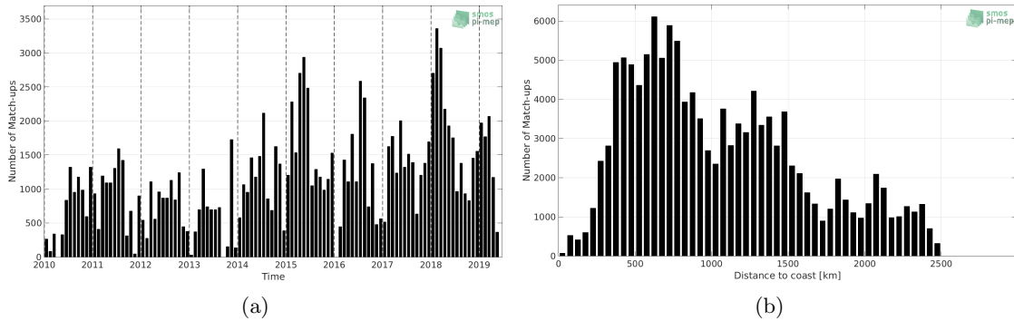
Figure 1: Number of match-ups between TSG-LEGOS-DM and SMOS L2Q v321 - 0.25 Deg (CATDS-CPDC) SSS as a function of time (a) and as function of the distance to coast (b) over the North Pacific Ocean Pi-MEP region and for the full satellite product period.
