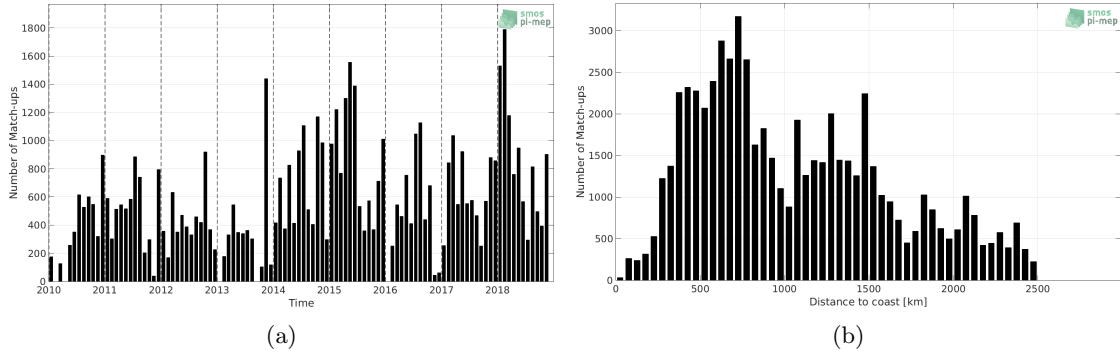
Figure 1: Number of match-ups between TSG-LEGOS-DM and SMOS-L3-CATDS-CPDC-V321-L2Q SSS as a function of time (a) and as function of the distance to coast (b) over the North Pacific Ocean Pi-MEP region and for the full satellite product period.
