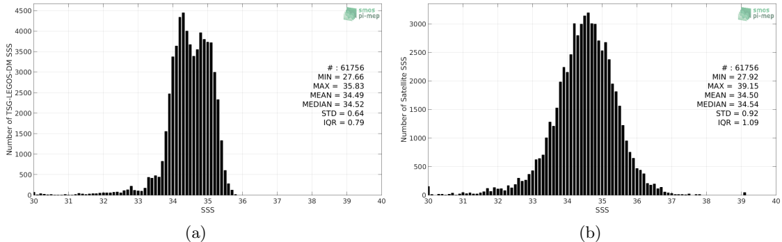
Figure 2: Histograms of SSS from TSG-LEGOS-DM (a) and SMOS-L3-CATDS-CPDC-V321-L2Q (b) considering all match-up pairs per bins of 0.1 over the North Pacific Ocean Pi-MEP region and for the full satellite product period.
