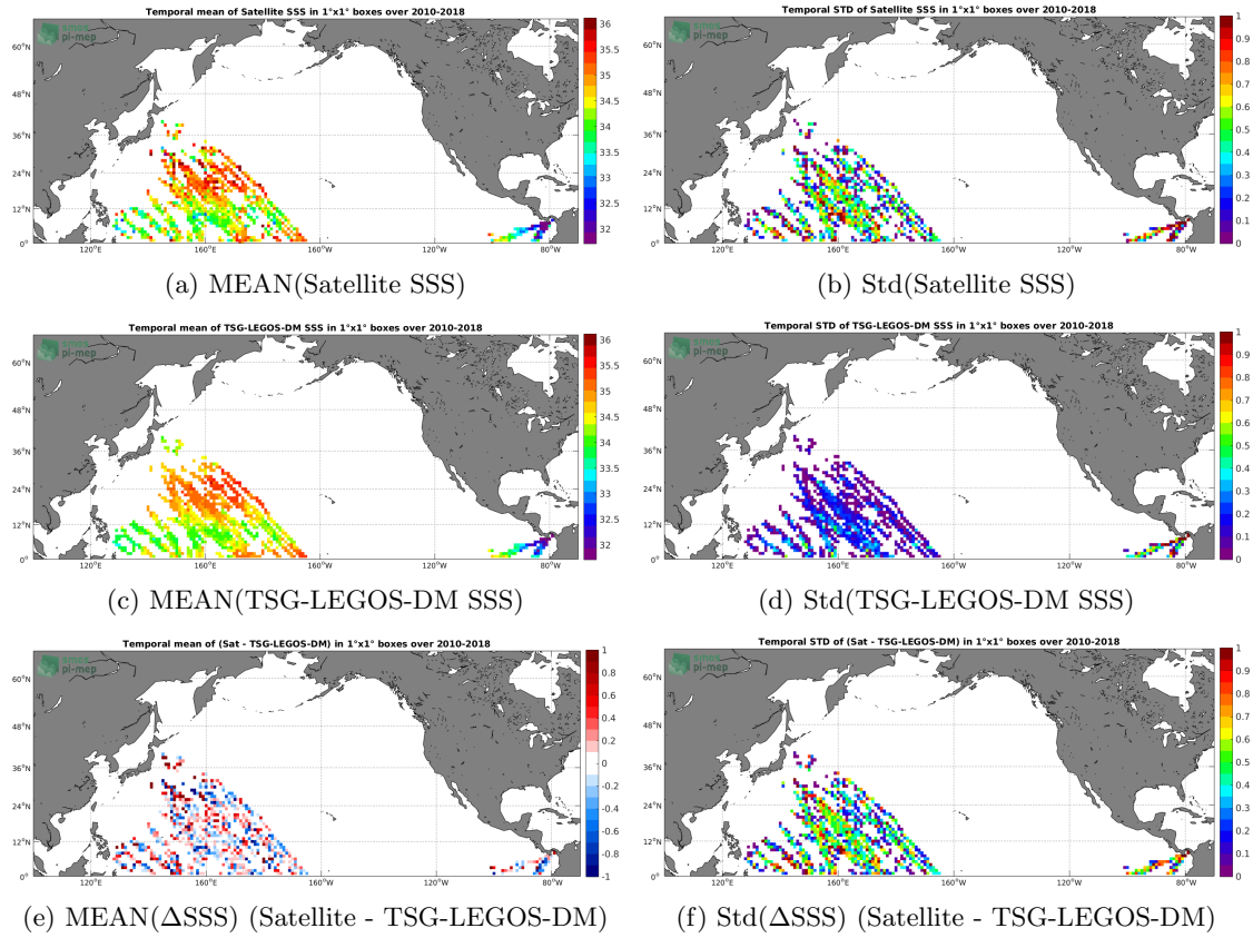
Figure 6: Temporal mean (left) and Std (right) of SSS from SMOS-L3-CATDS-CPDC-V321-L2Q (top), TSG-LEGOS-DM (middle), and of \Delta SSS (Satellite - TSG-LEGOS-DM). Only match-up pairs are used to generate these maps.
