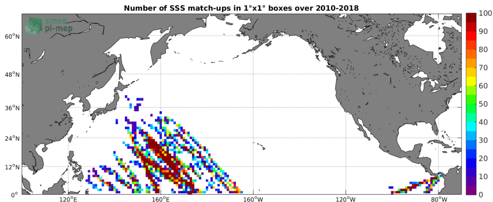
Figure 4: Number of SSS match-ups between TSG-LEGOS-DM SSS and the SMOS-L3-CATDS-CPDC-V321-L2Q SSS product for the North Pacific Ocean Pi-MEP region over 1^\circ \times 1^\circ boxes and for the full satellite product period.
