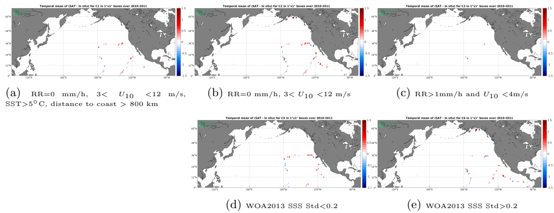
Figure 12: Temporal mean gridded over spatial boxes of size 1^\circ \times 1^\circ of \Delta\text{SSS} (SMOS SSS L2Q v321 - 0.25 Deg (CATDS-CPDC) - TSG (GOSUD-Sailing-ship)) for 5 different subdatasets corresponding to:RR=0 mm/h, 3 < U_{10} < 12 m/s, SST>5°C, distance to coast > 800 km (a), RR=0 mm/h, 3 < U_{10} < 12 m/s (b), RR>1mm/h and U_{10} < 4 m/s (c), WOA2013 SSS Std<0.2 (d), WOA2013 SSS Std>0.2 (e).
