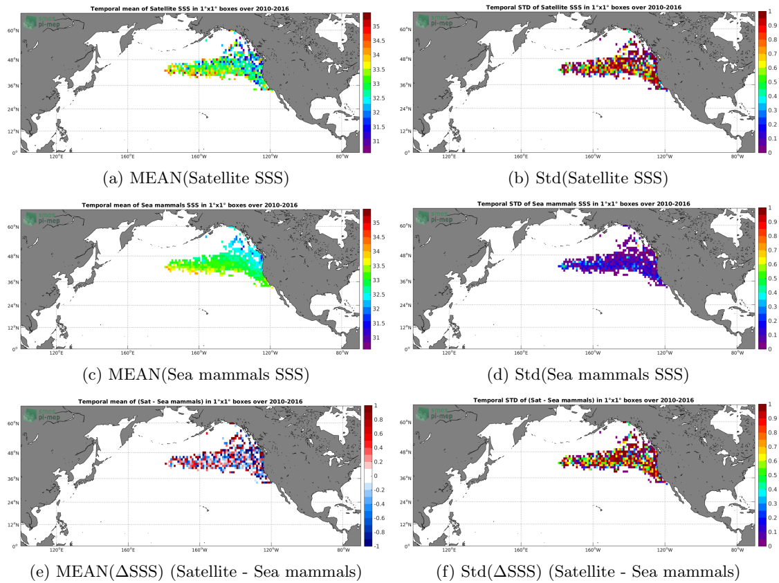
Figure 6: Temporal mean (left) and Std (right) of SSS from SMOS L2Q v321 - 0.25 Deg (CATDS-CPDC) (top), Sea mammals (middle), and of \Delta SSS (Satellite - Sea mammals). Only match-up pairs are used to generate these maps.
