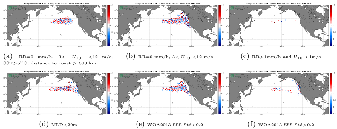
Figure 12: Temporal mean gridded over spatial boxes of size 1^\circ \times 1^\circ of \Delta SSS (SMOS L2Q v321 - 0.25 Deg (CATDS-CPDC) - Sea mammals) for 6 different subdatasets corresponding to:RR=0 mm/h, 3 < U_{10} < 12 m/s, SST >5^\circ C, distance to coast > 800 km (a), RR=0 mm/h, 3 < U_{10} < 12 m/s (b), RR >1 mm/h and U_{10} < 4 m/s (c),MLD <20 m (d),WOA2013 SSS Std <0.2 (e),WOA2013 SSS Std >0.2 (f).
