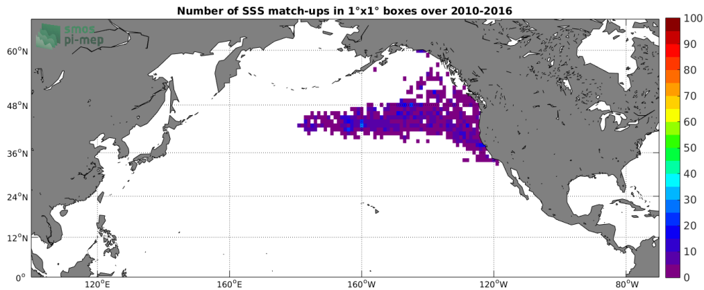
Figure 4: Number of SSS match-ups between Sea mammals SSS and the SMOS L2Q v321 - 0.25 Deg (CATDS-CPDC) SSS product for the North Pacific Ocean Pi-MEP region over 1^\circ \times 1^\circ boxes and for the full satellite product period.
