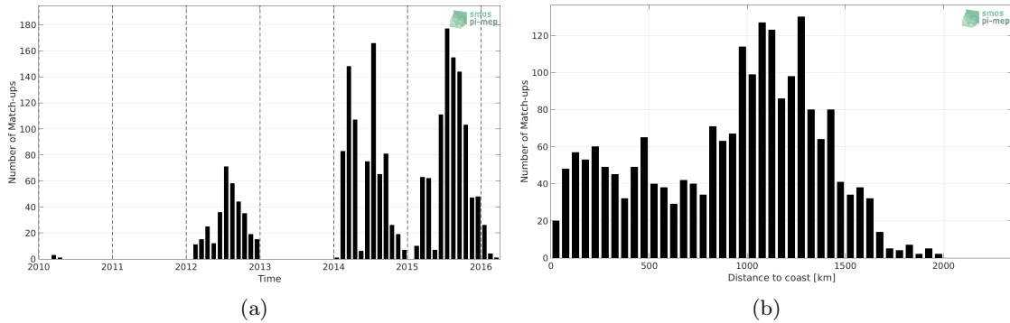
Figure 1: Number of match-ups between Sea mammals and SMOS L2Q v321 - 0.25 Deg (CATDS-CPDC) SSS as a function of time (a) and as function of the distance to coast (b) over the North Pacific Ocean Pi-MEP region and for the full satellite product period.
