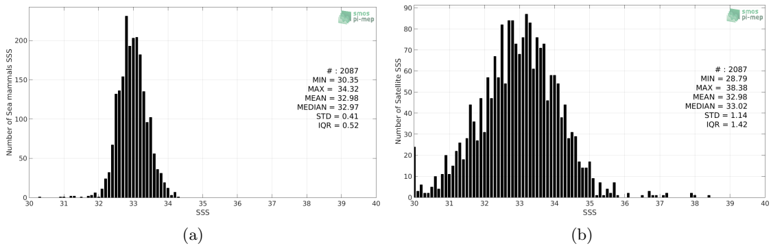
Figure 2: Histograms of SSS from Sea mammals (a) and SMOS L2Q v321 - 0.25 Deg (CATDS-CPDC) (b) considering all match-up pairs per bins of 0.1 over the North Pacific Ocean Pi-MEP region and for the full satellite product period.
