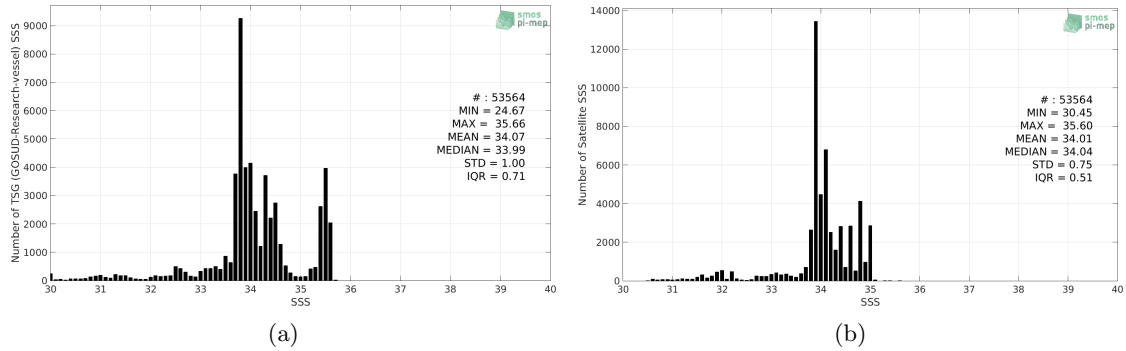
Figure 2: Histograms of SSS from TSG (GOSUD-Research-vessel) (a) and SMOS SSS L3 v317 - Monthly - 25 km (CATDS-CPDC) (b) considering all match-up pairs per bins of 0.1 over the North Pacific Ocean Pi-MEP region and for the full satellite product period.
