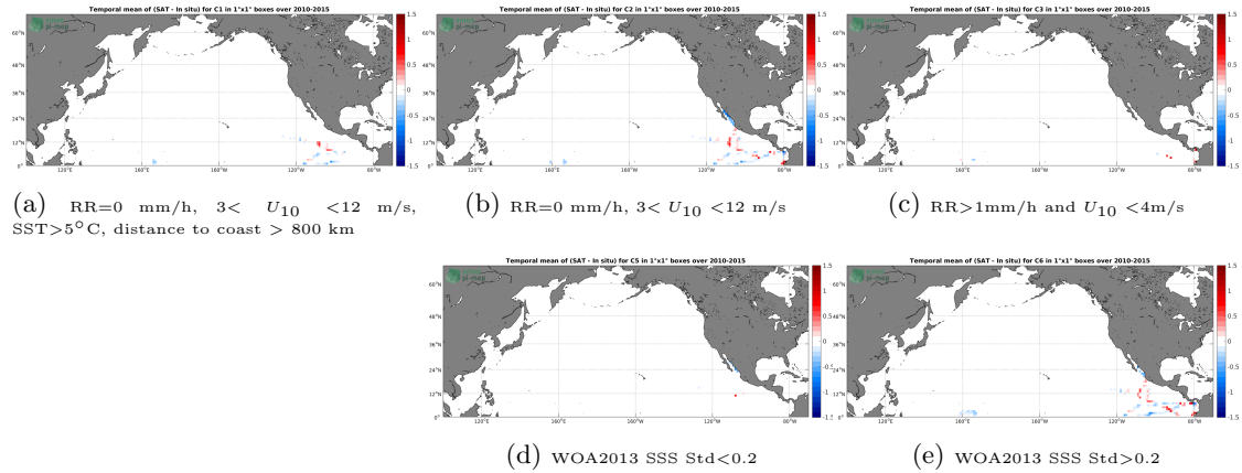
Figure 12: Temporal mean gridded over spatial boxes of size 1^{\circ}\times 1^{\circ} of \Delta SSS (SMOS SSS L3 v317 - Monthly - 25 km (CATDS-CPDC) - TSG (GOSUD-Research-vessel)) for 5 different subdatasets corresponding to:RR=0 mm/h, 3 < U_{10} < 12 m/s, SST >5^{\circ}\text{C} , distance to coast > 800 km (a), RR=0 mm/h, 3 < U_{10} < 12 m/s (b), RR >1 mm/h and U_{10} < 4 m/s (c), WOA2013 SSS Std <0.2 (d), WOA2013 SSS Std >0.2 (e).
