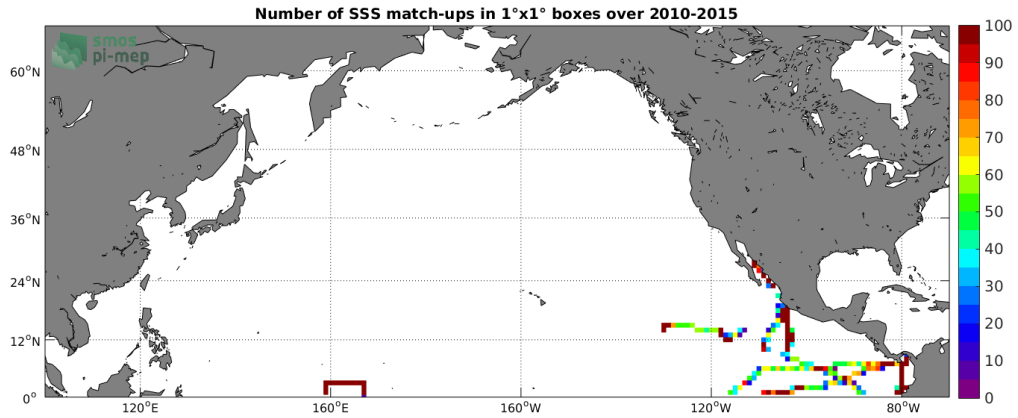
Figure 4: Number of SSS match-ups between TSG (GOSUD-Research-vessel) SSS and the SMOS SSS L3 v317 - Monthly - 25 km (CATDS-CPDC) SSS product for the North Pacific Ocean Pi-MEP region over 1^\circ \times 1^\circ boxes and for the full satellite product period.
