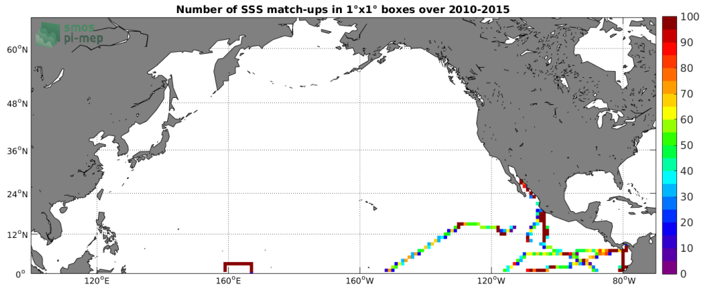
Figure 4: Number of SSS match-ups between TSG-GOSUD-Research-vessel SSS and the SMOS L3 v317 - Monthly - 25 km (CATDS-CPDC) SSS product for the North Pacific Ocean Pi-MEP region over 1°x1° boxes and for the full satellite product period.
