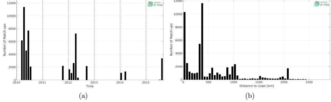
Figure 1: Number of match-ups between TSG-GOSUD-Research-vessel and SMOS L3 v317 - Monthly - 25 km (CATDS-CPDC) SSS as a function of time (a) and as function of the distance to coast (b) over the North Pacific Ocean Pi-MEP region and for the full satellite product period.
