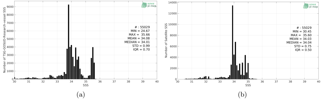
Figure 2: Histograms of SSS from TSG-GOSUD-Research-vessel (a) and SMOS L3 v317 - Monthly - 25 km (CATDS-CPDC) (b) considering all match-up pairs per bins of 0.1 over the North Pacific Ocean Pi-MEP region and for the full satellite product period.
