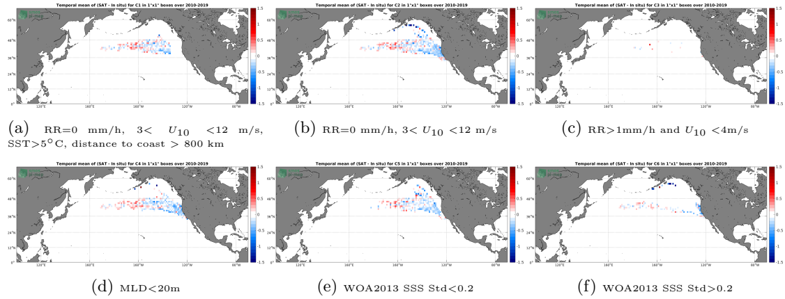
Figure 12: Temporal mean gridded over spatial boxes of size 1^\circ \times 1^\circ of \Delta SSS (SMOS SSS L3 v317 - Monthly - 25 km (CATDS-CPDC) - Marine mammals) for 6 different subdatasets corresponding to: RR=0 mm/h, 3 < U_{10} < 12 m/s, SST > 5^\circ C , distance to coast > 800 km (a), RR=0 mm/h, 3 < U_{10} < 12 m/s (b), RR > 1 mm/h and U_{10} < 4 m/s (c), MLD < 20 m (d), WOA2013 SSS Std < 0.2 (e), WOA2013 SSS Std > 0.2 (f).
