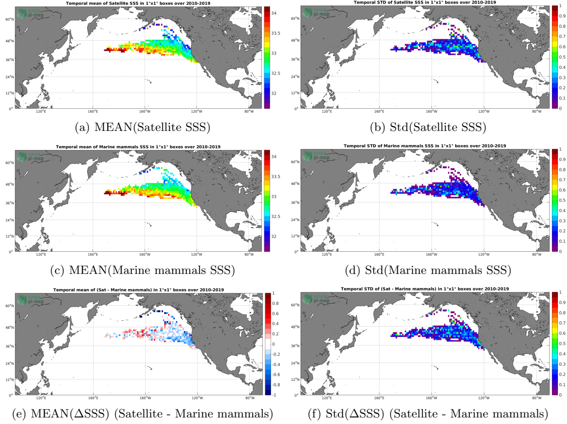
Figure 6: Temporal mean (left) and Std (right) of SSS from SMOS SSS L3 v317 - Monthly - 25 km (CATDS-CPDC) (top), Marine mammals (middle), and of \Delta SSS (Satellite - Marine mammals). Only match-up pairs are used to generate these maps.
