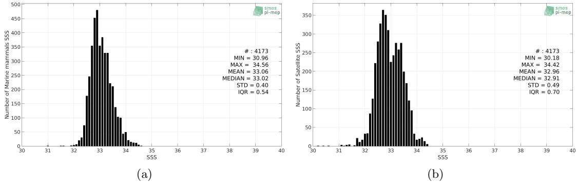
Figure 2: Histograms of SSS from Marine mammals (a) and SMOS SSS L3 v317 - Monthly - 25 km (CATDS-CPDC) (b) considering all match-up pairs per bins of 0.1 over the North Pacific Ocean Pi-MEP region and for the full satellite product period.
