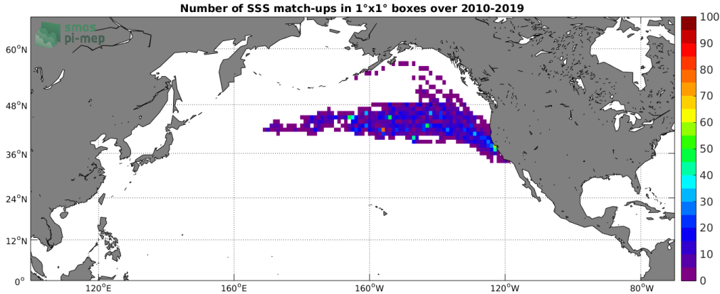
Figure 4: Number of SSS match-ups between Marine mammals SSS and the SMOS SSS L3 v317 - Monthly - 25 km (CATDS-CPDC) SSS product for the North Pacific Ocean Pi-MEP region over 1^\circ \times 1^\circ boxes and for the full satellite product period.
