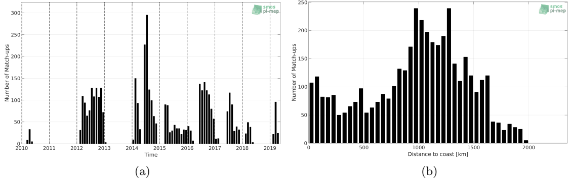
Figure 1: Number of match-ups between Marine mammals and SMOS SSS L3 v317 - Monthly - 25 km (CATDS-CPDC) SSS as a function of time (a) and as function of the distance to coast (b) over the North Pacific Ocean Pi-MEP region and for the full satellite product period.
