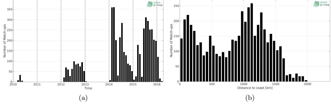
Figure 1: Number of match-ups between Sea mammals and SMOS SSS L3 v317 - Monthly - 25 km (CATDS-CPDC) SSS as a function of time (a) and as function of the distance to coast (b) over the North Pacific Ocean Pi-MEP region and for the full satellite product period.
