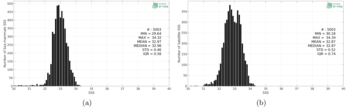
Figure 2: Histograms of SSS from Sea mammals (a) and SMOS SSS L3 v317 - Monthly - 25 km (CATDS-CPDC) (b) considering all match-up pairs per bins of 0.1 over the North Pacific Ocean Pi-MEP region and for the full satellite product period.
