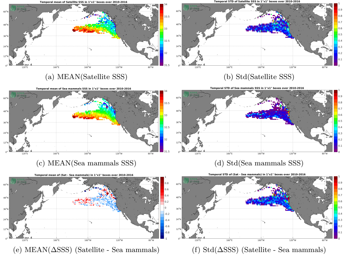
Figure 6: Temporal mean (left) and Std (right) of SSS from SMOS SSS L3 v317 - Monthly - 25 km (CATDS-CPDC) (top), Sea mammals (middle), and of \Delta SSS (Satellite - Sea mammals). Only match-up pairs are used to generate these maps.
