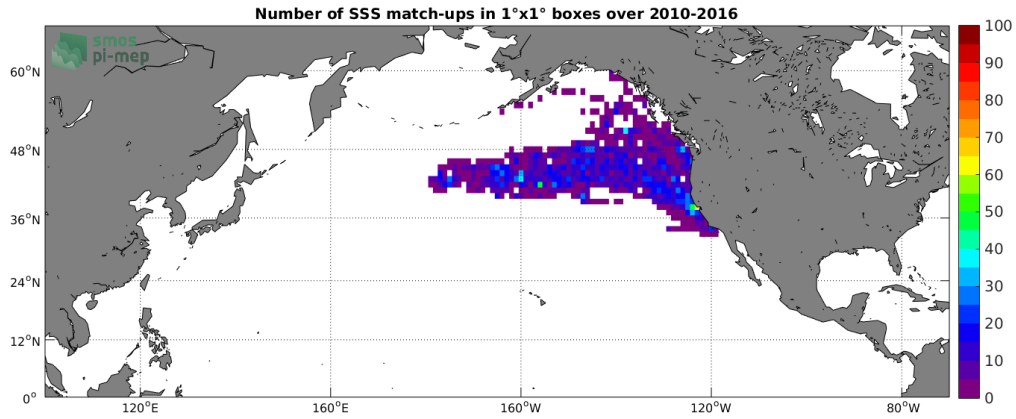
Figure 4: Number of SSS match-ups between Sea mammals SSS and the SMOS SSS L3 v317 - Monthly - 25 km (CATDS-CPDC) SSS product for the North Pacific Ocean Pi-MEP region over 1°x1° boxes and for the full satellite product period.
