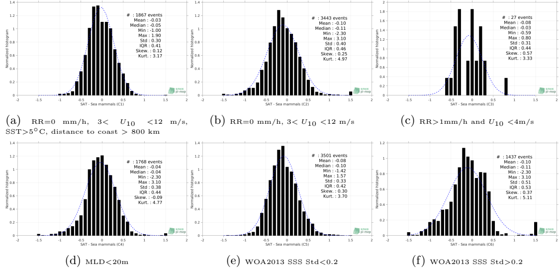
Figure 13: Normalized histogram of \Delta\text{SSS} (SMOS SSS L3 v317 - Monthly - 25 km (CATDS-CPDC) - Sea mammals) for 6 different subdatasets corresponding to: RR=0 mm/h, 3 < U_{10} < 12 m/s, SST>5°C, distance to coast > 800 km (a), RR=0 mm/h, 3 < U_{10} < 12 m/s (b), RR>1mm/h and U_{10} < 4 m/s (c), MLD<20m (d), WOA2013 SSS Std<0.2 (e), WOA2013 SSS Std>0.2 (f).
