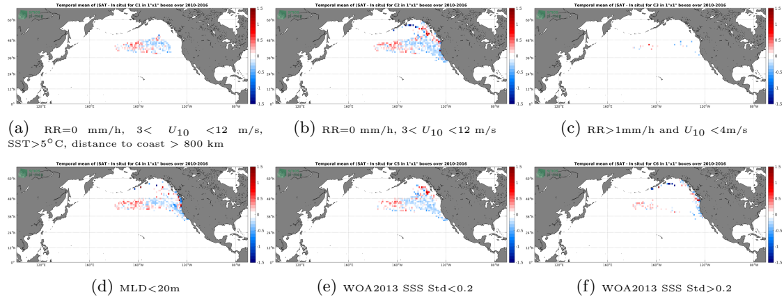
Figure 12: Temporal mean gridded over spatial boxes of size 1^\circ \times 1^\circ of \Delta SSS (SMOS SSS L3 v317 - Monthly - 25 km (CATDS-CPDC) - Sea mammals) for 6 different subdatasets corresponding to: RR=0 mm/h, 3 < U_{10} < 12 m/s, SST > 5^\circ C , distance to coast > 800 km (a), RR=0 mm/h, 3 < U_{10} < 12 m/s (b), RR > 1 mm/h and U_{10} < 4 m/s (c), MLD < 20 m (d), WOA2013 SSS Std < 0.2 (e), WOA2013 SSS Std > 0.2 (f).
