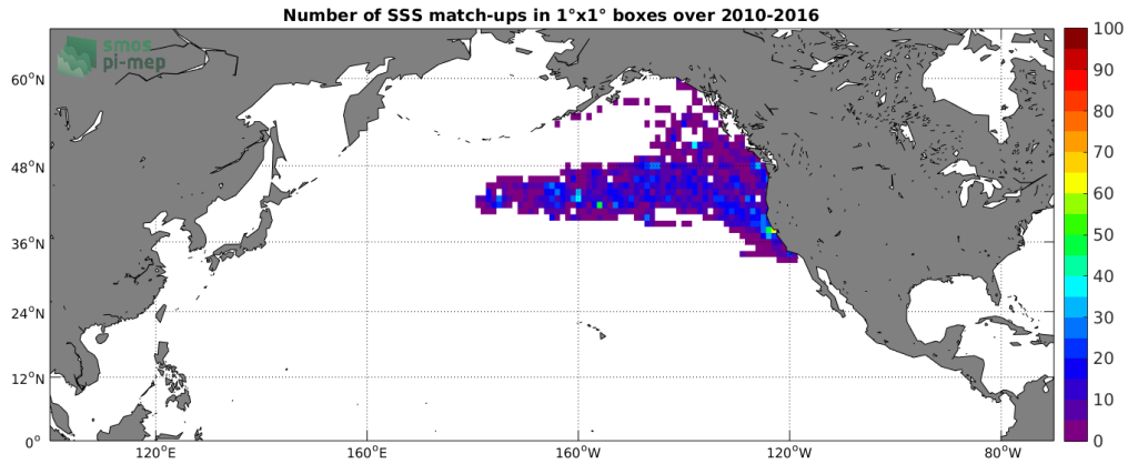
Figure 4: Number of SSS match-ups between Sea mammals SSS and the SMOS L3 v317 - Monthly - 25 km (CATDS-CPDC) SSS product for the North Pacific Ocean Pi-MEP region over 1°x1° boxes and for the full satellite product period.
