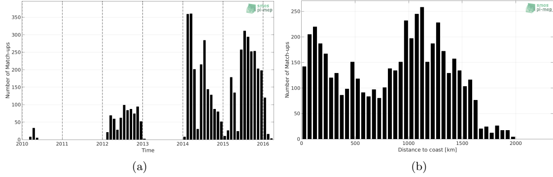
Figure 1: Number of match-ups between Sea mammals and SMOS L3 v317 - Monthly - 25 km (CATDS-CPDC) SSS as a function of time (a) and as function of the distance to coast (b) over the North Pacific Ocean Pi-MEP region and for the full satellite product period.
