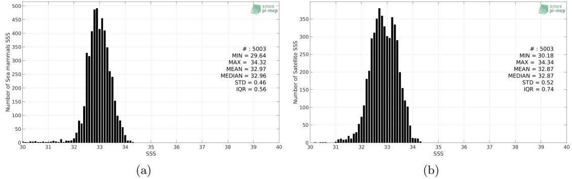
Figure 2: Histograms of SSS from Sea mammals (a) and SMOS L3 v317 - Monthly - 25 km (CATDS-CPDC) (b) considering all match-up pairs per bins of 0.1 over the North Pacific Ocean Pi-MEP region and for the full satellite product period.
