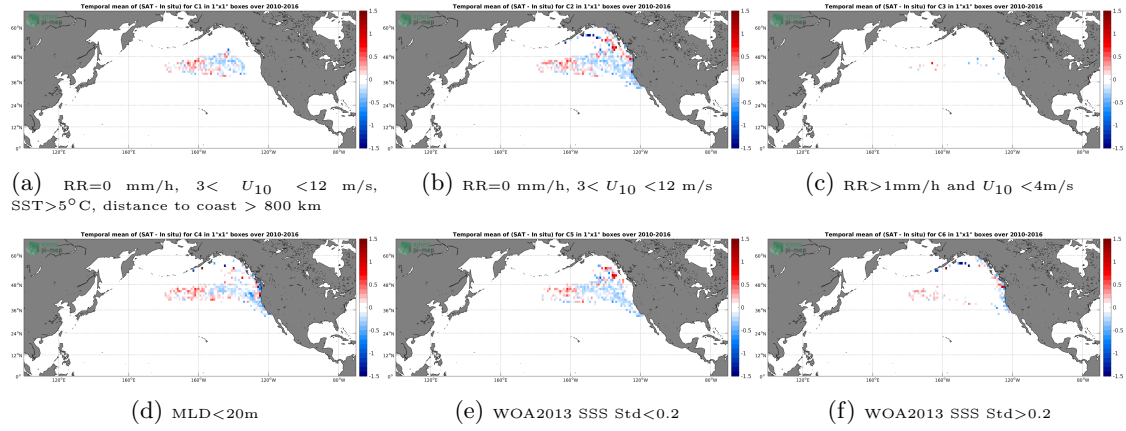
Figure 12: Temporal mean gridded over spatial boxes of size 1^\circ \times 1^\circ of \Delta SSS (SMOS L3 v317 - Monthly - 25 km (CATDS-CPDC) - Sea mammals) for 6 different subdatasets corresponding to: RR=0 mm/h, 3 < U_{10} < 12 m/s, SST > 5^\circ\text{C} , distance to coast > 800 km (a), RR=0 mm/h, 3 < U_{10} < 12 m/s (b), RR > 1 mm/h and U_{10} < 4 m/s (c), MLD < 20 m (d), WOA2013 SSS Std < 0.2 (e), WOA2013 SSS Std > 0.2 (f).
