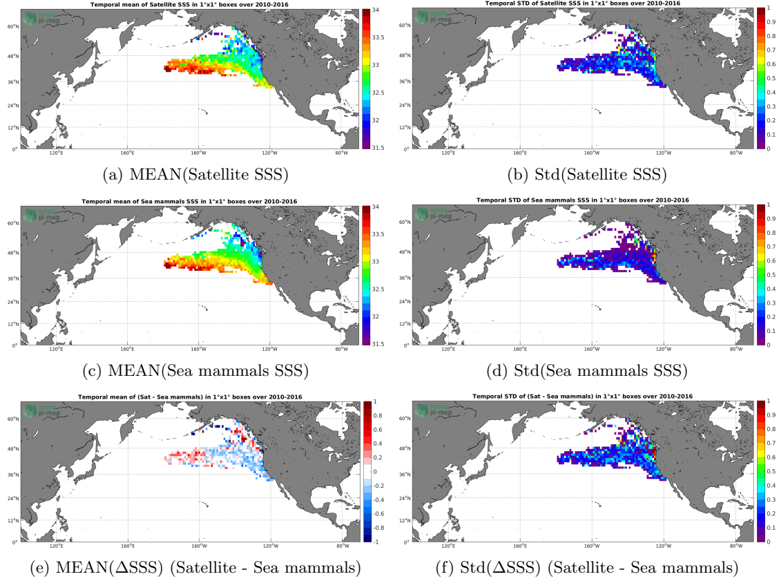
Figure 6: Temporal mean (left) and Std (right) of SSS from SMOS L3 v317 - Monthly - 25 km (CATDS-CPDC) (top), Sea mammals (middle), and of \Delta SSS (Satellite - Sea mammals). Only match-up pairs are used to generate these maps.
