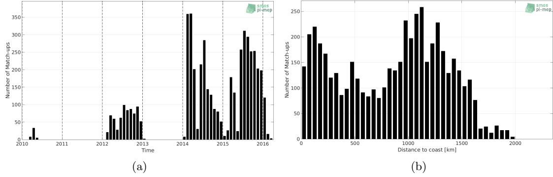
Figure 1: Number of match-ups between Sea mammals and SMOS-L3-CATDS-CPDC-V317-MONTHLY-25KM SSS as a function of time (a) and as function of the distance to coast (b) over the North Pacific Ocean Pi-MEP region and for the full satellite product period.
