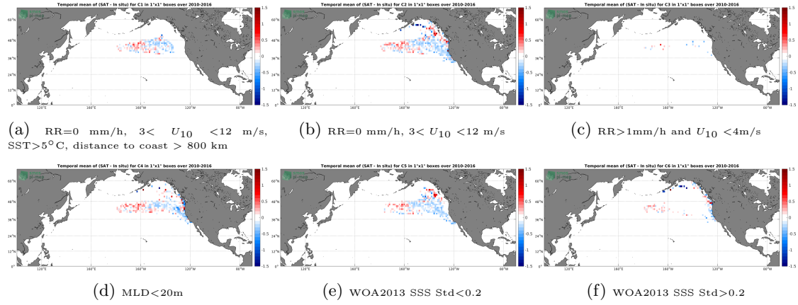
Figure 12: Temporal mean gridded over spatial boxes of size 1^\circ \times 1^\circ of \Delta SSS (SMOS-L3-CATDS-CPDC-V317-MONTHLY-25KM - Sea mammals) for 6 different subdatasets corresponding to: RR=0 mm/h, 3 < U_{10} < 12 m/s, SST > 5^\circ\text{C} , distance to coast > 800 km (a), RR=0 mm/h, 3 < U_{10} < 12 m/s (b), RR > 1 mm/h and U_{10} < 4 m/s (c), MLD < 20 m (d), WOA2013 SSS Std < 0.2 (e), WOA2013 SSS Std > 0.2 (f).
