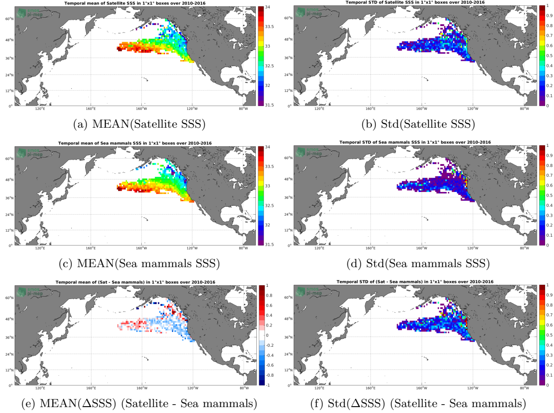
Figure 6: Temporal mean (left) and Std (right) of SSS from SMOS-L3-CATDS-CPDC-V317-MONTHLY-25KM (top), Sea mammals (middle), and of \Delta SSS (Satellite - Sea mammals). Only match-up pairs are used to generate these maps.
