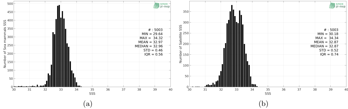
Figure 2: Histograms of SSS from Sea mammals (a) and SMOS-L3-CATDS-CPDC-V317-MONTHLY-25KM (b) considering all match-up pairs per bins of 0.1 over the North Pacific Ocean Pi-MEP region and for the full satellite product period.
