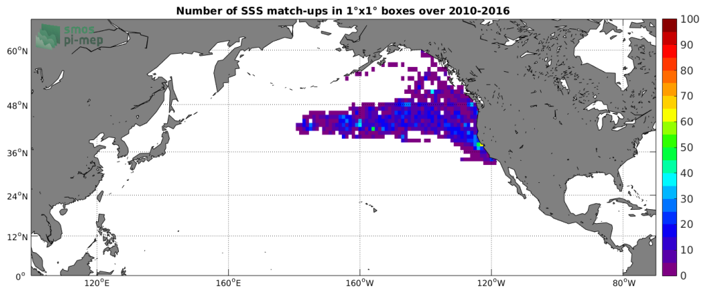
Figure 4: Number of SSS match-ups between Sea mammals SSS and the SMOS-L3-CATDS-CPDC-V317-MONTHLY-25KM SSS product for the North Pacific Ocean Pi-MEP region over 1^\circ \times 1^\circ boxes and for the full satellite product period.
