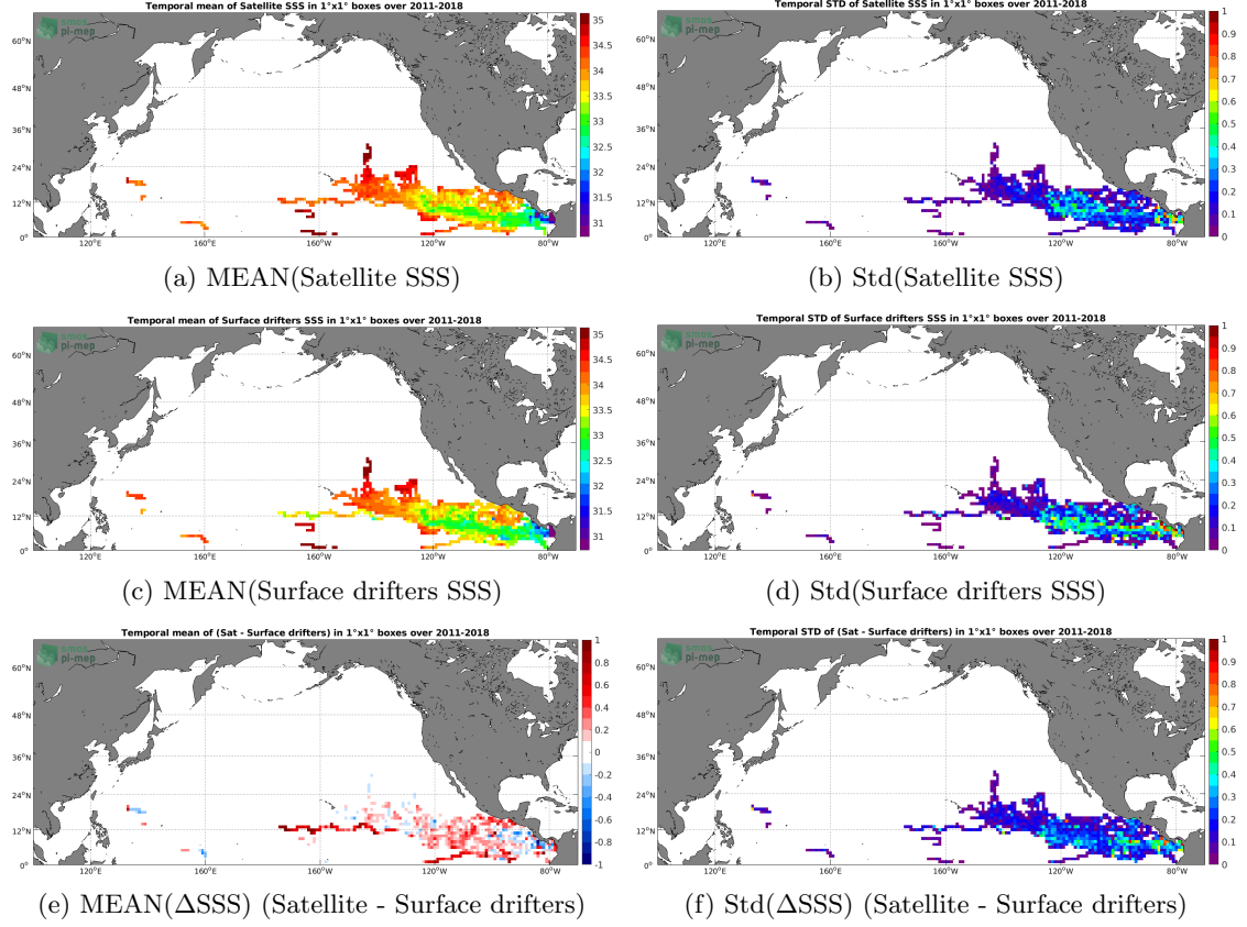
Figure 5: Temporal mean (left) and Std (right) of SSS from SMOS SSS L3 v317 - Monthly - 25 km (CATDS-CPDC) (top), Surface drifters (middle), and of \Delta\text{SSS} (Satellite - Surface drifters). Only match-up pairs are used to generate these maps.
