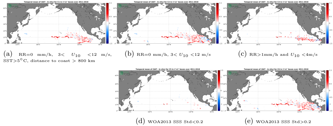
Figure 11: Temporal mean gridded over spatial boxes of size 1^\circ \times 1^\circ of \Delta SSS (SMOS L3 v317 - Monthly - 25 km (CATDS-CPDC) - Surface drifters) for 5 different subdatasets corresponding to: RR=0 mm/h, 3 < U_{10} < 12 m/s, SST > 5^\circ\text{C} , distance to coast > 800 km (a), RR=0 mm/h, 3 < U_{10} < 12 m/s (b), RR > 1 mm/h and U_{10} < 4 m/s (c), WOA2013 SSS Std < 0.2 (d), WOA2013 SSS Std > 0.2 (e).
