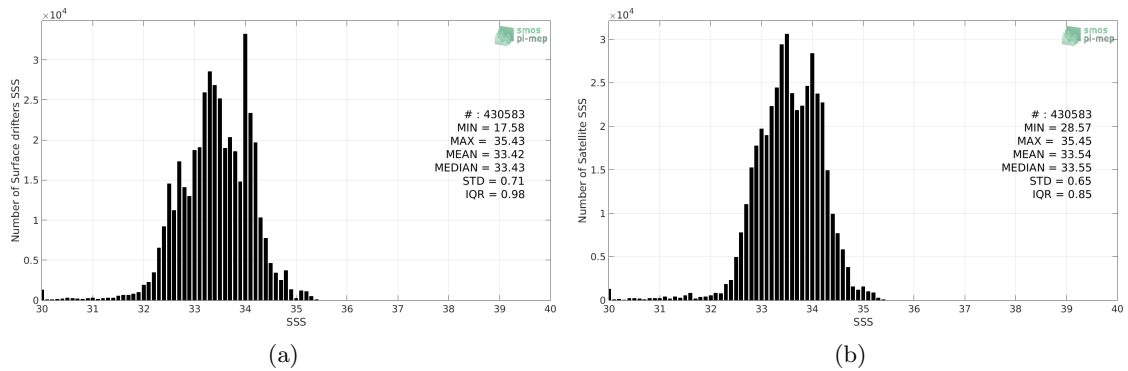
Figure 2: Histograms of SSS from Surface drifters (a) and SMOS L3 v317 - Monthly - 25 km (CATDS-CPDC) (b) considering all match-up pairs per bins of 0.1 over the North Pacific Ocean Pi-MEP region and for the full satellite product period.
