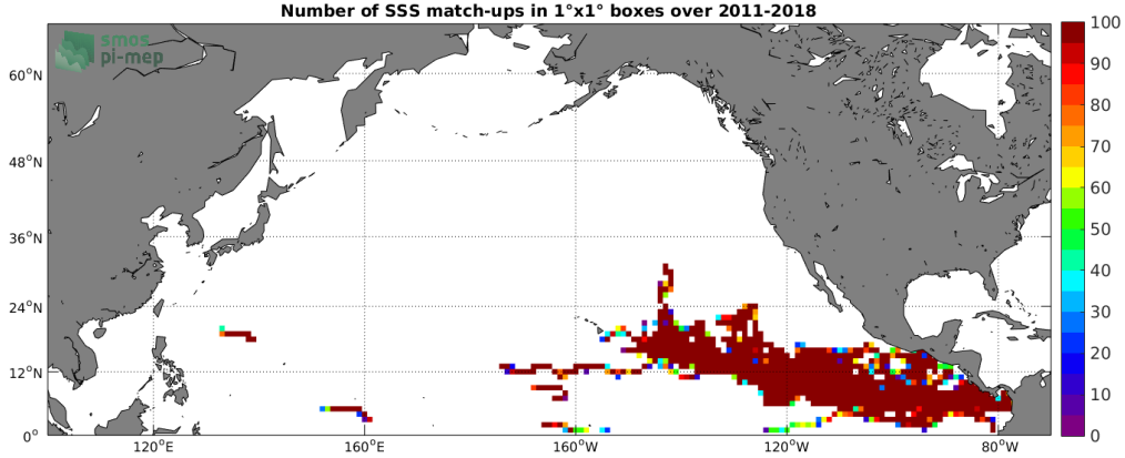
Figure 3: Number of SSS match-ups between Surface drifters SSS and the SMOS L3 v317 - Monthly - 25 km (CATDS-CPDC) SSS product for the North Pacific Ocean Pi-MEP region over 1^\circ \times 1^\circ boxes and for the full satellite product period.
