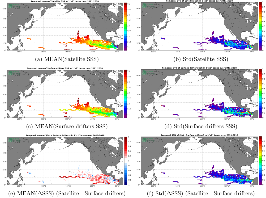
Figure 5: Temporal mean (left) and Std (right) of SSS from SMOS L3 v317 - Monthly - 25 km (CATDS-CPDC) (top), Surface drifters (middle), and of \Delta SSS (Satellite - Surface drifters). Only match-up pairs are used to generate these maps.
