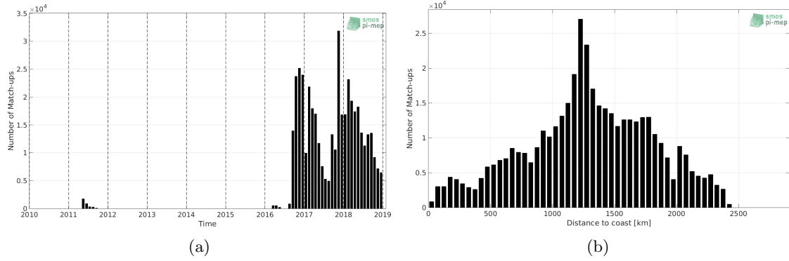
Figure 1: Number of match-ups between Surface drifters and SMOS L3 v317 - Monthly - 25 km (CATDS-CPDC) SSS as a function of time (a) and as function of the distance to coast (b) over the North Pacific Ocean Pi-MEP region and for the full satellite product period.
