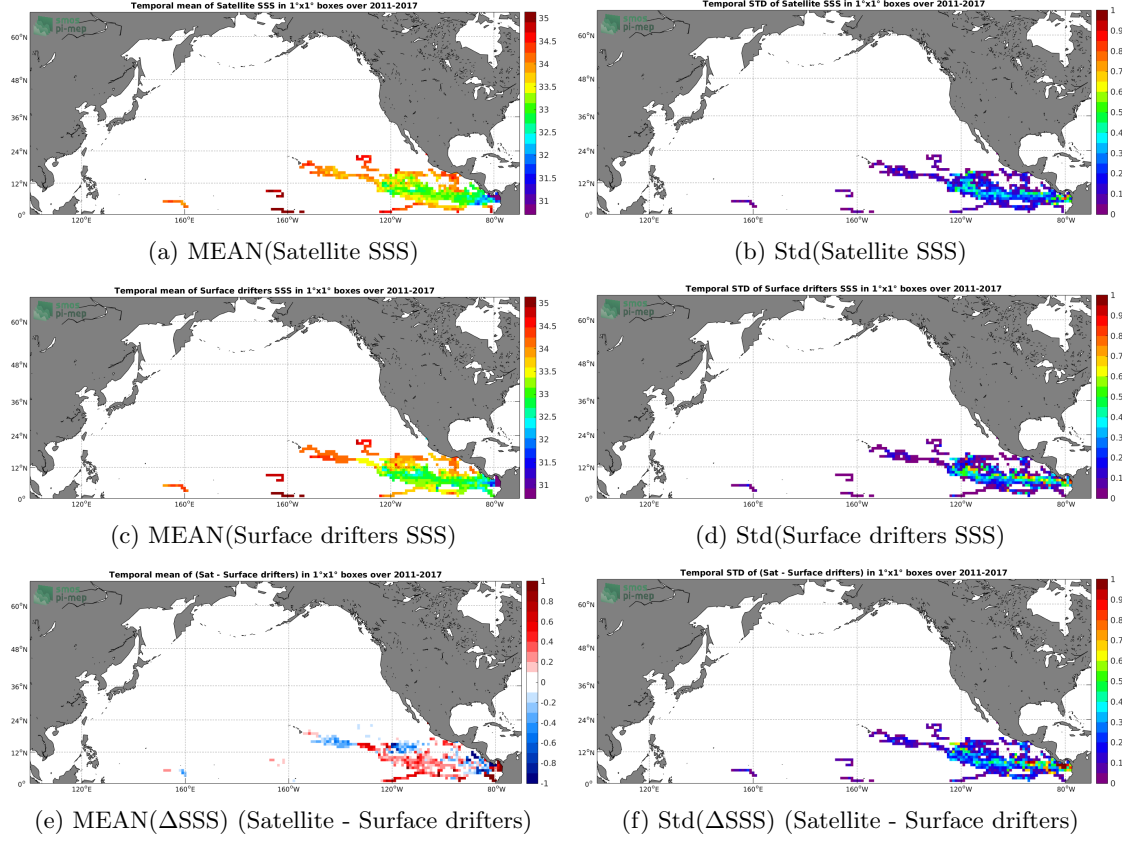
Figure 5: Temporal mean (left) and Std (right) of SSS from SMOS-L3-CATDS-CPDC-V317-MONTHLY-25KM (top), Surface drifters (middle), and of \Delta SSS (Satellite - Surface drifters). Only match-up pairs are used to generate these maps.
