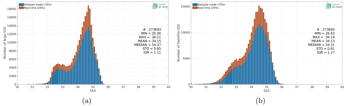
Figure 2: Histograms of SSS from Argo (a) and SMOS SSS L3 v317 - Monthly - 25 km (CATDS-CPDC) (b) considering all match-up pairs per bins of 0.1 over the North Pacific Ocean Pi-MEP region and for the full satellite product period.
