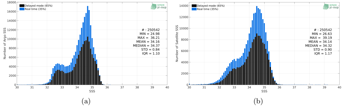
Figure 2: Histograms of SSS from Argo (a) and SMOS L3 v317 - Monthly - 25 km (CATDS-CPDC) (b) considering all match-up pairs per bins of 0.1 over the North Pacific Ocean Pi-MEP region and for the full satellite product period.
