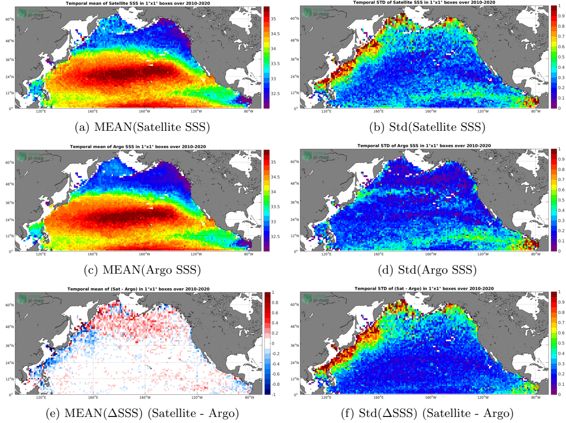
Figure 6: Temporal mean (left) and Std (right) of SSS from SMOS L3 v317 - Monthly - 25 km (CATDS-CPDC) (top), Argo (middle), and of \Delta SSS (Satellite - Argo). Only match-up pairs are used to generate these maps.
