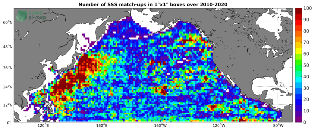
Figure 4: Number of SSS match-ups between Argo SSS and the SMOS L3 v317 - Monthly - 25 km (CATDS-CPDC) SSS product for the North Pacific Ocean Pi-MEP region over 1^\circ \times 1^\circ boxes and for the full satellite product period.
