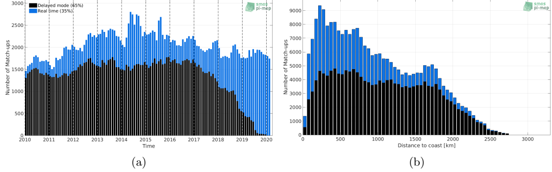
Figure 1: Number of match-ups between Argo and SMOS L3 v317 - Monthly - 25 km (CATDS-CPDC) SSS as a function of time (a) and as function of the distance to coast (b) over the North Pacific Ocean Pi-MEP region and for the full satellite product period.
