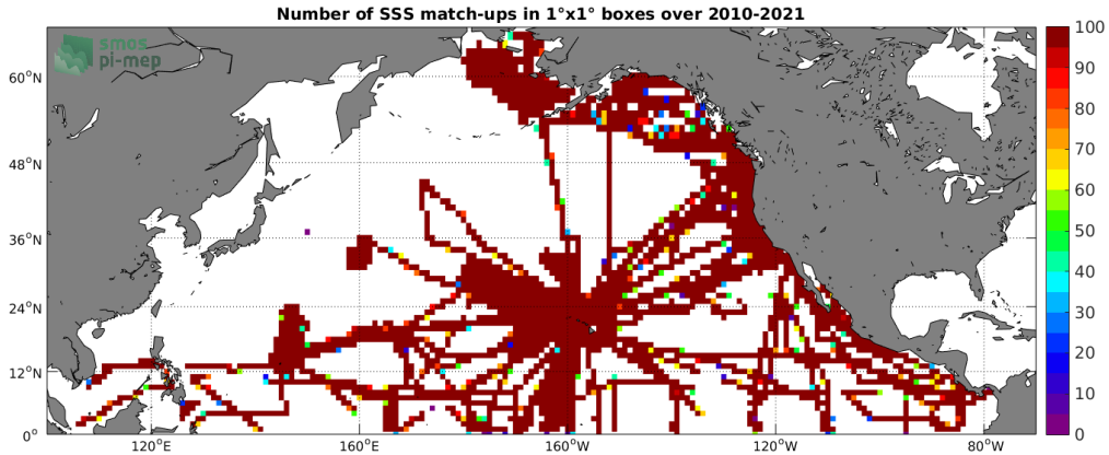
Figure 4: Number of SSS match-ups between TSG (SAMOS) SSS and the SMOS SSS L3 v317 - 10 Days - 25 km (CATDS-CPDC) SSS product for the North Pacific Ocean Pi-MEP region over 1^\circ \times 1^\circ boxes and for the full satellite product period.
