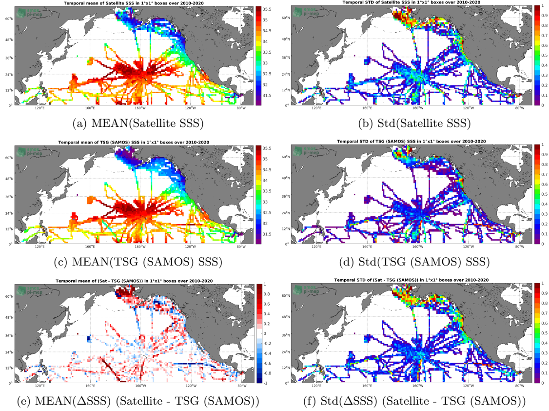
Figure 6: Temporal mean (left) and Std (right) of SSS from SMOS SSS L3 v317 - 10 Days - 25 km (CATDS-CPDC) (top), TSG (SAMOS) (middle), and of \Delta SSS (Satellite - TSG (SAMOS)). Only match-up pairs are used to generate these maps.
