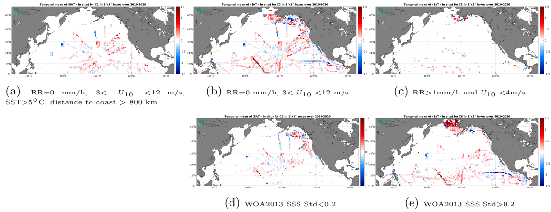
Figure 12: Temporal mean gridded over spatial boxes of size 1^\circ \times 1^\circ of \Delta SSS (SMOS SSS L3 v317 - 10 Days - 25 km (CATDS-CPDC) - TSG (SAMOS)) for 5 different subdatasets corresponding to: RR=0 mm/h, 3 < U_{10} < 12 m/s, SST > 5^\circ C , distance to coast > 800 km (a), RR=0 mm/h, 3 < U_{10} < 12 m/s (b), RR > 1 mm/h and U_{10} < 4 m/s (c), WOA2013 SSS Std < 0.2 (d), WOA2013 SSS Std > 0.2 (e).
