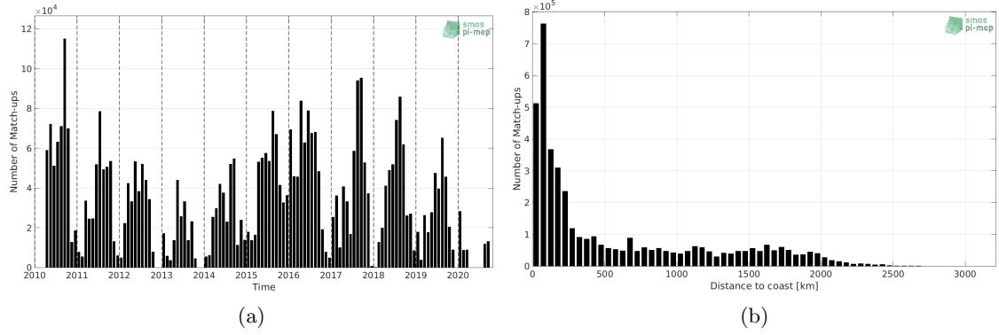
Figure 1: Number of match-ups between TSG (SAMOS) and SMOS SSS L3 v317 - 10 Days - 25 km (CATDS-CPDC) SSS as a function of time (a) and as function of the distance to coast (b) over the North Pacific Ocean Pi-MEP region and for the full satellite product period.
