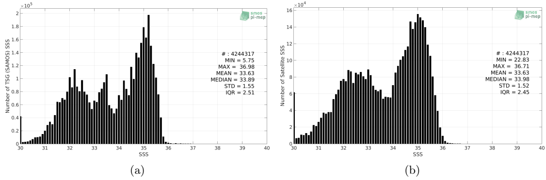
Figure 2: Histograms of SSS from TSG (SAMOS) (a) and SMOS SSS L3 v317 - 10 Days - 25 km (CATDS-CPDC) (b) considering all match-up pairs per bins of 0.1 over the North Pacific Ocean Pi-MEP region and for the full satellite product period.
