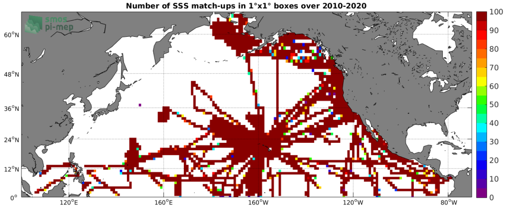
Figure 4: Number of SSS match-ups between TSG (SAMOS) SSS and the SMOS SSS L3 v317 - 10 Days - 25 km (CATDS-CPDC) SSS product for the North Pacific Ocean Pi-MEP region over 1°x1° boxes and for the full satellite product period.
