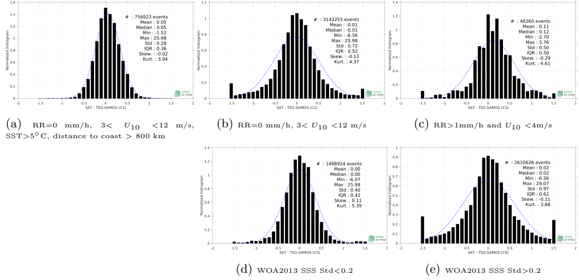
Figure 13: Normalized histogram of \Delta\text{SSS} (SMOS L3 v317 - 10 Days - 25 km (CATDS-CPDC) - TSG-SAMOS) for 5 different subdatasets corresponding to: RR=0 mm/h, 3 < U_{10} < 12 m/s, SST > 5^{\circ}\text{C} , distance to coast > 800 km (a), RR=0 mm/h, 3 < U_{10} < 12 m/s (b), RR > 1 mm/h and U_{10} < 4 m/s (c), WOA2013 SSS Std < 0.2 (d), WOA2013 SSS Std > 0.2 (e).
