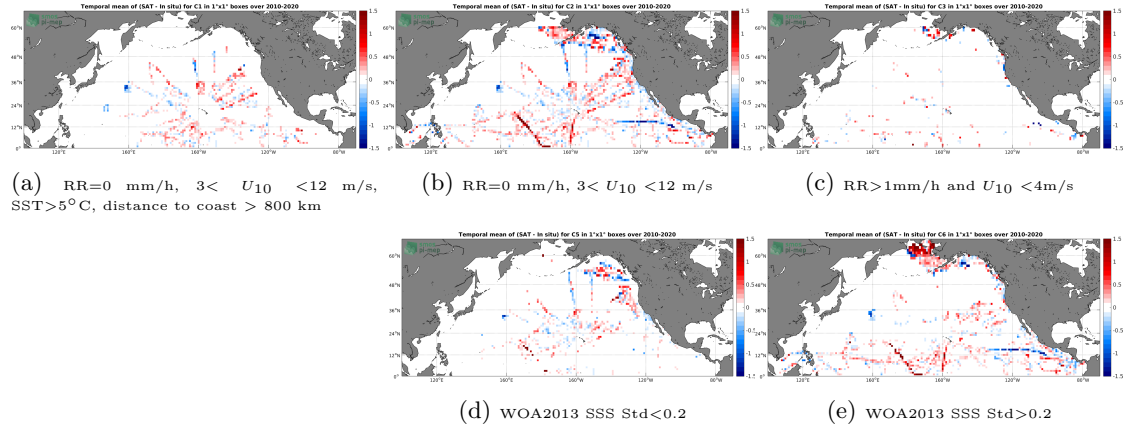
Figure 12: Temporal mean gridded over spatial boxes of size 1^\circ \times 1^\circ of \Delta SSS (SMOS L3 v317 - 10 Days - 25 km (CATDS-CPDC) - TSG-SAMOS) for 5 different subdatasets corresponding to: RR=0 mm/h, 3 < U_{10} < 12 m/s, SST > 5^\circ C , distance to coast > 800 km (a), RR=0 mm/h, 3 < U_{10} < 12 m/s (b), RR > 1 mm/h and U_{10} < 4 m/s (c), WOA2013 SSS Std < 0.2 (d), WOA2013 SSS Std > 0.2 (e).
