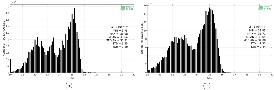
Figure 2: Histograms of SSS from TSG-SAMOS (a) and SMOS L3 v317 - 10 Days - 25 km (CATDS-CPDC) (b) considering all match-up pairs per bins of 0.1 over the North Pacific Ocean Pi-MEP region and for the full satellite product period.
