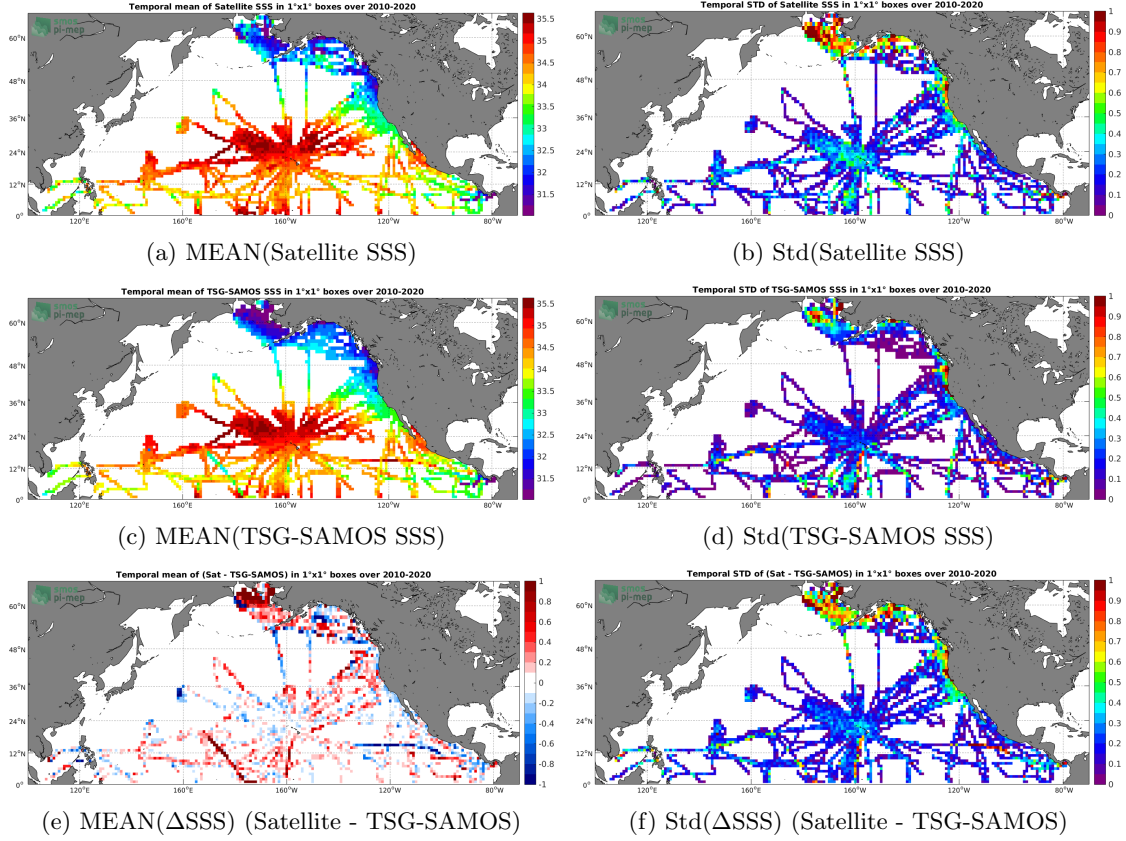
Figure 6: Temporal mean (left) and Std (right) of SSS from SMOS L3 v317 - 10 Days - 25 km (CATDS-CPDC) (top), TSG-SAMOS (middle), and of \Delta SSS (Satellite - TSG-SAMOS). Only match-up pairs are used to generate these maps.
