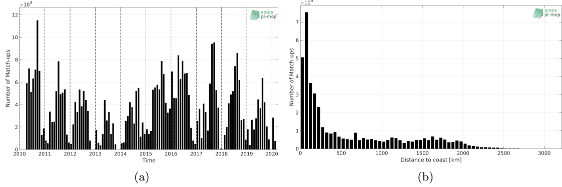
Figure 1: Number of match-ups between TSG-SAMOS and SMOS L3 v317 - 10 Days - 25 km (CATDS-CPDC) SSS as a function of time (a) and as function of the distance to coast (b) over the North Pacific Ocean Pi-MEP region and for the full satellite product period.
