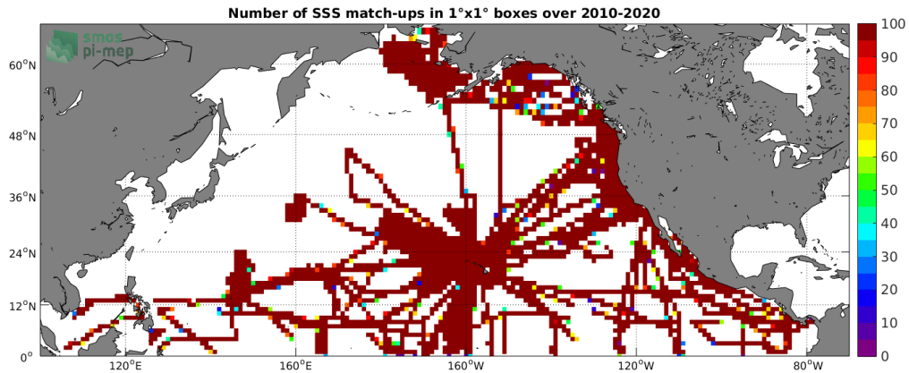
Figure 4: Number of SSS match-ups between TSG-SAMOS SSS and the SMOS L3 v317 - 10 Days - 25 km (CATDS-CPDC) SSS product for the North Pacific Ocean Pi-MEP region over 1°x1° boxes and for the full satellite product period.
