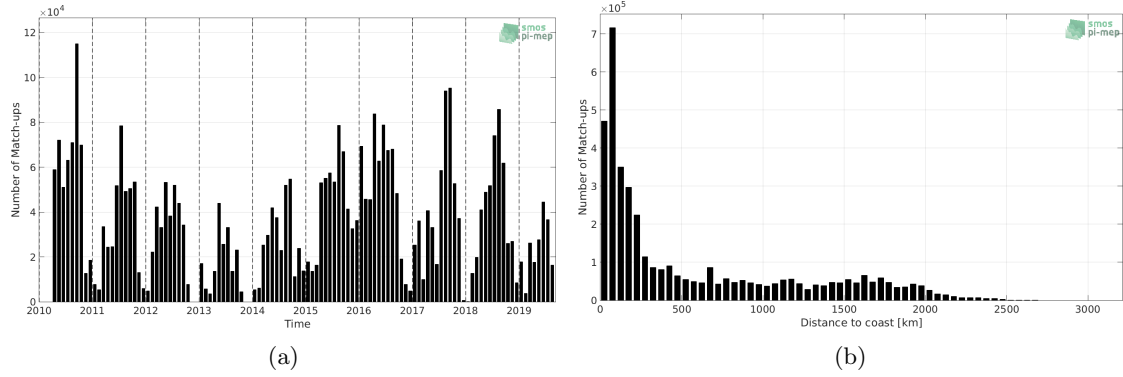
Figure 1: Number of match-ups between TSG-SAMOS and SMOS-L3-CATDS-CPDC-V317-10DAYS-25KM SSS as a function of time (a) and as function of the distance to coast (b) over the North Pacific Ocean Pi-MEP region and for the full satellite product period.
