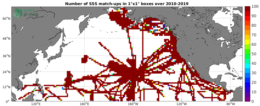
Figure 4: Number of SSS match-ups between TSG-SAMOS SSS and the SMOS-L3-CATDS-CPDC-V317-10DAYS-25KM SSS product for the North Pacific Ocean Pi-MEP region over 1^\circ \times 1^\circ boxes and for the full satellite product period.
