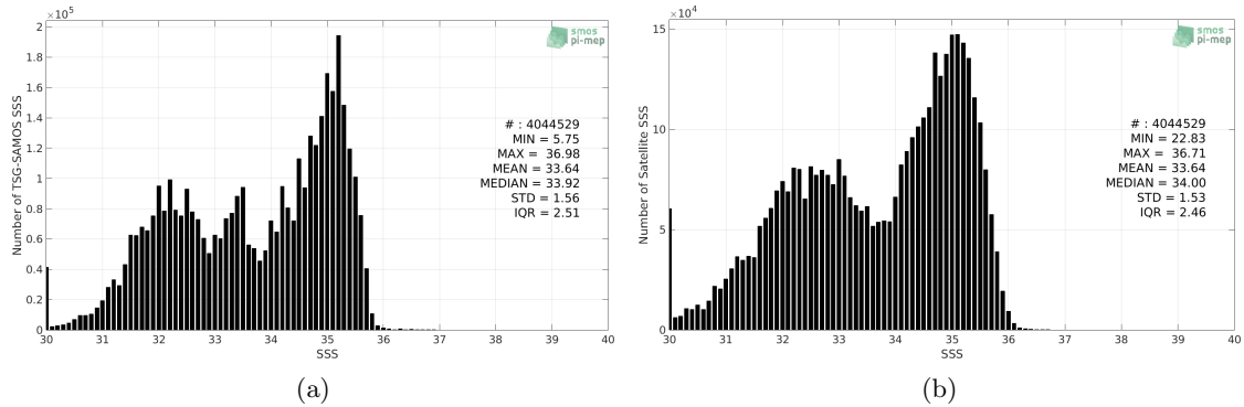
Figure 2: Histograms of SSS from TSG-SAMOS (a) and SMOS-L3-CATDS-CPDC-V317-10DAYS-25KM (b) considering all match-up pairs per bins of 0.1 over the North Pacific Ocean Pi-MEP region and for the full satellite product period.
