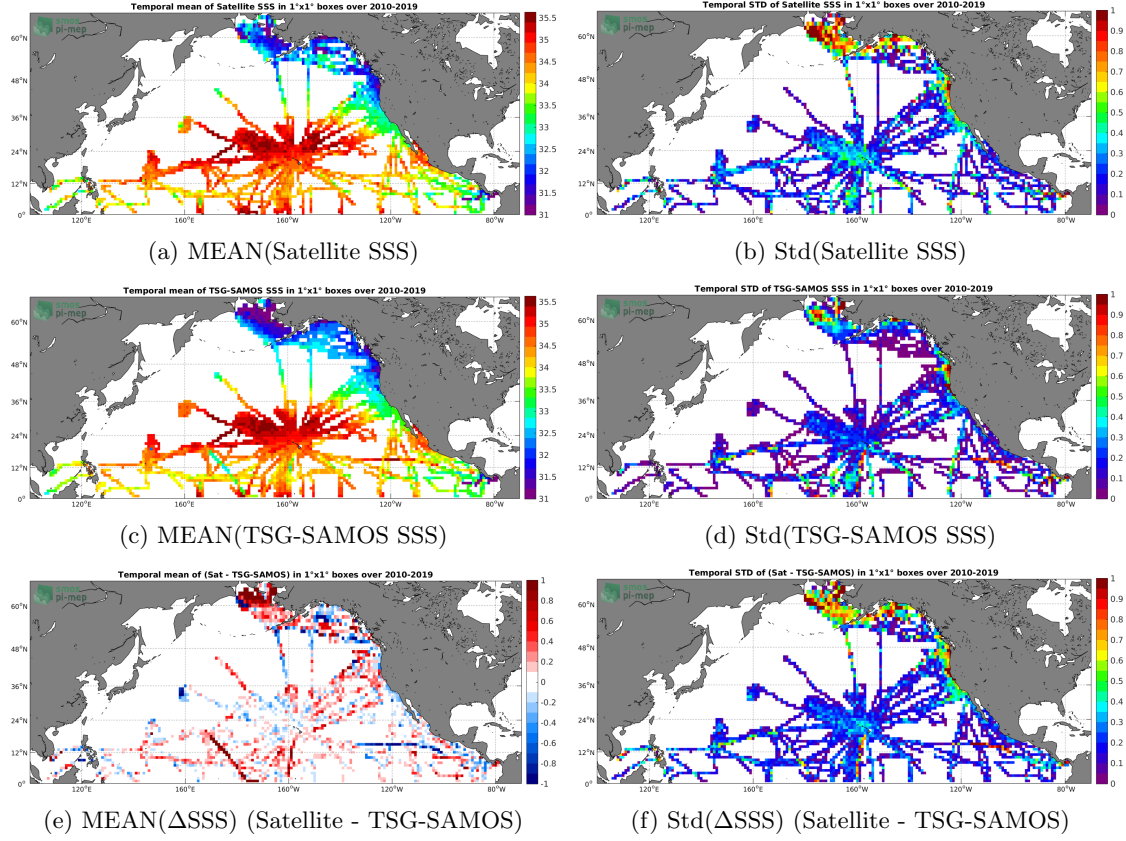
Figure 6: Temporal mean (left) and Std (right) of SSS from SMOS-L3-CATDS-CPDC-V317-10DAYS-25KM (top), TSG-SAMOS (middle), and of \Delta SSS (Satellite - TSG-SAMOS). Only match-up pairs are used to generate these maps.
