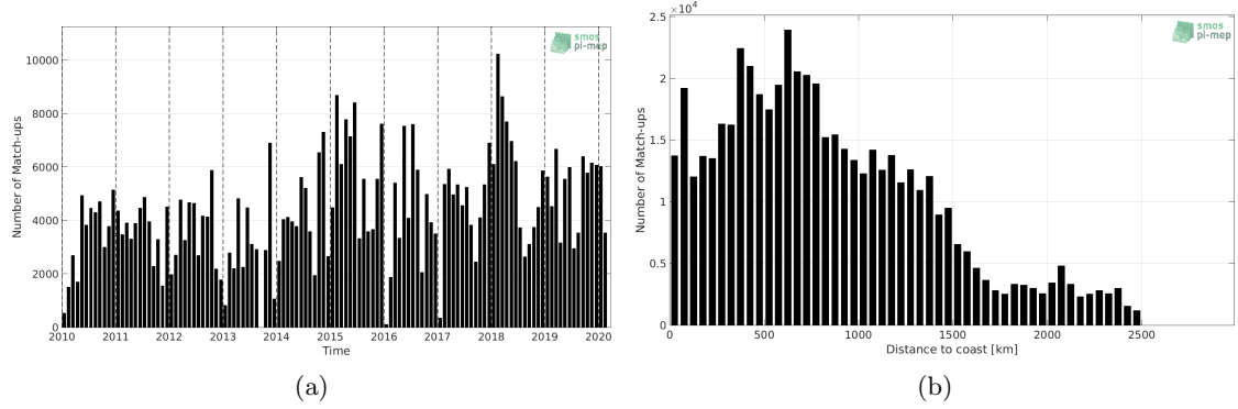
Figure 1: Number of match-ups between TSG (LEGOS-DM) and SMOS SSS L3 v317 - 10 Days - 25 km (CATDS-CPDC) SSS as a function of time (a) and as function of the distance to coast (b) over the North Pacific Ocean Pi-MEP region and for the full satellite product period.
