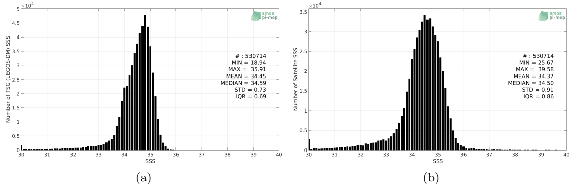
Figure 2: Histograms of SSS from TSG (LEGOS-DM) (a) and SMOS SSS L3 v317 - 10 Days - 25 km (CATDS-CPDC) (b) considering all match-up pairs per bins of 0.1 over the North Pacific Ocean Pi-MEP region and for the full satellite product period.
