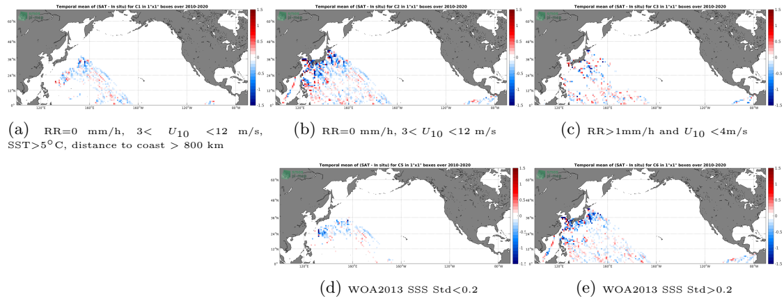
Figure 12: Temporal mean gridded over spatial boxes of size 1^\circ \times 1^\circ of \Delta SSS (SMOS SSS L3 v317 - 10 Days - 25 km (CATDS-CPDC) - TSG (LEGOS-DM)) for 5 different subdatasets corresponding to: RR=0 mm/h, 3 < U_{10} < 12 m/s, SST >5^\circ\text{C} , distance to coast > 800 km (a), RR=0 mm/h, 3 < U_{10} < 12 m/s (b), RR >1 mm/h and U_{10} < 4 m/s (c), WOA2013 SSS Std <0.2 (d), WOA2013 SSS Std >0.2 (e).
