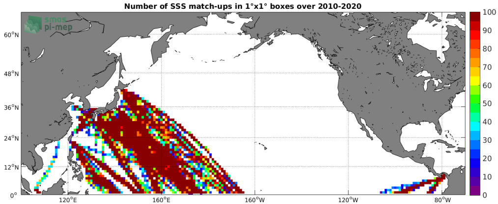
Figure 4: Number of SSS match-ups between TSG (LEGOS-DM) SSS and the SMOS SSS L3 v317 - 10 Days - 25 km (CATDS-CPDC) SSS product for the North Pacific Ocean Pi-MEP region over 1^\circ \times 1^\circ boxes and for the full satellite product period.
