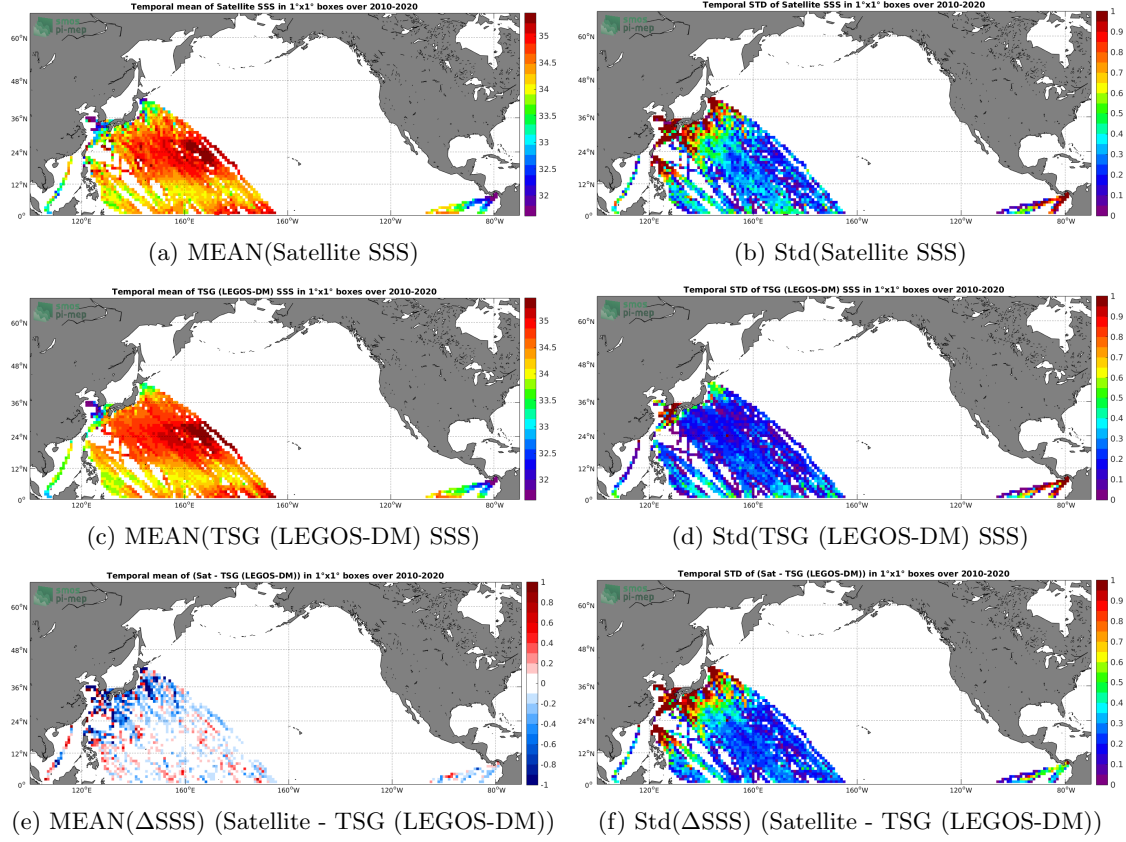
Figure 6: Temporal mean (left) and Std (right) of SSS from SMOS SSS L3 v317 - 10 Days - 25 km (CATDS-CPDC) (top), TSG (LEGOS-DM) (middle), and of \Delta SSS (Satellite - TSG (LEGOS-DM)). Only match-up pairs are used to generate these maps.
