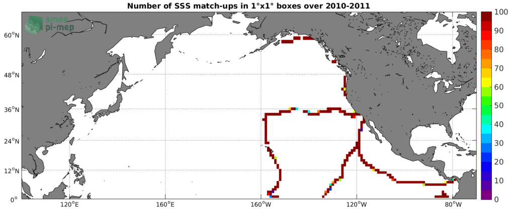
Figure 4: Number of SSS match-ups between TSG (GOSUD-Sailing-ship) SSS and the SMOS SSS L3 v317 - 10 Days - 25 km (CATDS-CPDC) SSS product for the North Pacific Ocean Pi-MEP region over 1^\circ \times 1^\circ boxes and for the full satellite product period.
