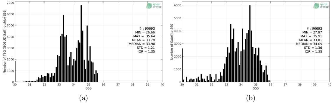
Figure 2: Histograms of SSS from TSG (GOSUD-Sailing-ship) (a) and SMOS SSS L3 v317 - 10 Days - 25 km (CATDS-CPDC) (b) considering all match-up pairs per bins of 0.1 over the North Pacific Ocean Pi-MEP region and for the full satellite product period.
