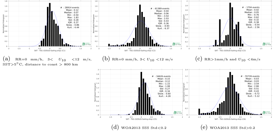
Figure 13: Normalized histogram of \Delta SSS (SMOS SSS L3 v317 - 10 Days - 25 km (CATDS-CPDC) - TSG (GOSUD-Sailing-ship)) for 5 different subdatasets corresponding to: RR=0 mm/h, 3 < U_{10} < 12 m/s, SST>5°C, distance to coast > 800 km (a), RR=0 mm/h, 3 < U_{10} < 12 m/s (b), RR>1mm/h and U_{10} < 4 m/s (c), WOA2013 SSS Std<0.2 (d), WOA2013 SSS Std>0.2 (e).
