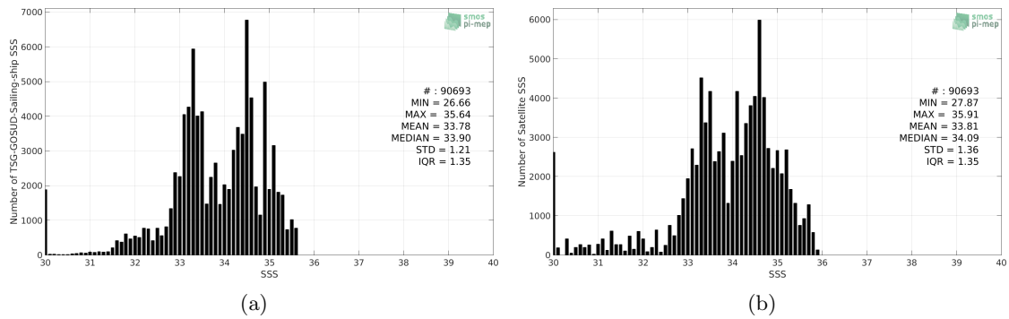
Figure 2: Histograms of SSS from TSG-GOSUD-Sailing-ship (a) and SMOS L3 v317 - 10 Days - 25 km (CATDS-CPDC) (b) considering all match-up pairs per bins of 0.1 over the North Pacific Ocean Pi-MEP region and for the full satellite product period.
