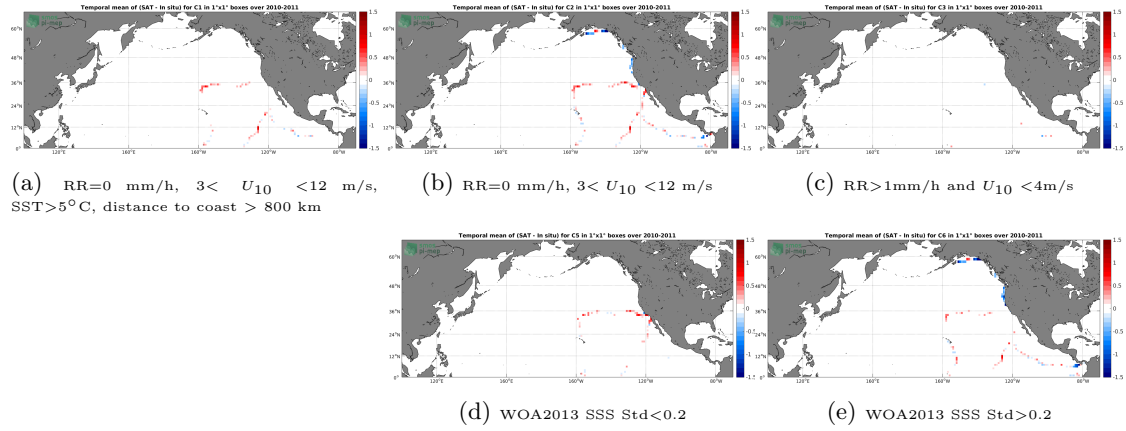
Figure 12: Temporal mean gridded over spatial boxes of size 1^\circ \times 1^\circ of \Delta SSS (SMOS L3 v317 - 10 Days - 25 km (CATDS-CPDC) - TSG-GOSUD-Sailing-ship) for 5 different subdatasets corresponding to: RR=0 mm/h, 3 < U_{10} < 12 m/s, SST >5^\circ\text{C} , distance to coast > 800 km (a), RR=0 mm/h, 3 < U_{10} < 12 m/s (b), RR >1 mm/h and U_{10} < 4 m/s (c), WOA2013 SSS Std <0.2 (d), WOA2013 SSS Std >0.2 (e).
