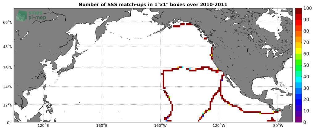
Figure 4: Number of SSS match-ups between TSG-GOSUD-Sailing-ship SSS and the SMOS L3 v317 - 10 Days - 25 km (CATDS-CPDC) SSS product for the North Pacific Ocean Pi-MEP region over 1^\circ \times 1^\circ boxes and for the full satellite product period.
