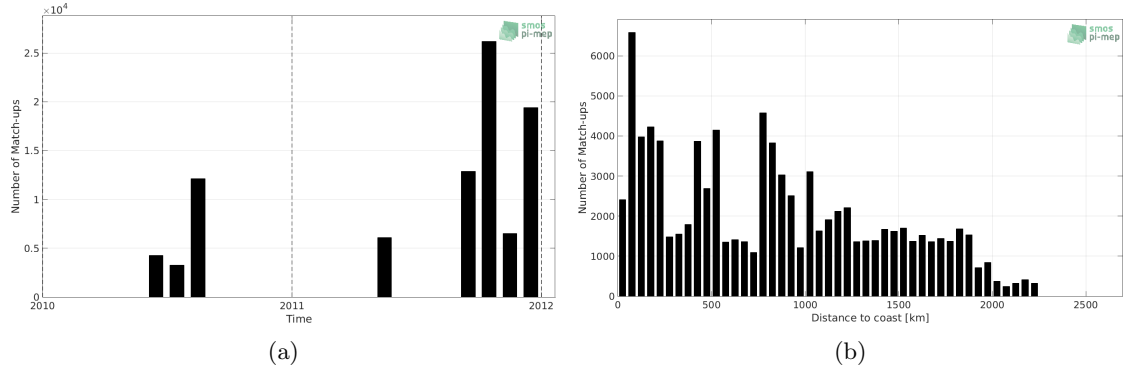
Figure 1: Number of match-ups between TSG-GOSUD-Sailing-ship and SMOS L3 v317 - 10 Days - 25 km (CATDS-CPDC) SSS as a function of time (a) and as function of the distance to coast (b) over the North Pacific Ocean Pi-MEP region and for the full satellite product period.
