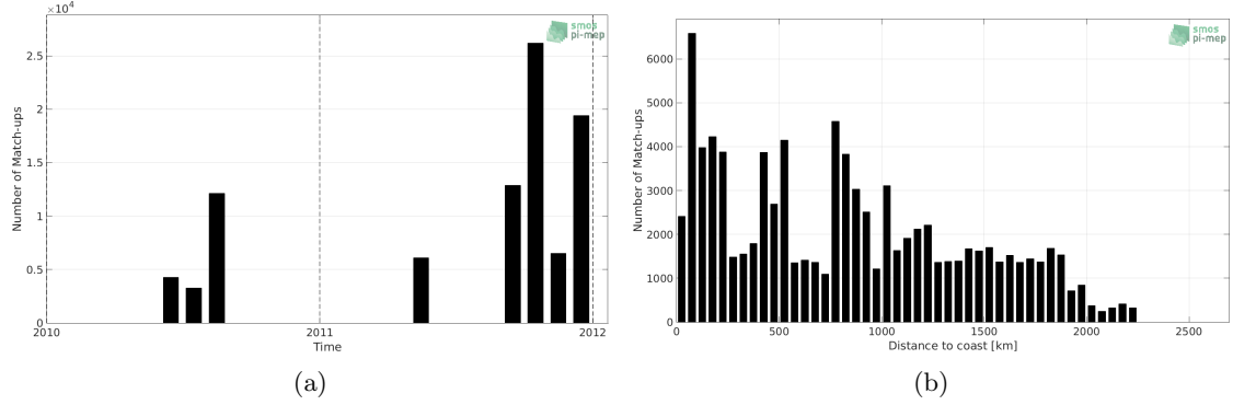
Figure 1: Number of match-ups between TSG-GOSUD-Sailing-ship and SMOS-L3-CATDS-CPDC-V317-10DAYS-25KM SSS as a function of time (a) and as function of the distance to coast (b) over the North Pacific Ocean Pi-MEP region and for the full satellite product period.
