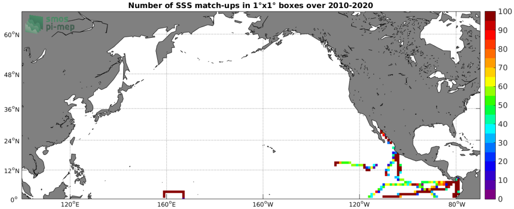
Figure 4: Number of SSS match-ups between TSG (GOSUD-Research-vessel) SSS and the SMOS SSS L3 v317 - 10 Days - 25 km (CATDS-CPDC) SSS product for the North Pacific Ocean Pi-MEP region over 1^\circ \times 1^\circ boxes and for the full satellite product period.
