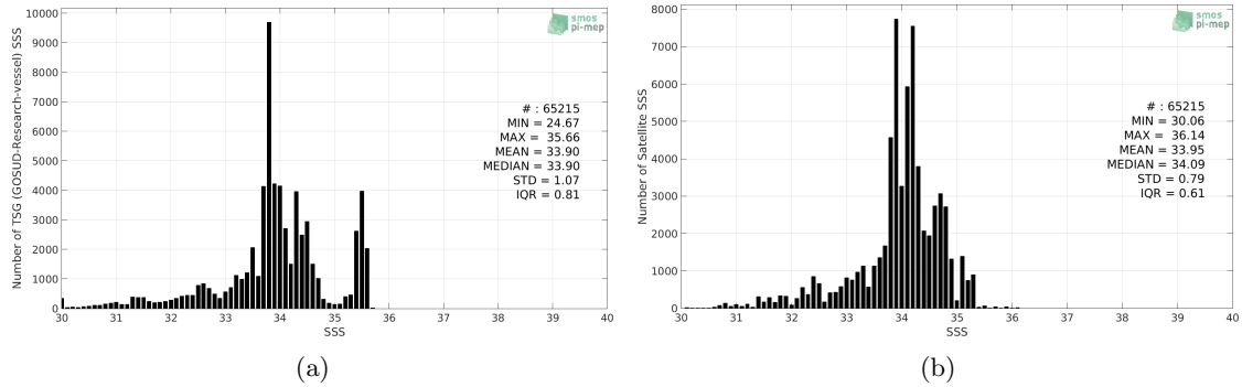
Figure 2: Histograms of SSS from TSG (GOSUD-Research-vessel) (a) and SMOS SSS L3 v317 - 10 Days - 25 km (CATDS-CPDC) (b) considering all match-up pairs per bins of 0.1 over the North Pacific Ocean Pi-MEP region and for the full satellite product period.
