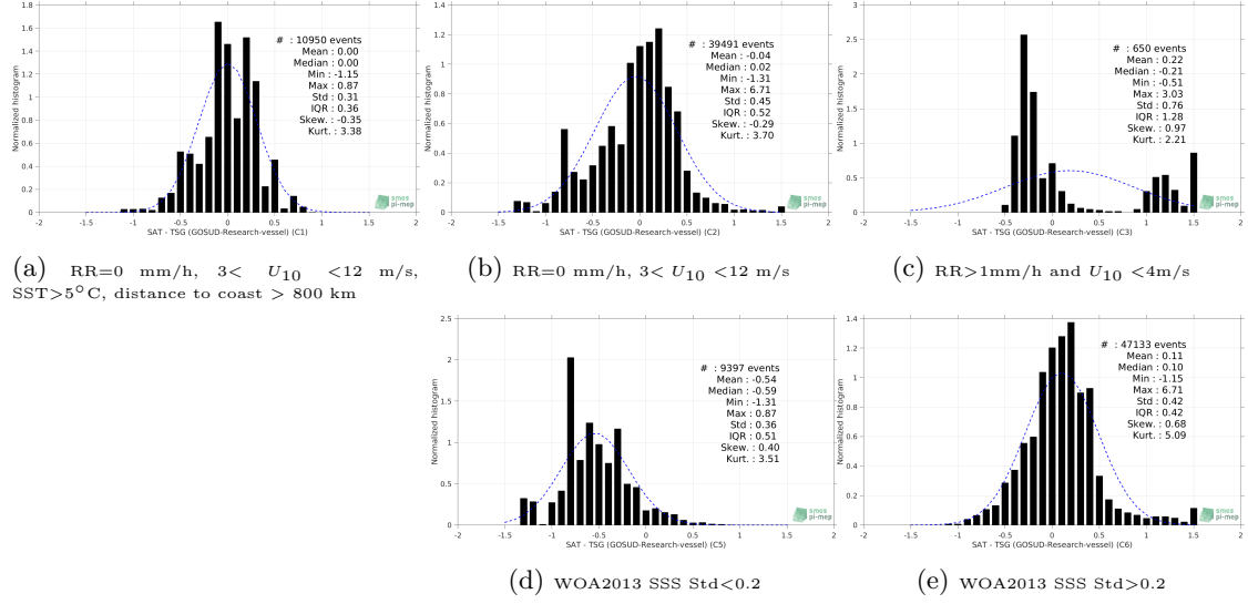
Figure 13: Normalized histogram of \Delta\text{SSS} (SMOS SSS L3 v317 - 10 Days - 25 km (CATDS-CPDC) - TSG (GOSUD-Research-vessel)) for 5 different subdatasets corresponding to: RR=0 mm/h, 3 < U_{10} < 12 m/s, SST > 5^\circ\text{C} , distance to coast > 800 km (a), RR=0 mm/h, 3 < U_{10} < 12 m/s (b), RR > 1\text{mm/h} and U_{10} < 4\text{m/s} (c), WOA2013 SSS Std < 0.2 (d), WOA2013 SSS Std > 0.2 (e).
