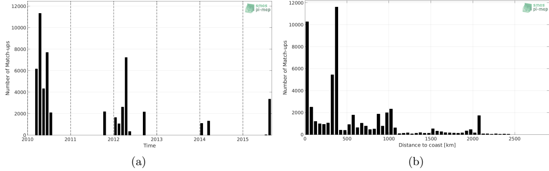
Figure 1: Number of match-ups between TSG-GOSUD-Research-vessel and SMOS L3 v317 - 10 Days - 25 km (CATDS-CPDC) SSS as a function of time (a) and as function of the distance to coast (b) over the North Pacific Ocean Pi-MEP region and for the full satellite product period.
