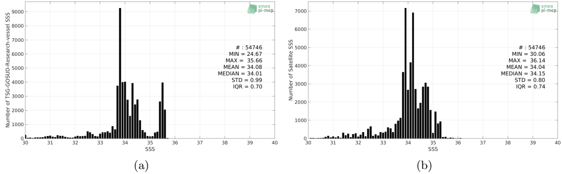
Figure 2: Histograms of SSS from TSG-GOSUD-Research-vessel (a) and SMOS L3 v317 - 10 Days - 25 km (CATDS-CPDC) (b) considering all match-up pairs per bins of 0.1 over the North Pacific Ocean Pi-MEP region and for the full satellite product period.
