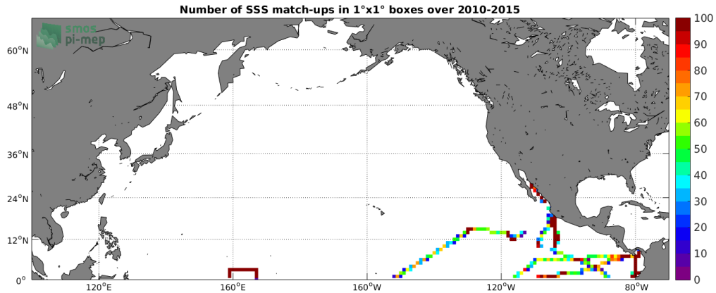
Figure 4: Number of SSS match-ups between TSG-GOSUD-Research-vessel SSS and the SMOS L3 v317 - 10 Days - 25 km (CATDS-CPDC) SSS product for the North Pacific Ocean Pi-MEP region over 1^\circ \times 1^\circ boxes and for the full satellite product period.
