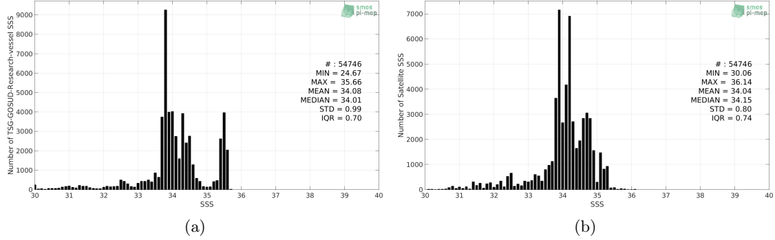
Figure 2: Histograms of SSS from TSG-GOSUD-Research-vessel (a) and SMOS-L3-CATDS-CPDC-V317-10DAYS-25KM (b) considering all match-up pairs per bins of 0.1 over the North Pacific Ocean Pi-MEP region and for the full satellite product period.
