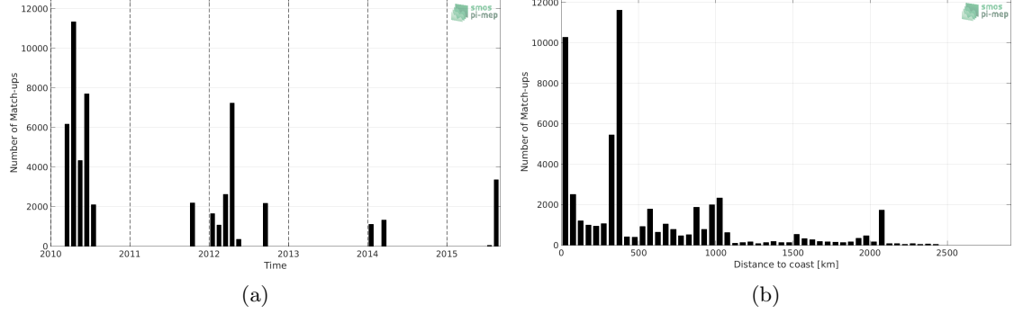
Figure 1: Number of match-ups between TSG-GOSUD-Research-vessel and SMOS-L3-CATDS-CPDC-V317-10DAYS-25KM SSS as a function of time (a) and as function of the distance to coast (b) over the North Pacific Ocean Pi-MEP region and for the full satellite product period.
