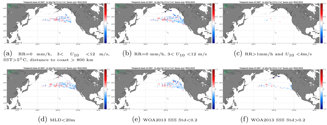
Figure 12: Temporal mean gridded over spatial boxes of size 1^\circ \times 1^\circ of \Delta SSS (SMOS SSS L3 v317 - 10 Days - 25 km (CATDS-CPDC) - Marine mammals) for 6 different subdatasets corresponding to:RR=0 mm/h, 3 < U_{10} < 12 m/s, SST >5^\circ\text{C} , distance to coast > 800 km (a), RR=0 mm/h, 3 < U_{10} < 12 m/s (b), RR >1 mm/h and U_{10} < 4 m/s (c),MLD <20 m (d),WOA2013 SSS Std <0.2 (e),WOA2013 SSS Std >0.2 (f).
