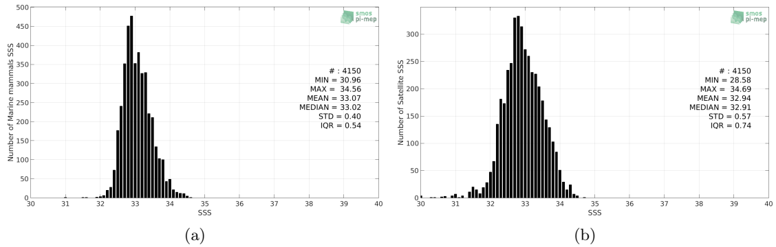
Figure 2: Histograms of SSS from Marine mammals (a) and SMOS SSS L3 v317 - 10 Days - 25 km (CATDS-CPDC) (b) considering all match-up pairs per bins of 0.1 over the North Pacific Ocean Pi-MEP region and for the full satellite product period.
