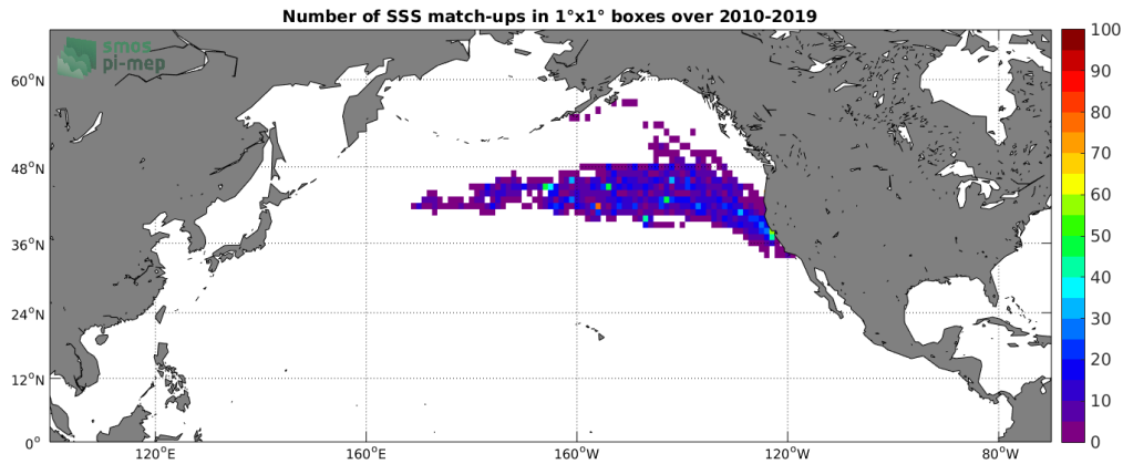
Figure 4: Number of SSS match-ups between Marine mammals SSS and the SMOS SSS L3 v317 - 10 Days - 25 km (CATDS-CPDC) SSS product for the North Pacific Ocean Pi-MEP region over 1^\circ \times 1^\circ boxes and for the full satellite product period.
