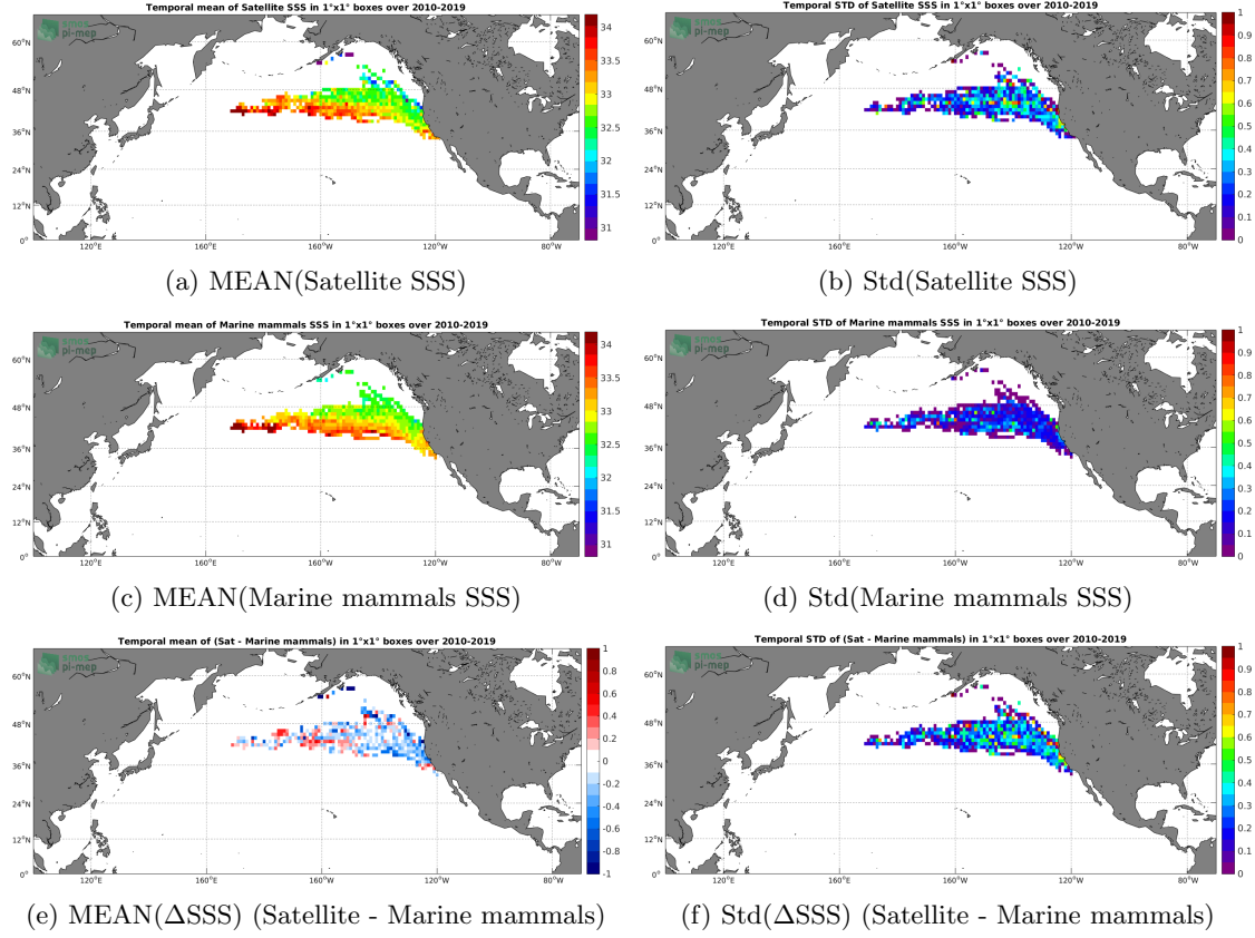
Figure 6: Temporal mean (left) and Std (right) of SSS from SMOS SSS L3 v317 - 10 Days - 25 km (CATDS-CPDC) (top), Marine mammals (middle), and of \Delta SSS (Satellite - Marine mammals). Only match-up pairs are used to generate these maps.
