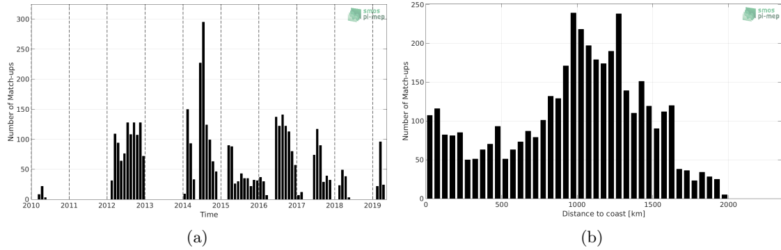
Figure 1: Number of match-ups between Marine mammals and SMOS SSS L3 v317 - 10 Days - 25 km (CATDS-CPDC) SSS as a function of time (a) and as function of the distance to coast (b) over the North Pacific Ocean Pi-MEP region and for the full satellite product period.
