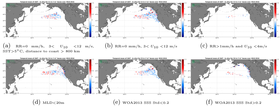
Figure 12: Temporal mean gridded over spatial boxes of size 1^\circ \times 1^\circ of \Delta SSS (SMOS SSS L3 v317 - 10 Days - 25 km (CATDS-CPDC) - Sea mammals) for 6 different subdatasets corresponding to: RR=0 mm/h, 3 < U_{10} < 12 m/s, SST > 5^\circ C , distance to coast > 800 km (a), RR=0 mm/h, 3 < U_{10} < 12 m/s (b), RR > 1 mm/h and U_{10} < 4 m/s (c), MLD < 20 m (d), WOA2013 SSS Std < 0.2 (e), WOA2013 SSS Std > 0.2 (f).
