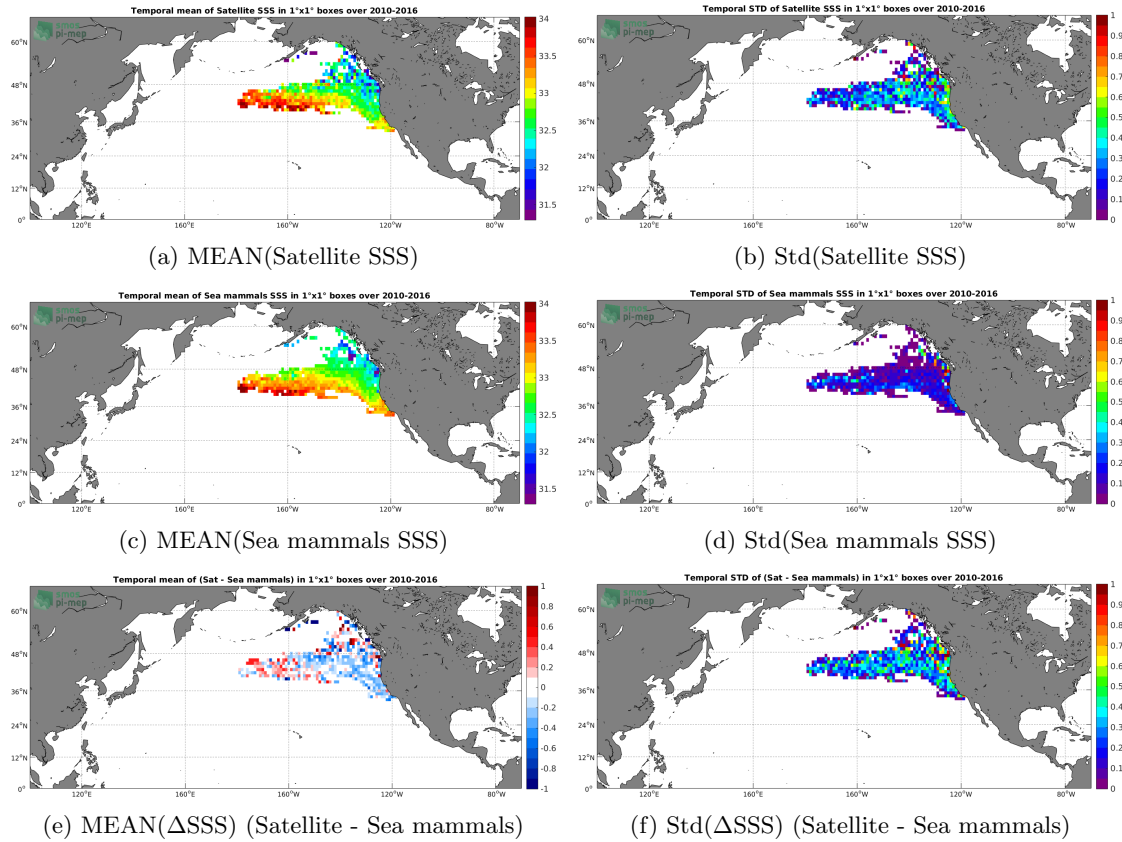
Figure 6: Temporal mean (left) and Std (right) of SSS from SMOS SSS L3 v317 - 10 Days - 25 km (CATDS-CPDC) (top), Sea mammals (middle), and of \Delta SSS (Satellite - Sea mammals). Only match-up pairs are used to generate these maps.
