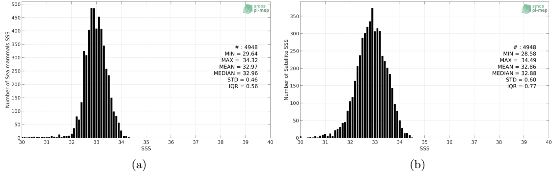
Figure 2: Histograms of SSS from Sea mammals (a) and SMOS SSS L3 v317 - 10 Days - 25 km (CATDS-CPDC) (b) considering all match-up pairs per bins of 0.1 over the North Pacific Ocean Pi-MEP region and for the full satellite product period.
