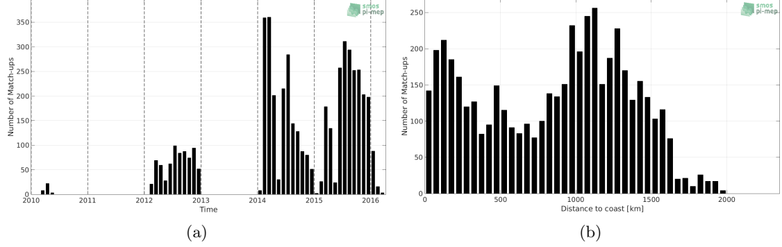
Figure 1: Number of match-ups between Sea mammals and SMOS SSS L3 v317 - 10 Days - 25 km (CATDS-CPDC) SSS as a function of time (a) and as function of the distance to coast (b) over the North Pacific Ocean Pi-MEP region and for the full satellite product period.
