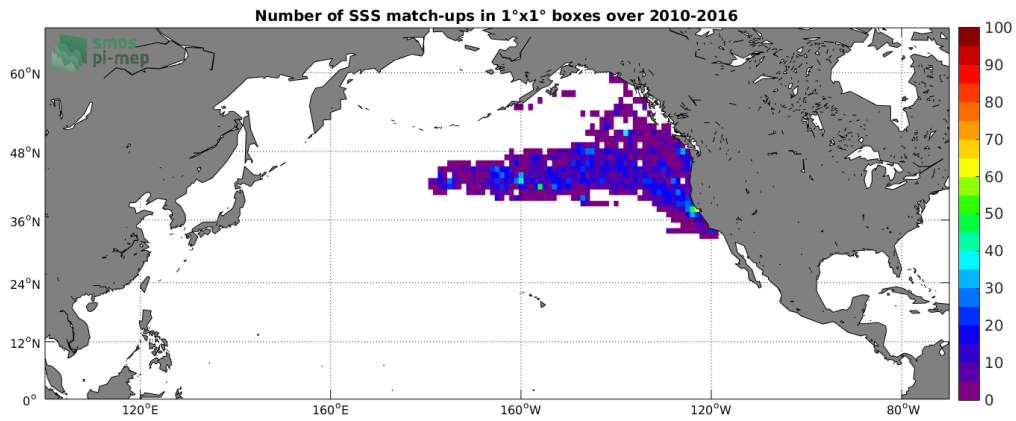
Figure 4: Number of SSS match-ups between Sea mammals SSS and the SMOS SSS L3 v317 - 10 Days - 25 km (CATDS-CPDC) SSS product for the North Pacific Ocean Pi-MEP region over 1^\circ \times 1^\circ boxes and for the full satellite product period.
