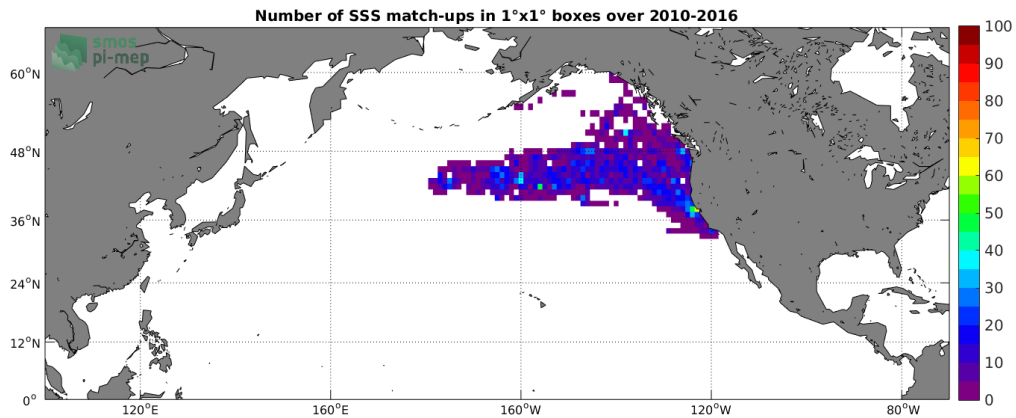
Figure 4: Number of SSS match-ups between Sea mammals SSS and the SMOS L3 v317 - 10 Days - 25 km (CATDS-CPDC) SSS product for the North Pacific Ocean Pi-MEP region over 1°x1° boxes and for the full satellite product period.
