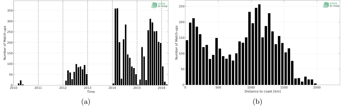
Figure 1: Number of match-ups between Sea mammals and SMOS L3 v317 - 10 Days - 25 km (CATDS-CPDC) SSS as a function of time (a) and as function of the distance to coast (b) over the North Pacific Ocean Pi-MEP region and for the full satellite product period.
