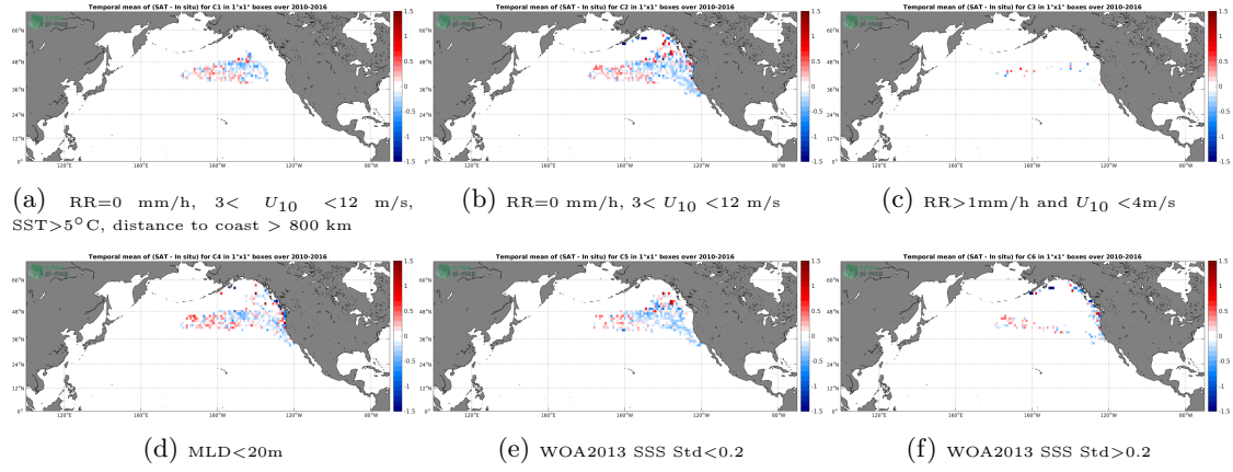
Figure 12: Temporal mean gridded over spatial boxes of size 1^\circ \times 1^\circ of \Delta SSS (SMOS L3 v317 - 10 Days - 25 km (CATDS-CPDC) - Sea mammals) for 6 different subdatasets corresponding to: RR=0 mm/h, 3 < U_{10} < 12 m/s, SST > 5^\circ\text{C} , distance to coast > 800 km (a), RR=0 mm/h, 3 < U_{10} < 12 m/s (b), RR > 1 mm/h and U_{10} < 4 m/s (c), MLD < 20 m (d), WOA2013 SSS Std < 0.2 (e), WOA2013 SSS Std > 0.2 (f).
