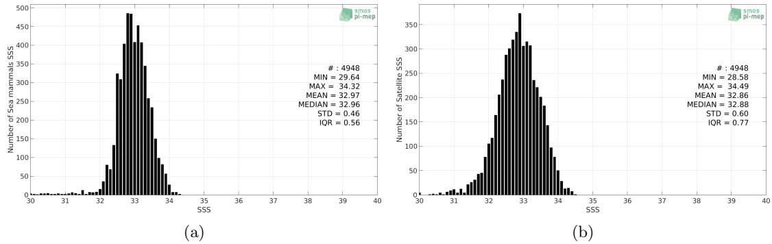
Figure 2: Histograms of SSS from Sea mammals (a) and SMOS L3 v317 - 10 Days - 25 km (CATDS-CPDC) (b) considering all match-up pairs per bins of 0.1 over the North Pacific Ocean Pi-MEP region and for the full satellite product period.
