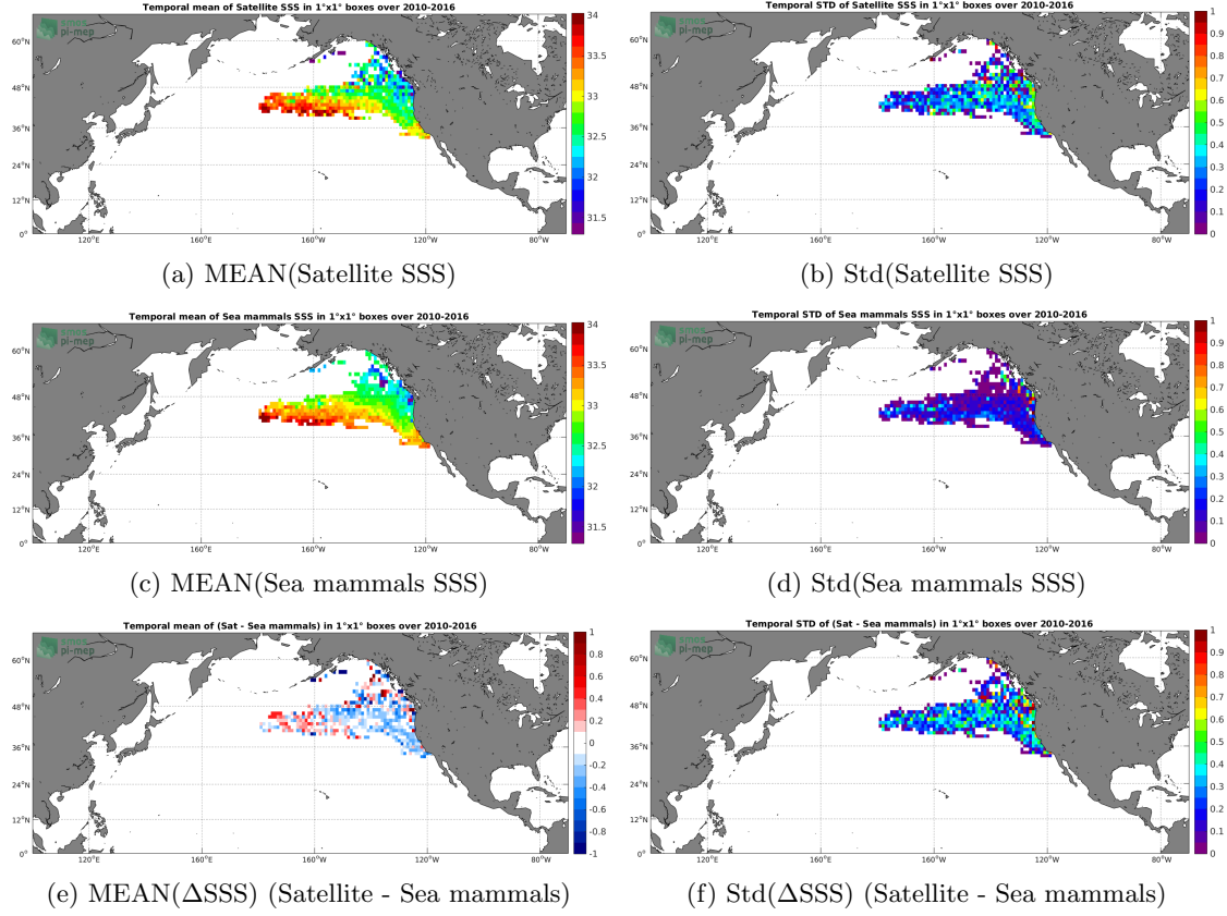
Figure 6: Temporal mean (left) and Std (right) of SSS from SMOS L3 v317 - 10 Days - 25 km (CATDS-CPDC) (top), Sea mammals (middle), and of \Delta SSS (Satellite - Sea mammals). Only match-up pairs are used to generate these maps.
