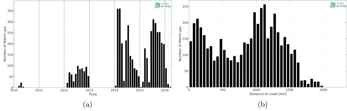
Figure 1: Number of match-ups between Sea mammals and SMOS-L3-CATDS-CPDC-V317-10DAYS-25KM SSS as a function of time (a) and as function of the distance to coast (b) over the North Pacific Ocean Pi-MEP region and for the full satellite product period.
