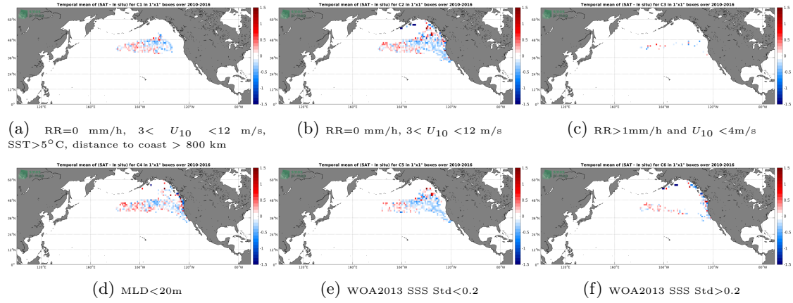
Figure 12: Temporal mean gridded over spatial boxes of size 1^\circ \times 1^\circ of \Delta SSS (SMOS-L3-CATDS-CPDC-V317-10DAYS-25KM - Sea mammals) for 6 different subdatasets corresponding to: RR=0 mm/h, 3 < U_{10} < 12 m/s, SST > 5^\circ\text{C} , distance to coast > 800 km (a), RR=0 mm/h, 3 < U_{10} < 12 m/s (b), RR > 1 mm/h and U_{10} < 4 m/s (c), MLD < 20 m (d), WOA2013 SSS Std < 0.2 (e), WOA2013 SSS Std > 0.2 (f).
