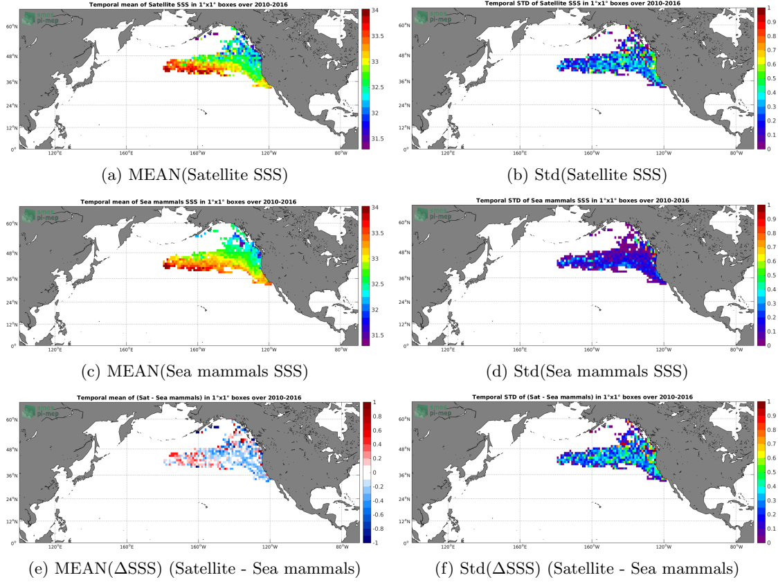
Figure 6: Temporal mean (left) and Std (right) of SSS from SMOS-L3-CATDS-CPDC-V317-10DAYS-25KM (top), Sea mammals (middle), and of \Delta SSS (Satellite - Sea mammals). Only match-up pairs are used to generate these maps.
