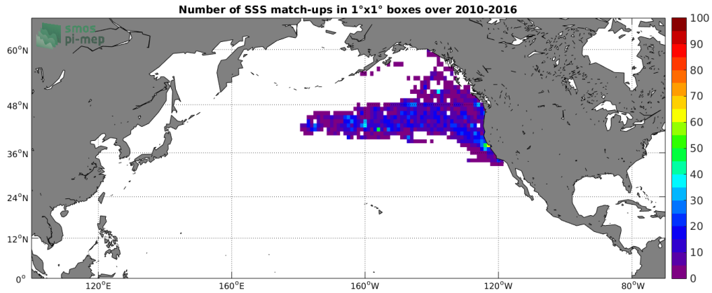
Figure 4: Number of SSS match-ups between Sea mammals SSS and the SMOS-L3-CATDS-CPDC-V317-10DAYS-25KM SSS product for the North Pacific Ocean Pi-MEP region over 1°x1° boxes and for the full satellite product period.
