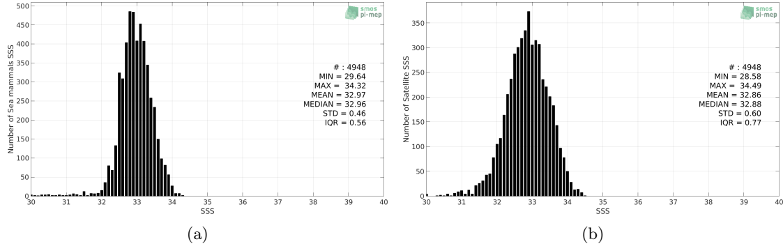
Figure 2: Histograms of SSS from Sea mammals (a) and SMOS-L3-CATDS-CPDC-V317-10DAYS-25KM (b) considering all match-up pairs per bins of 0.1 over the North Pacific Ocean Pi-MEP region and for the full satellite product period.
