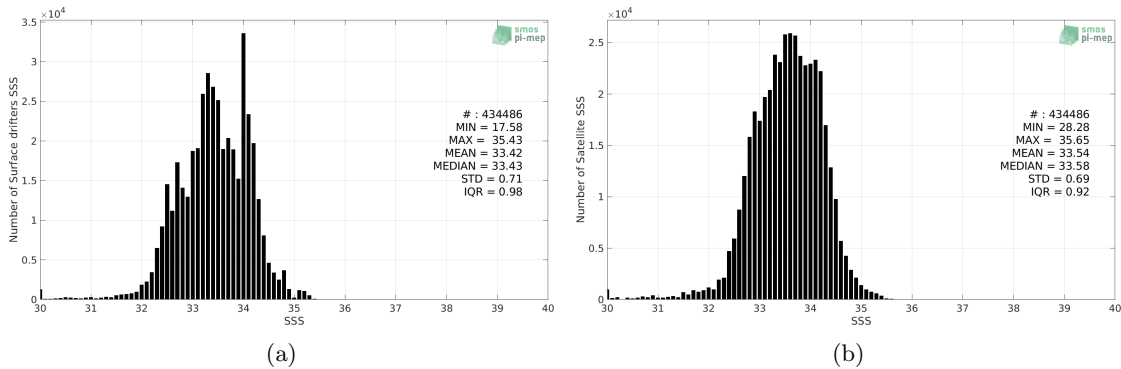
Figure 2: Histograms of SSS from Surface drifters (a) and SMOS SSS L3 v317 - 10 Days - 25 km (CATDS-CPDC) (b) considering all match-up pairs per bins of 0.1 over the North Pacific Ocean Pi-MEP region and for the full satellite product period.
