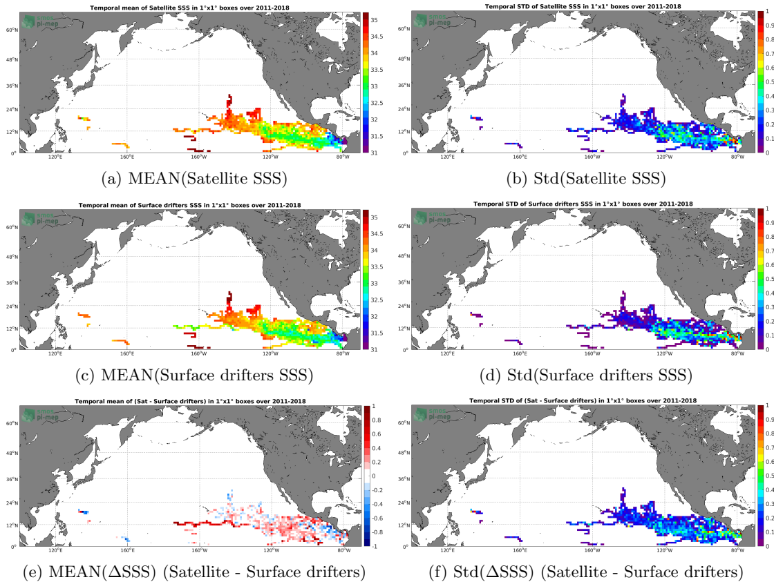
Figure 5: Temporal mean (left) and Std (right) of SSS from SMOS SSS L3 v317 - 10 Days - 25 km (CATDS-CPDC) (top), Surface drifters (middle), and of \Delta SSS (Satellite - Surface drifters). Only match-up pairs are used to generate these maps.
