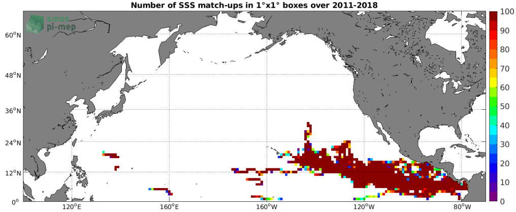
Figure 3: Number of SSS match-ups between Surface drifters SSS and the SMOS SSS L3 v317 - 10 Days - 25 km (CATDS-CPDC) SSS product for the North Pacific Ocean Pi-MEP region over 1^\circ \times 1^\circ boxes and for the full satellite product period.
