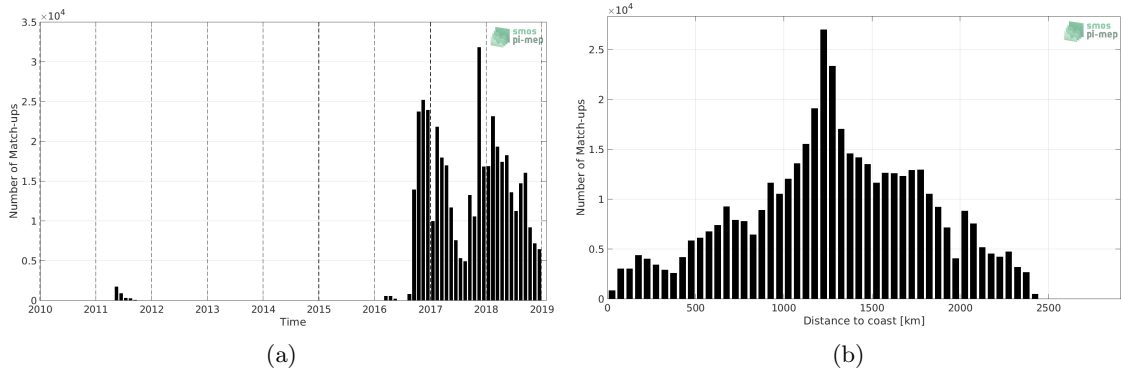
Figure 1: Number of match-ups between Surface drifters and SMOS SSS L3 v317 - 10 Days - 25 km (CATDS-CPDC) SSS as a function of time (a) and as function of the distance to coast (b) over the North Pacific Ocean Pi-MEP region and for the full satellite product period.
