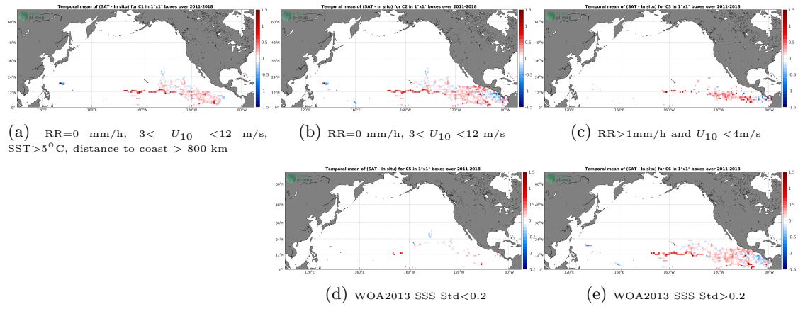
Figure 11: Temporal mean gridded over spatial boxes of size 1^\circ \times 1^\circ of \Delta SSS (SMOS SSS L3 v317 - 10 Days - 25 km (CATDS-CPDC) - Surface drifters) for 5 different subdatasets corresponding to: RR=0 mm/h, 3 < U_{10} < 12 m/s, SST >5^\circ\text{C} , distance to coast > 800 km (a), RR=0 mm/h, 3 < U_{10} < 12 m/s (b), RR >1 mm/h and U_{10} < 4 m/s (c), WOA2013 SSS Std <0.2 (d), WOA2013 SSS Std >0.2 (e).
