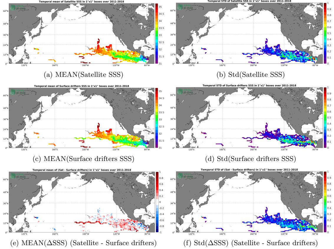
Figure 5: Temporal mean (left) and Std (right) of SSS from SMOS SSS L3 v317 - 10 Days - 25 km (CATDS-CPDC) (top), Surface drifters (middle), and of \Delta\text{SSS} (Satellite - Surface drifters). Only match-up pairs are used to generate these maps.
