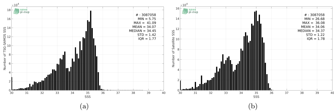
Figure 2: Histograms of SSS from TSG-SAMOS (a) and SMOS-L3-CATDS-CPDC-V3-MONTHLY-25KM (b) considering all match-up pairs per bins of 0.1 over the North Pacific Ocean Pi-MEP region and for the full satellite product period.
