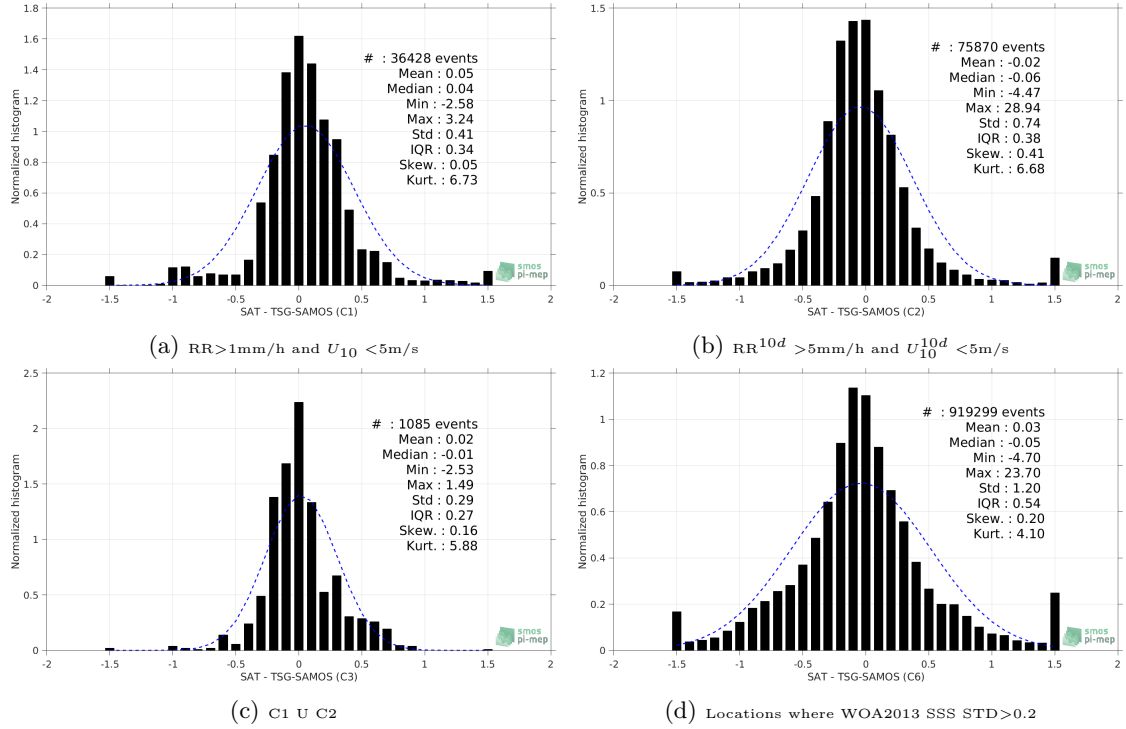
Figure 13: Normalized histogram of \Delta\text{SSS} (SMOS-L3-CATDS-CPDC-V3-MONTHLY-25KM - TSG-SAMOS) for 6 different subdatasets corresponding to: RR > 1\text{mm/h} and U_{10} < 5\text{m/s} (a), RR^{10d} > 5\text{mm/h} and U_{10}^{10d} < 5\text{m/s} (b), C1 U C2 (c), Locations where WOA2013 SSS STD > 0.2 (d).
