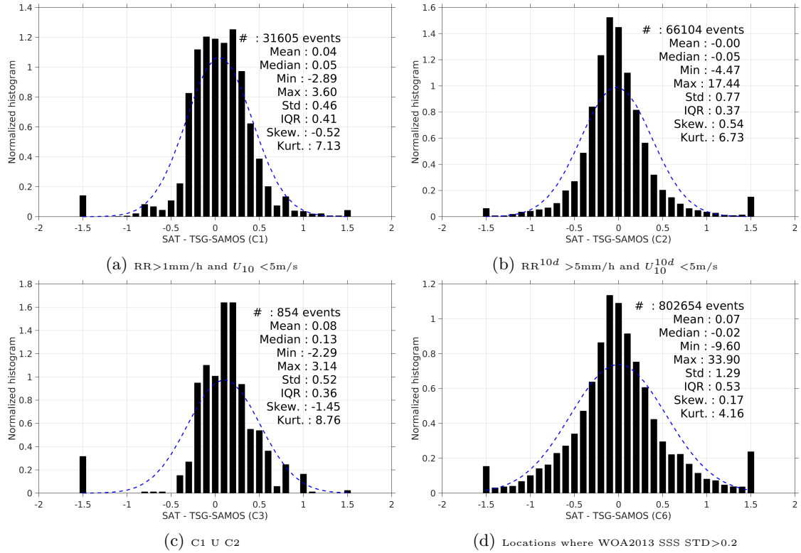
Figure 13: Normalized histogram of \Delta\text{SSS} (SMOS-L3-CATDS-CPDC-V3-MONTHLY-25KM - TSG-SAMOS) for 6 different subdatasets corresponding to: RR > 1\text{mm/h} and U_{10} < 5\text{m/s} (a), RR^{10d} > 5\text{mm/h} and U_{10}^{10d} < 5\text{m/s} (b), C1 U C2 (c), Locations where WOA2013 SSS STD > 0.2 (d).
