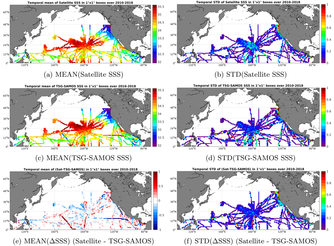
Figure 6: Temporal mean (left) and STD (right) of SSS from SMOS-L3-CATDS-CPDC-V3-MONTHLY-25KM (top), TSG-SAMOS (middle), and of \Delta SSS (Satellite - TSG-SAMOS). Only match-up pairs are used to generate these maps.
