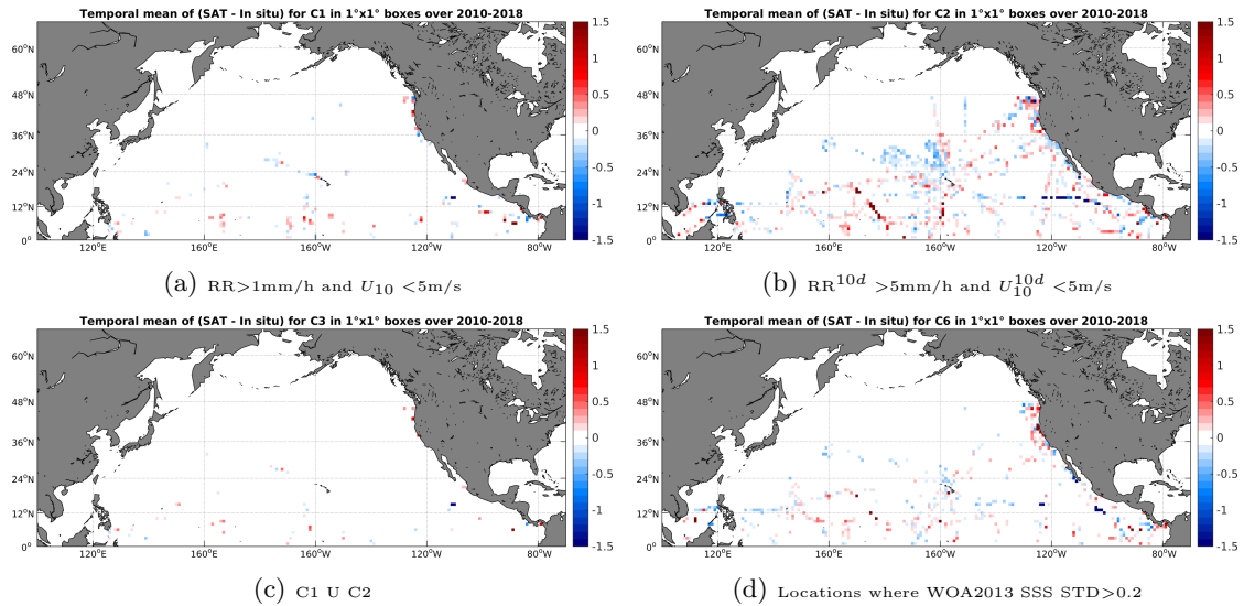
Figure 12: Temporal mean gridded over spatial boxes of size 1^\circ \times 1^\circ of \Delta SSS (SMOS-L3-CATDS-CPDC-V3-MONTHLY-25KM - TSG-SAMOS) for 4 different subdatasets corresponding to: RR > 1\text{mm/h} and U_{10} < 5\text{m/s} (a), RR^{10d} > 5\text{mm/h} and U_{10}^{10d} < 5\text{m/s} (b), C1 U C2 (c), Locations where WOA2013 SSS STD > 0.2 (d).
