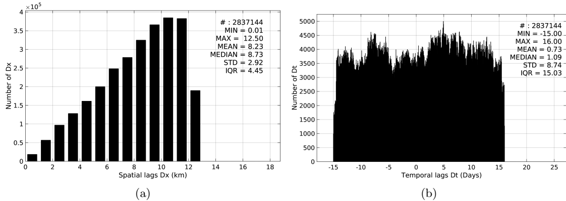
Figure 5: Histograms of the spatial (a) and temporal (b) lags between the time of the TSG-SAMOS measurements and the date of the corresponding SMOS-L3-CATDS-CPDC-V3-MONTHLY-25KM SSS product.
