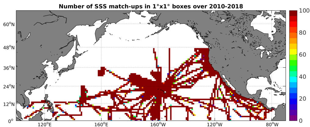
Figure 4: Number of SSS match-ups between TSG-SAMOS SSS and the SMOS-L3-CATDS-CPDC-V3-MONTHLY-25KM SSS product for the North Pacific Ocean Pi-MEP region over 1^\circ \times 1^\circ boxes and for the full satellite product period.
