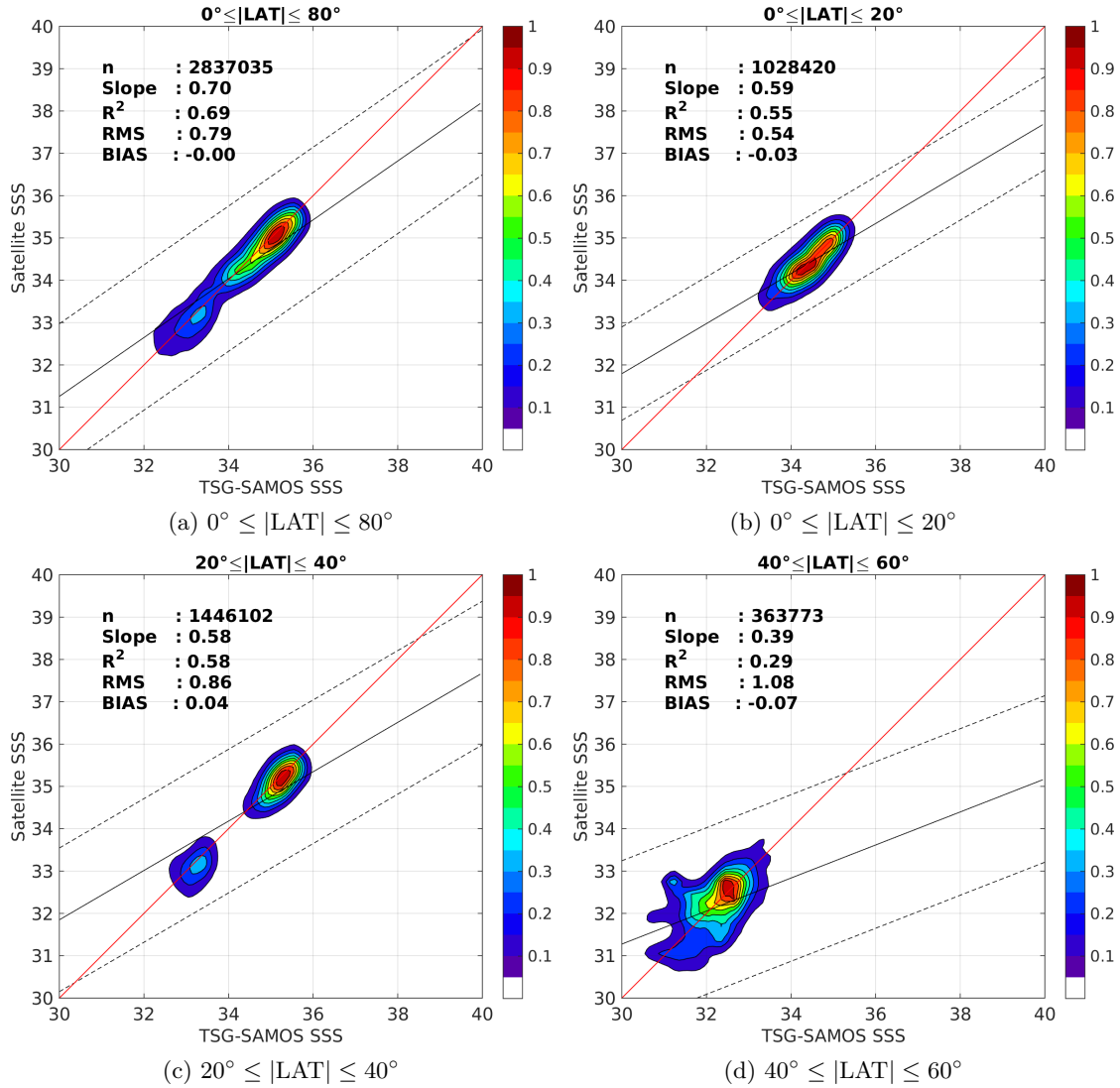
Figure 9: Contour maps of the concentration of SMOS-L3-CATDS-CPDC-V3-MONTHLY-25KM SSS (y-axis) versus TSG-SAMOS SSS (x-axis) at match-up pairs for different latitude bands. For each plot, the red line shows x=y . The black thin and dashed lines indicate a linear fit through the data cloud and the \pm 95\% confidence levels, respectively. The number match-up pairs n , the slope and R^2 coefficient of the linear fit, the root mean square (RMS) and the mean bias between satellite and in situ data are indicated for each latitude band in each plots.
