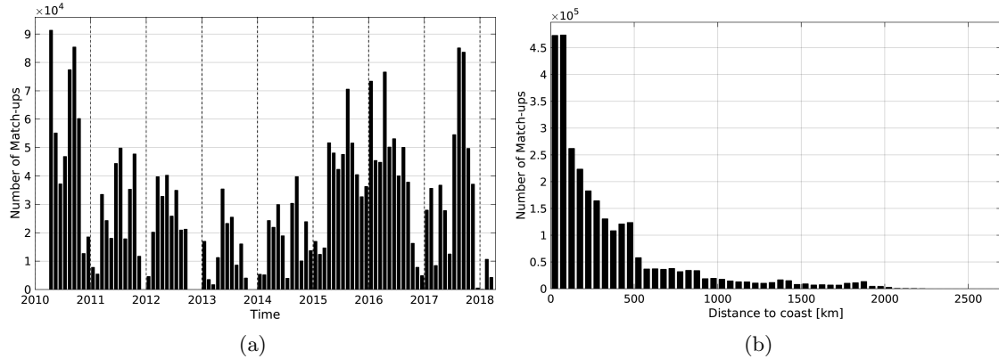
Figure 1: Number of match-ups between TSG-SAMOS and SMOS-L3-CATDS-CPDC-V3-MONTHLY-25KM SSS as a function of time (a) and as function of the distance to coast (b) over the North Pacific Ocean Pi-MEP region and for the full satellite product period.
