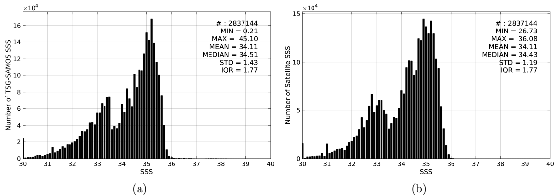
Figure 2: Histograms of SSS from TSG-SAMOS (a) and SMOS-L3-CATDS-CPDC-V3-MONTHLY-25KM (b) considering all match-up pairs per bins of 0.1 over the North Pacific Ocean Pi-MEP region and for the full satellite product period.
