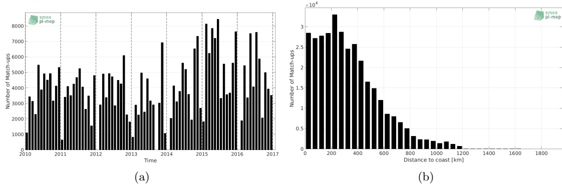
Figure 1: Number of match-ups between TSG-LEGOS-DM and SMOS-L3-CATDS-CPDC-V3-MONTHLY-25KM SSS as a function of time (a) and as function of the distance to coast (b) over the North Pacific Ocean Pi-MEP region and for the full satellite product period.
