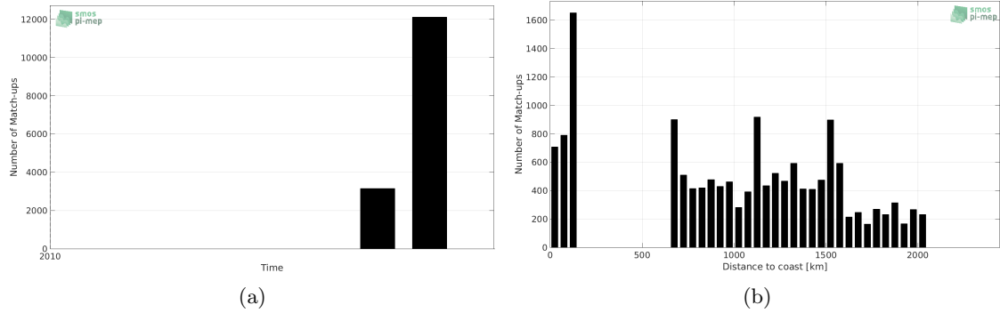
Figure 1: Number of match-ups between TSG-GOSUD-Sailing-ship and SMOS-L3-CATDS-CPDC-V3-MONTHLY-25KM SSS as a function of time (a) and as function of the distance to coast (b) over the North Pacific Ocean Pi-MEP region and for the full satellite product period.
