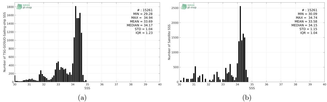
Figure 2: Histograms of SSS from TSG-GOSUD-Sailing-ship (a) and SMOS-L3-CATDS-CPDC-V3-MONTHLY-25KM (b) considering all match-up pairs per bins of 0.1 over the North Pacific Ocean Pi-MEP region and for the full satellite product period.
