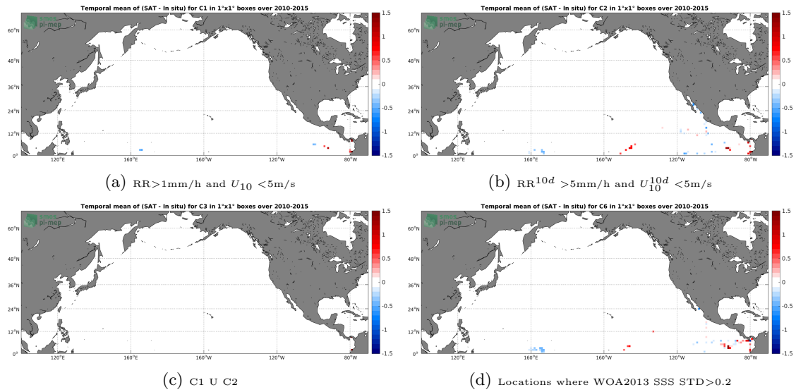
Figure 12: Temporal mean gridded over spatial boxes of size 1^\circ \times 1^\circ of \Delta SSS (SMOS-L3-CATDS-CPDC-V3-MONTHLY-25KM - TSG-GOSUD-Research-vessel) for 4 different subdatasets corresponding to: RR > 1\text{mm/h} and U_{10} < 5\text{m/s} (a), RR^{10d} > 5\text{mm/h} and U_{10}^{10d} < 5\text{m/s} (b), C1 U C2 (c), Locations where WOA2013 SSS STD > 0.2 (d).
