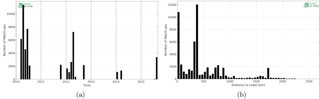
Figure 1: Number of match-ups between TSG-GOSUD-Research-vessel and SMOS-L3-CATDS-CPDC-V3-MONTHLY-25KM SSS as a function of time (a) and as function of the distance to coast (b) over the North Pacific Ocean Pi-MEP region and for the full satellite product period.
