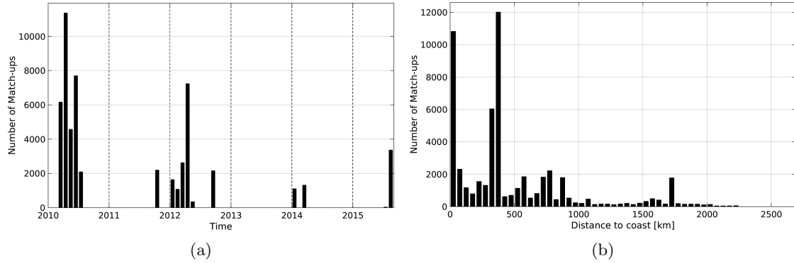
Figure 1: Number of match-ups between TSG-GOSUD-Research-vessel and SMOS-L3-CATDS-CPDC-V3-MONTHLY-25KM SSS as a function of time (a) and as function of the distance to coast (b) over the North Pacific Ocean Pi-MEP region and for the full satellite product period.
