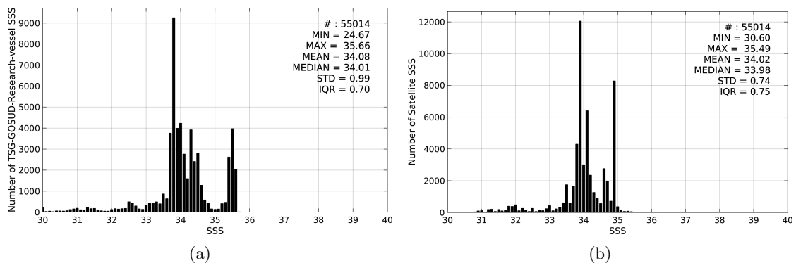
Figure 2: Histograms of SSS from TSG-GOSUD-Research-vessel (a) and SMOS-L3-CATDS-CPDC-V3-MONTHLY-25KM (b) considering all match-up pairs per bins of 0.1 over the North Pacific Ocean Pi-MEP region and for the full satellite product period.
