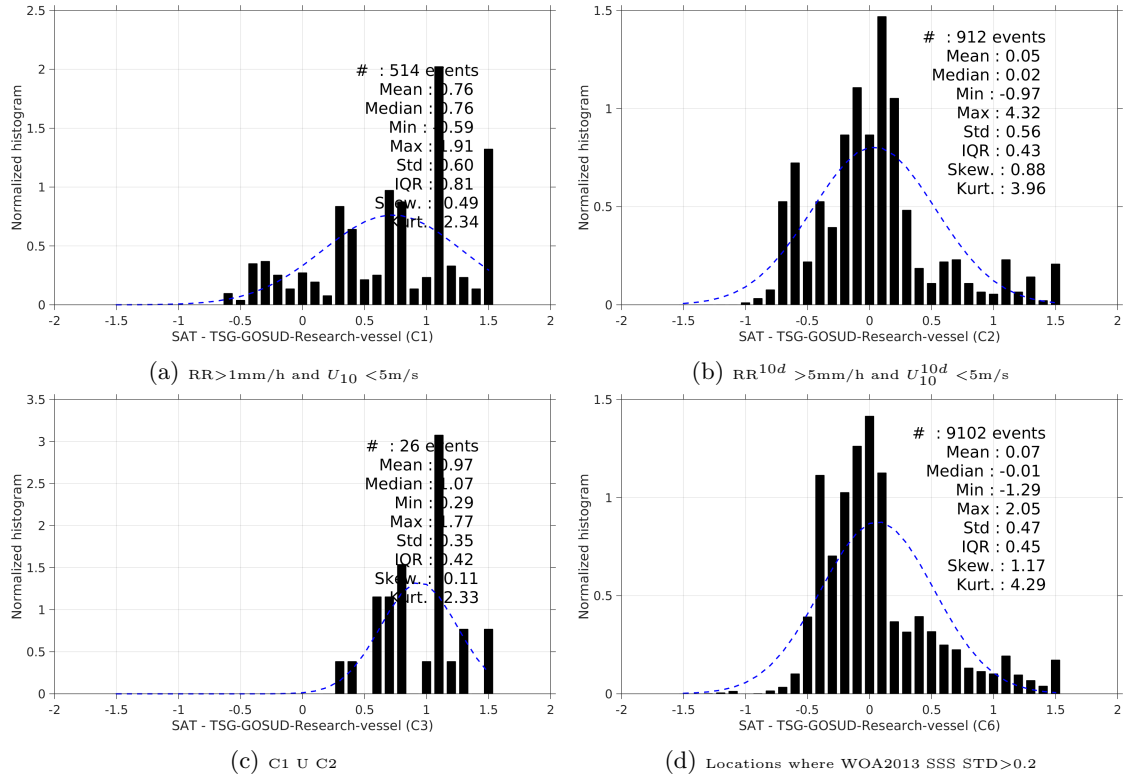
Figure 13: Normalized histogram of \Delta SSS (SMOS-L3-CATDS-CPDC-V3-MONTHLY-25KM - TSG-GOSUD-Research-vessel) for 6 different subdatasets corresponding to: RR > 1\text{mm/h} and U_{10} < 5\text{m/s} (a), RR^{10d} > 5\text{mm/h} and U_{10}^{10d} < 5\text{m/s} (b), C1 U C2 (c), Locations where WOA2013 SSS STD > 0.2 (d).
