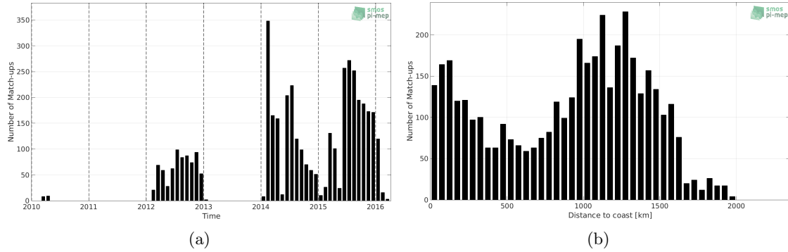
Figure 1: Number of match-ups between Sea mammals and SMOS-L3-CATDS-CPDC-V3-MONTHLY-25KM SSS as a function of time (a) and as function of the distance to coast (b) over the North Pacific Ocean Pi-MEP region and for the full satellite product period.
