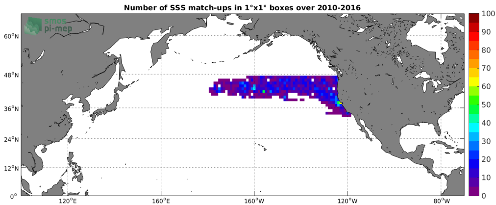
Figure 4: Number of SSS match-ups between Sea mammals SSS and the SMOS-L3-CATDS-CPDC-V3-MONTHLY-25KM SSS product for the North Pacific Ocean Pi-MEP region over 1°x1° boxes and for the full satellite product period.
