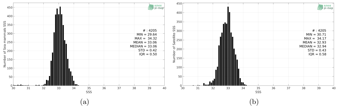
Figure 2: Histograms of SSS from Sea mammals (a) and SMOS-L3-CATDS-CPDC-V3-MONTHLY-25KM (b) considering all match-up pairs per bins of 0.1 over the North Pacific Ocean Pi-MEP region and for the full satellite product period.
