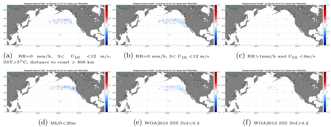
Figure 12: Temporal mean gridded over spatial boxes of size 1^\circ \times 1^\circ of \Delta SSS (SMOS-L3-CATDS-CPDC-V3-MONTHLY-25KM - Sea mammals) for 6 different subdatasets corresponding to:RR=0 mm/h, 3 < U_{10} < 12 m/s, SST >5^\circ C, distance to coast > 800 km (a), RR=0 mm/h, 3 < U_{10} < 12 m/s (b), RR >1 mm/h and U_{10} < 4 m/s (c),MLD <20 m (d),WOA2013 SSS Std <0.2 (e),WOA2013 SSS Std >0.2 (f).
