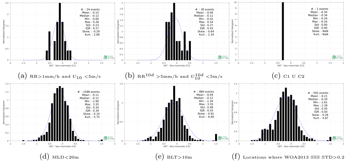
Figure 13: Normalized histogram of \Delta SSS (SMOS-L3-CATDS-CPDC-V3-MONTHLY-25KM - Sea mammals) for 6 different subdatasets corresponding to: RR>1mm/h and U_{10} < 5 m/s (a), RR^{10d} > 5 mm/h and U_{10}^{10d} < 5 m/s (b), C1 U C2 (c),MLD<20m (d),BLT>10m (e),Locations where WOA2013 SSS STD>0.2 (f).
