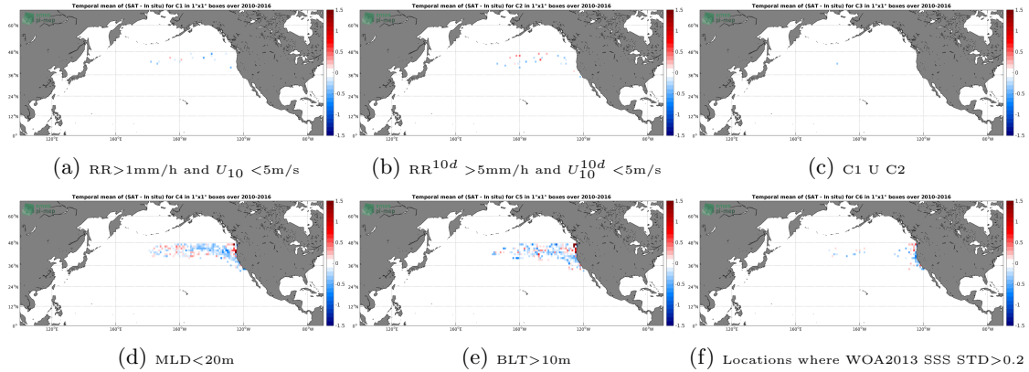
Figure 12: Temporal mean gridded over spatial boxes of size 1°x1° of \Delta SSS (SMOS-L3-CATDS-CPDC-V3-MONTHLY-25KM - Sea mammals) for 6 different subdatasets corresponding to:RR>1mm/h and U_{10} < 5 m/s (a), RR^{10d} > 5 mm/h and U_{10}^{10d} < 5 m/s (b), C1 U C2 (c),MLD<20m (d),BLT>10m (e),Locations where WOA2013 SSS STD>0.2 (f).
